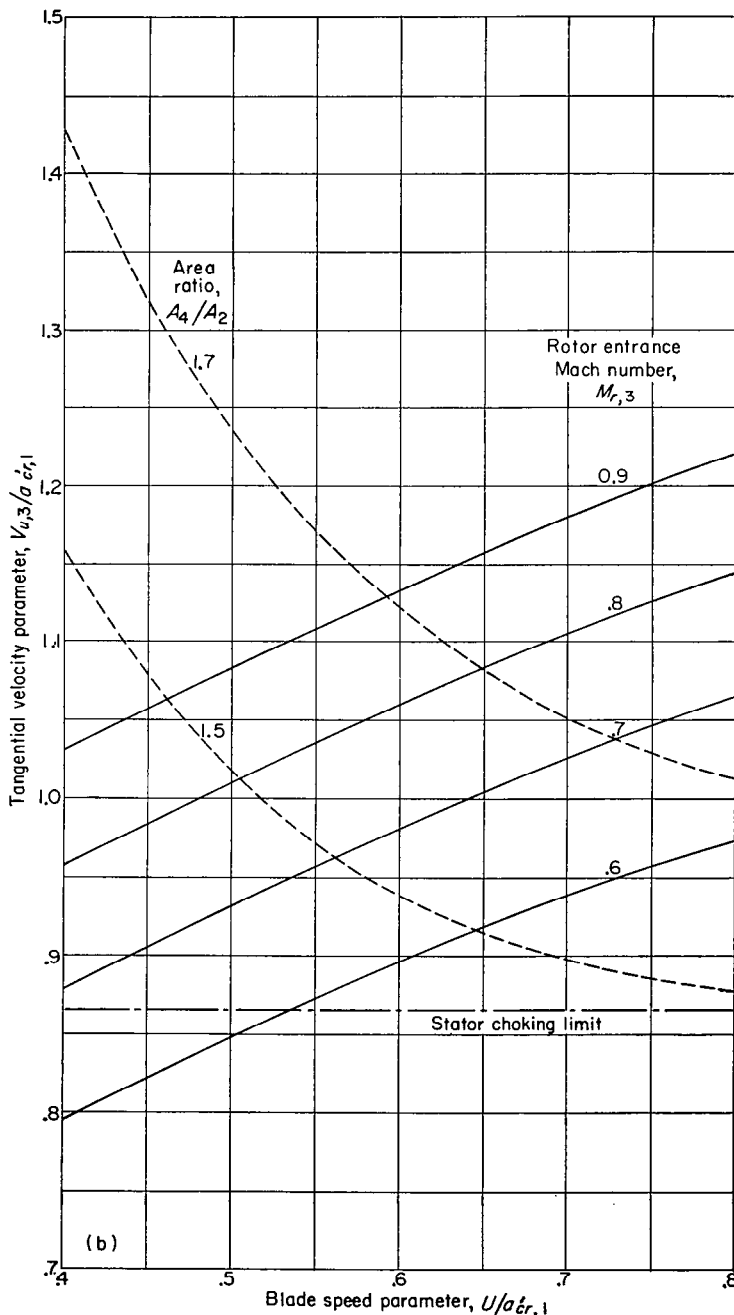
(b) Stator exit flow angle, 30°.
