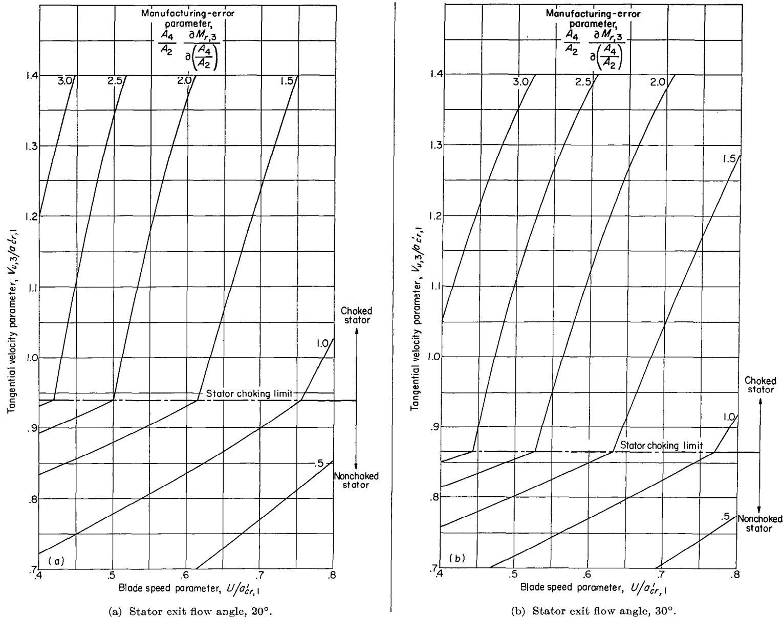
FIGURE 11.—Effect of manufacturing errors in throat areas on rotor entrance Mach number for stator followed by choked rotor. Equation (22) applies above stator choking limit and equation (53) applies below stator choking limit.
