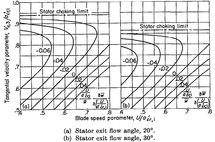
FIGURE 13.—Rate of variation of specific-mass-flow parameter with blade speed parameter for nonchoked stator followed by choked rotor (eq. (55)).
