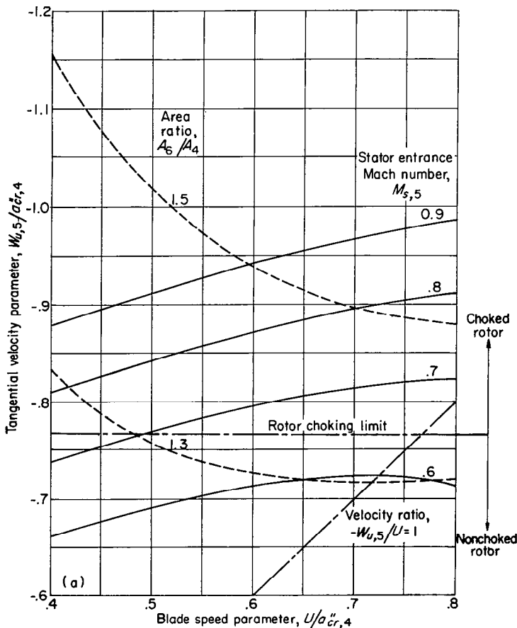
(a) Rotor exit flow angle, 140°.
