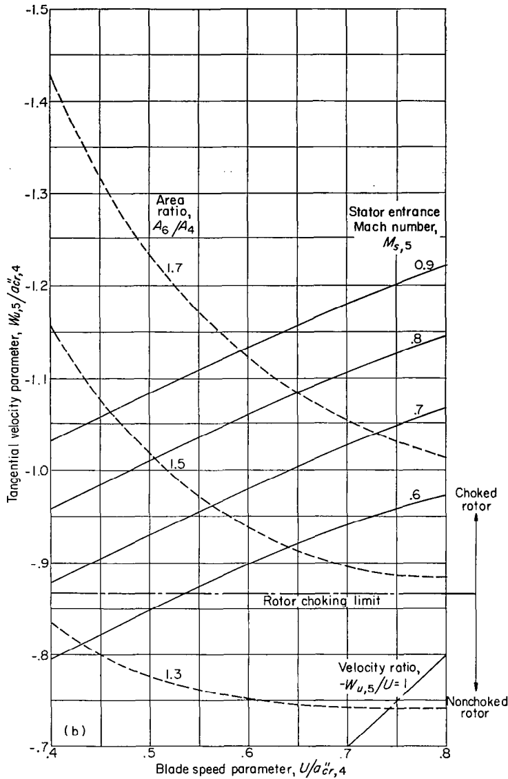
(b) Rotor exit flow angle, 150^\circ .
