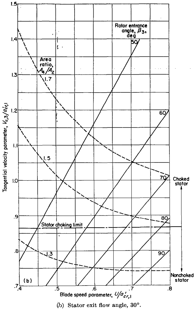
FIGURE 7.—Concluded. Relation among area ratio, rotor entrance angle, and velocity parameters at exit of choked stator followed by choked rotor (eq. (29)). For lines of constant area ratio, equation (17) applies above stator choking limit and equation (50) applies below stator choking limit.
