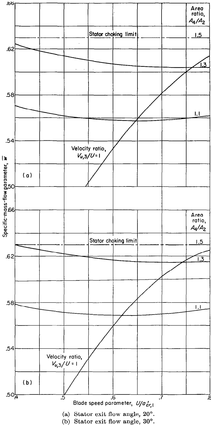
FIGURE 12.—Variation of specific-mass-flow parameter with blade speed parameter and area ratio for nonchoked stator followed by choked rotor (eqs. (50) and (54)).
