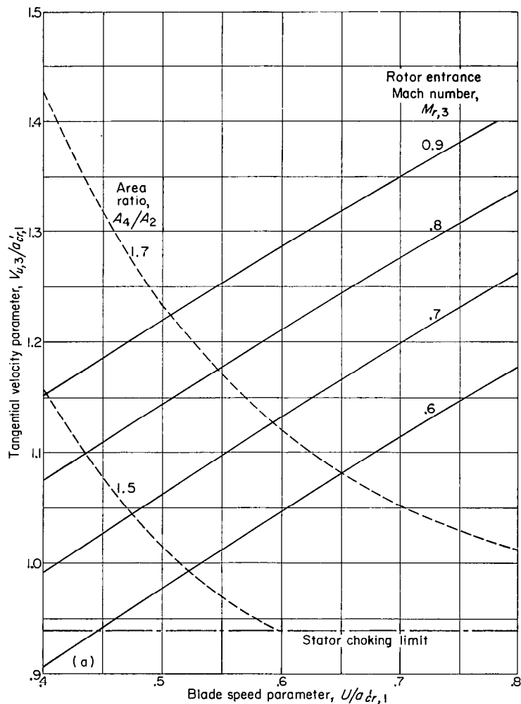
(a) Stator exit flow angle, 20°.
