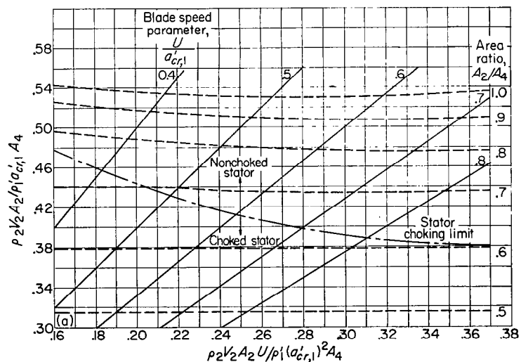
(a) Critical stator exit flow angle, 15°.
