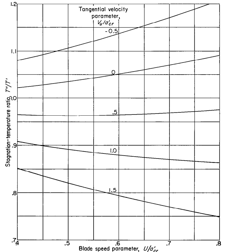
FIGURE 2.—Variation of stagnation-temperature ratio with blade speed parameter for various tangential velocity parameters (eq. (12)).
