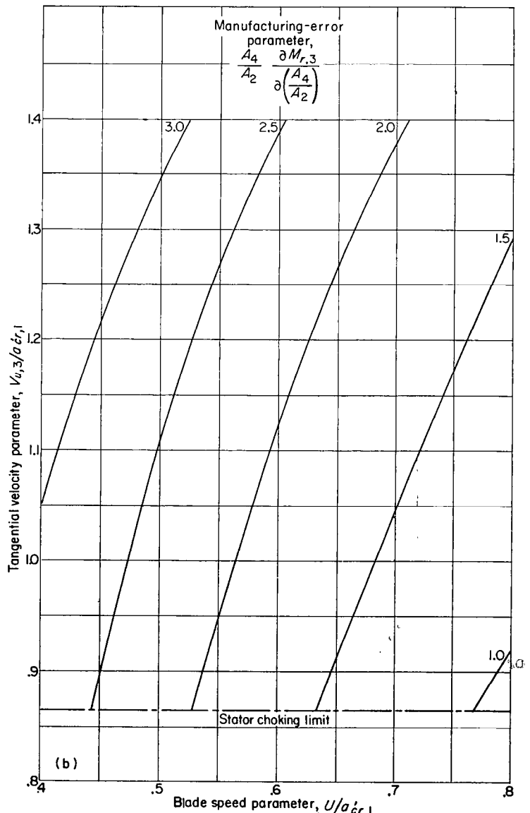
(b) Stator exit flow angle, 30^\circ .
