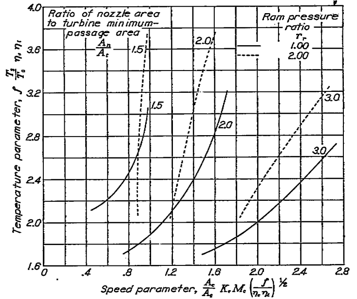
FIGURE 7.—Equilibrium operating lines for turbojet engine with several ratios of nozzle area to turbine minimum-passage area and two ram pressure ratios. Burner pressure ratio, 1.05.
