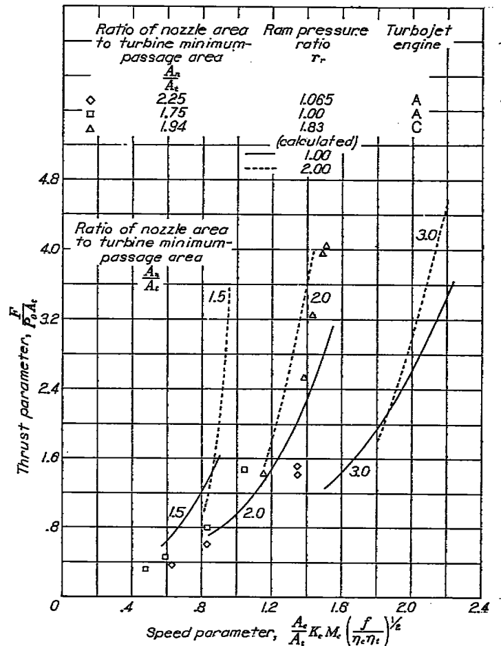
FIGURE 8.—Effect of speed parameter on turbojet-engine thrust for several ratios of nozzle area to turbine minimum-passage area and two ram pressure ratios. Burner pressure ratio, 1.05.
