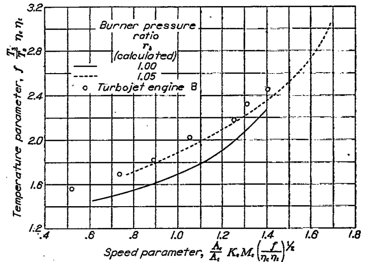
FIGURE 5.—Comparison of experimental data and calculated equilibrium operating lines for two assumed burner pressure ratios. Ratio of nozzle area to turbine minimum-passage area, 1.96; ram pressure ratio, 1.04.
