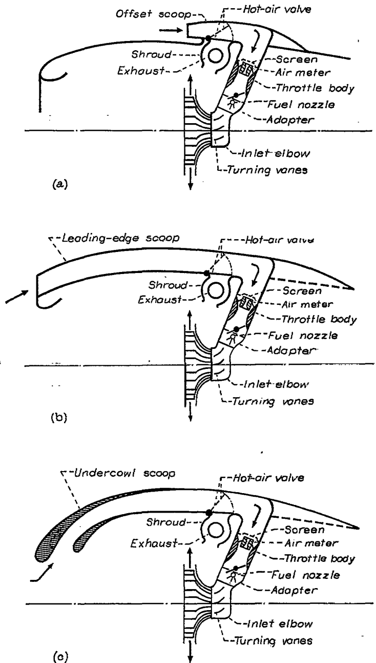
(a) With offset scoop. (b) With leading-edge scoop. (c) With undercowl scoop.
