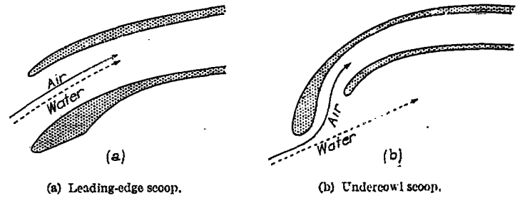
FIGURE 10.—Air and water-droplet paths for conventional and undercowl scoops.
