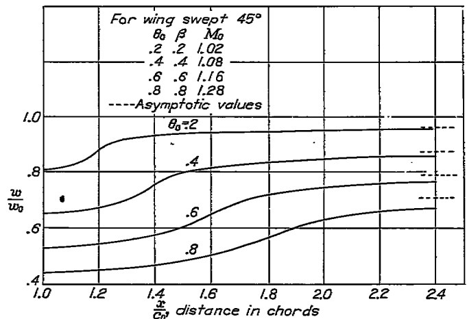
FIGURE 6.—Variation of downwash on x axis behind a triangular wing plotted as a function of distance in chord lengths.
