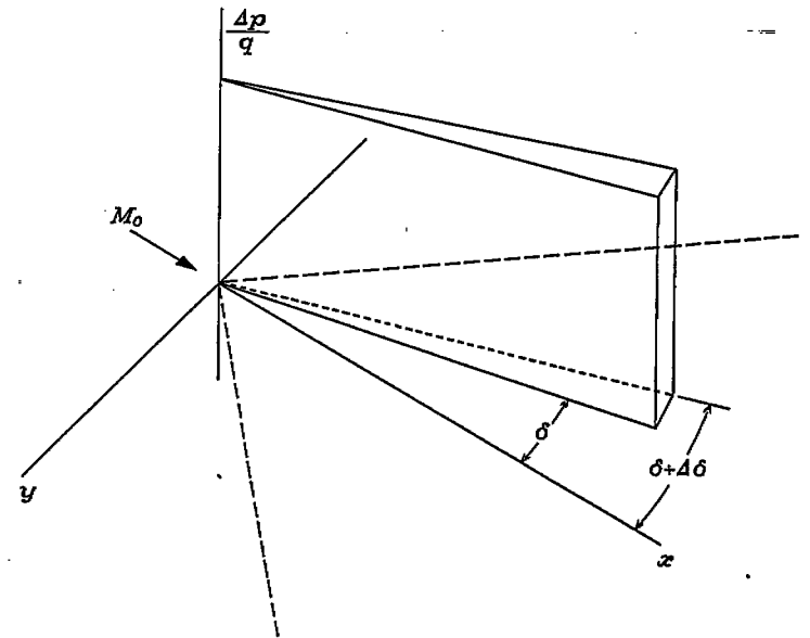
FIGURE 2.—Lifting-surface element carrying constant load.
