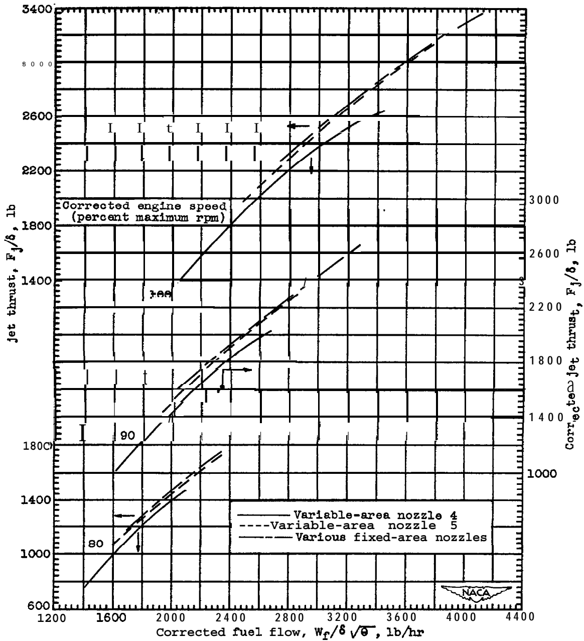
Figure 17. - Variation of corrected jet thrust with corrected fuel flow for variable-area nozzles 4 and 5 and various fixed-area nozzles at several engine speeds.
