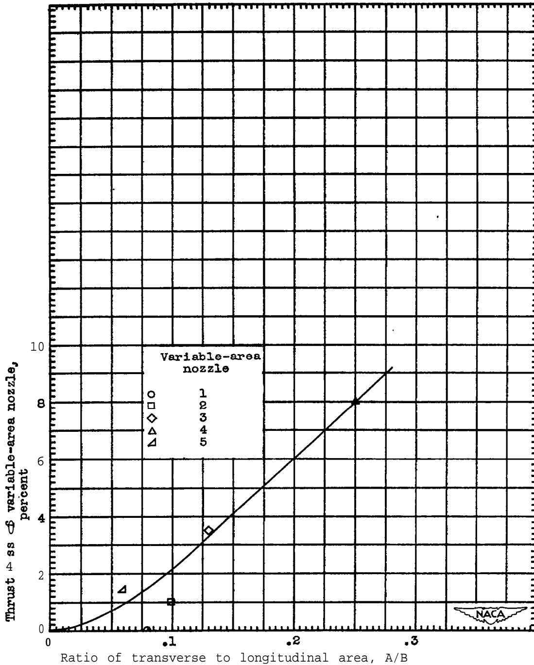
Figure 19. - Variation of thrust loss of variable-area nozzle at rated engine conditions with ratio of transverse to longitudinal projected outlet area A/B.
