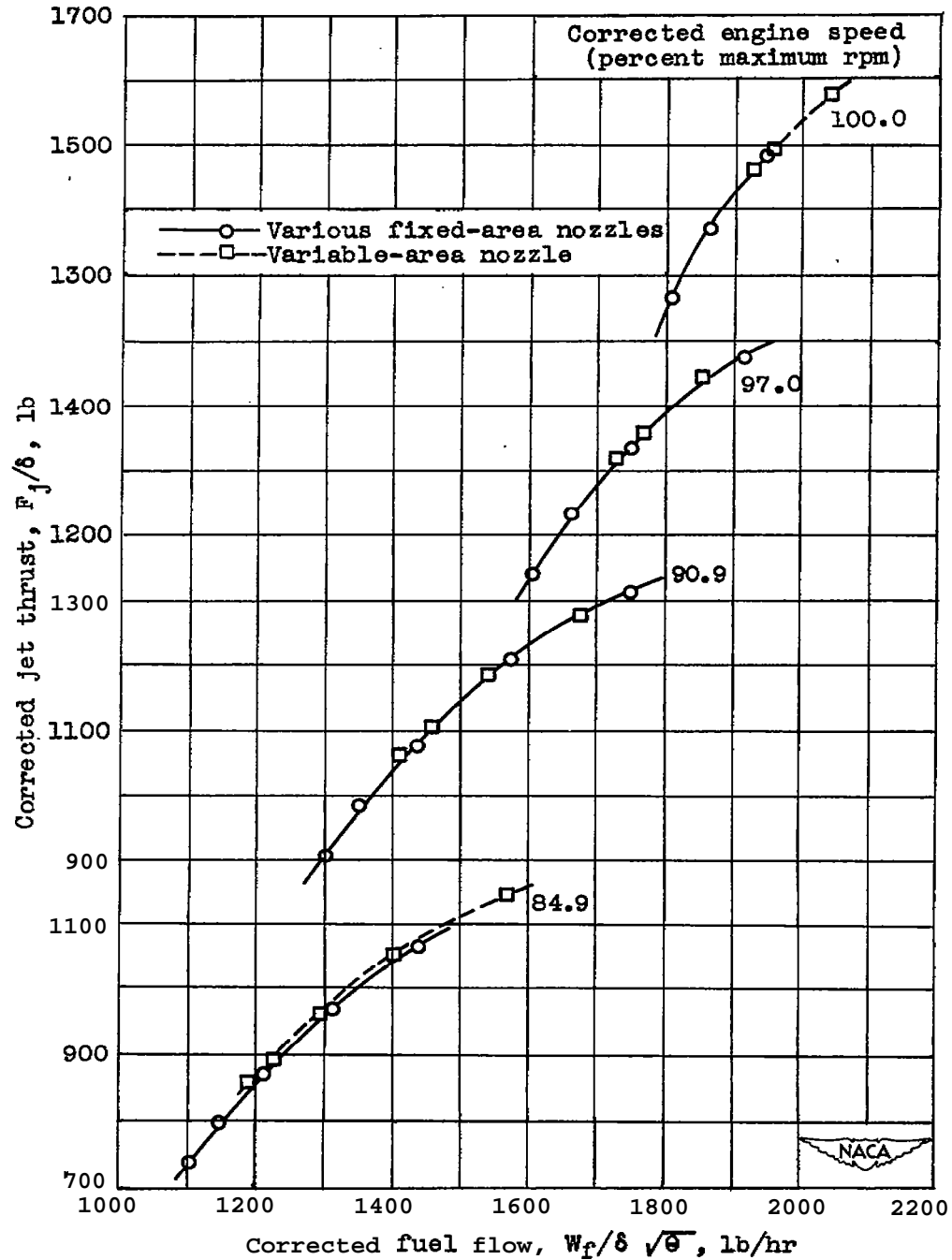
Figure 5. - Variation of corrected jet thrust with corrected fuel flow for variable-area nozzle 1 and various fixed-area nozzles at several engine speeds. (Figure taken from reference 1.)
