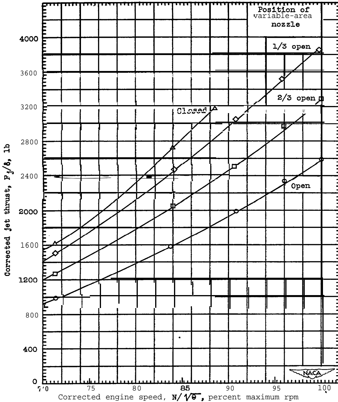
Figure 20. - Variation of corrected jet thrust with corrected engine speed for variable-area nozzle in various positions. Axial-flow turbojet engine at zero-ram sea-level conditions.
