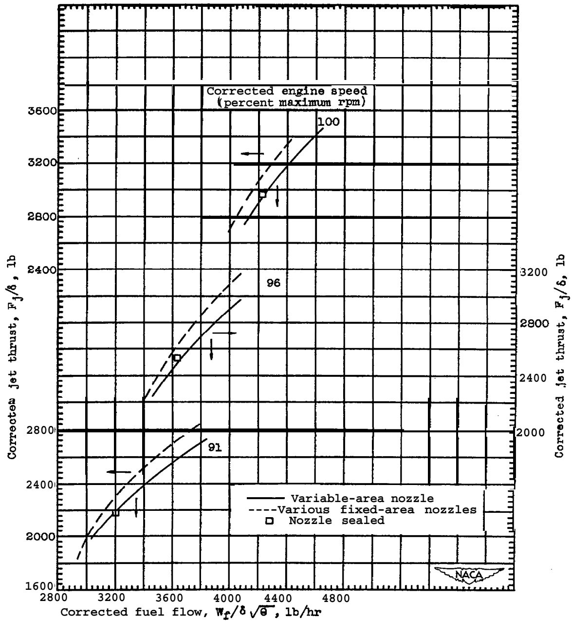
Figure 11. - Variation of corrected jet thrust with corrected fuel flow for variable-area nozzle 3 and various fixed-area nozzles at several engine speeds.
