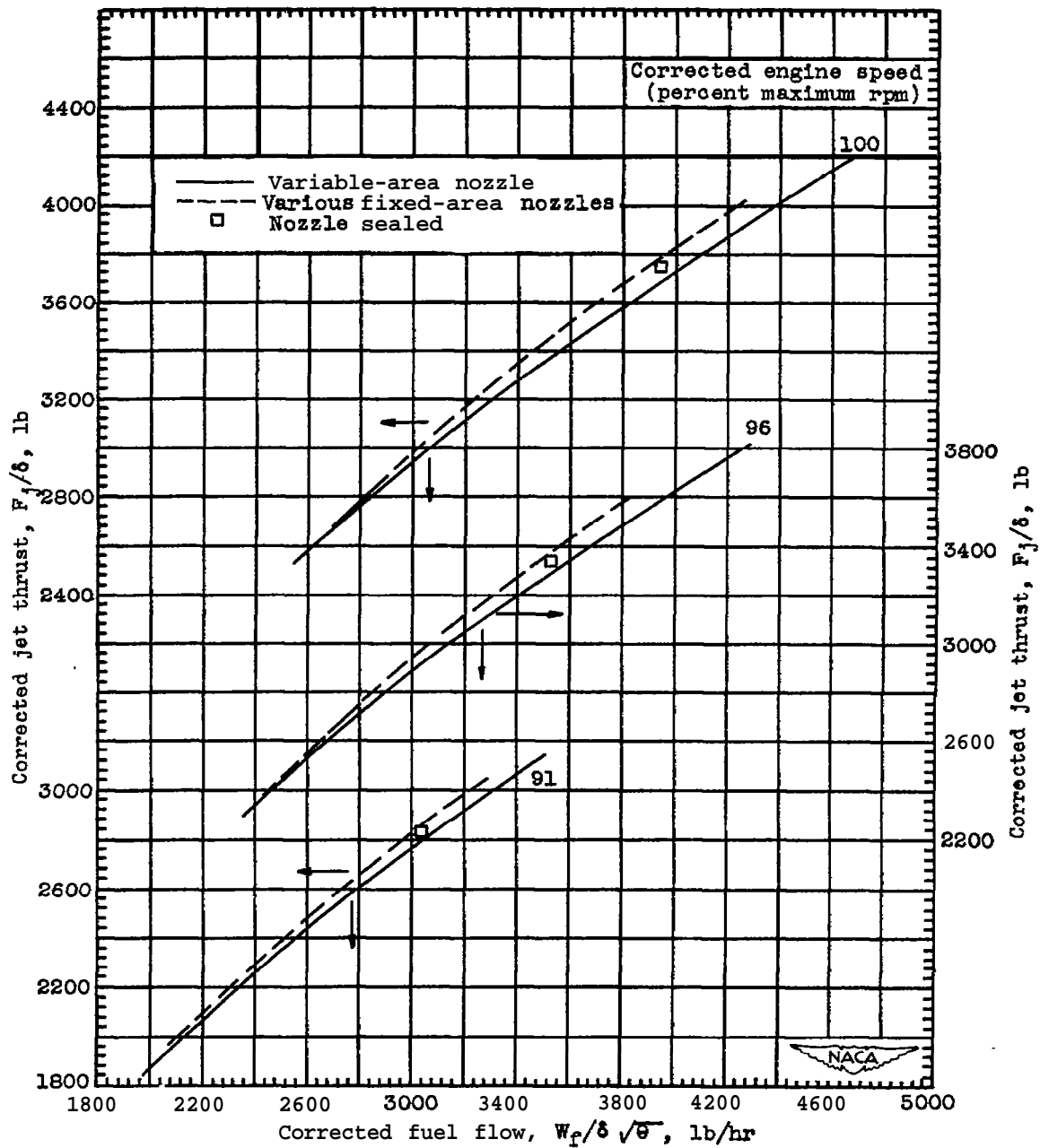
Figure 8. - Variation of corrected jet thrust with corrected fuel flow for variable-area nozzle 2 and various fixed-area nozzles at several engine speeds.
