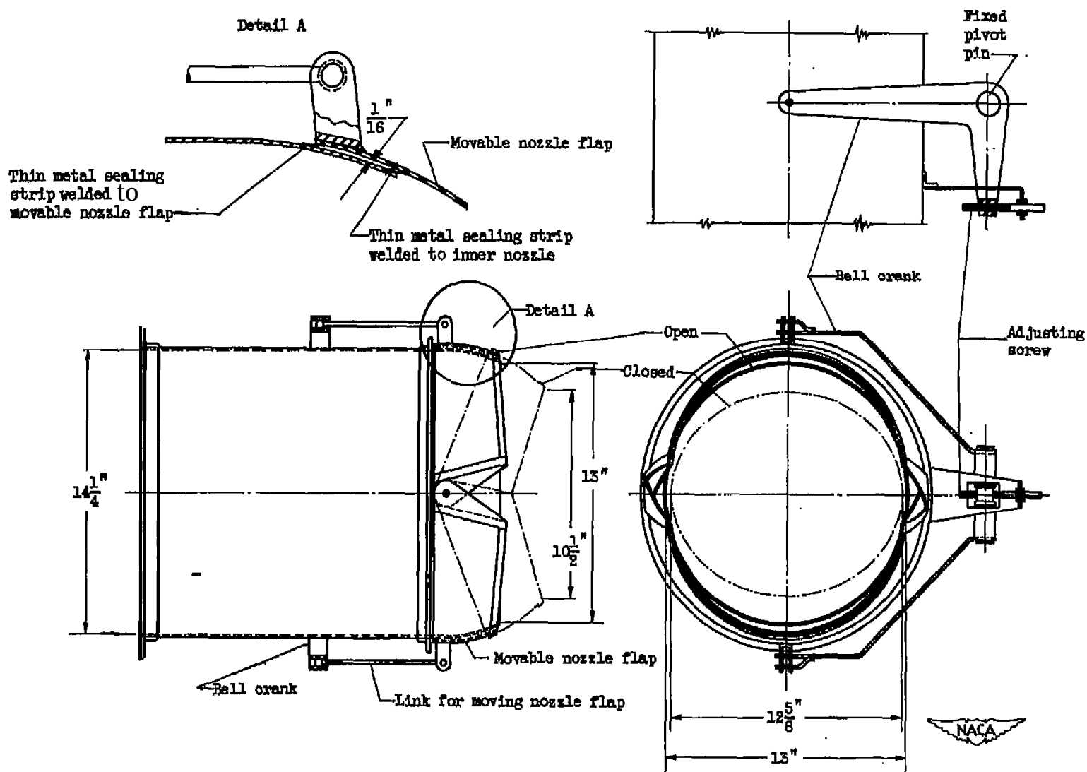
Figure 4. - Details of variable-area nozzle 1.
