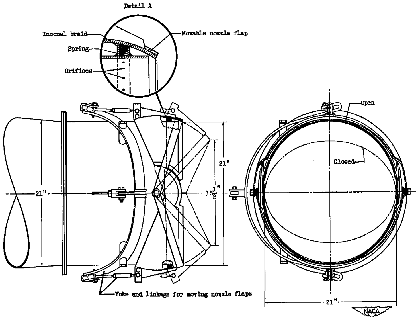
Figure 10. - Details of variable-area nozzle 3.
