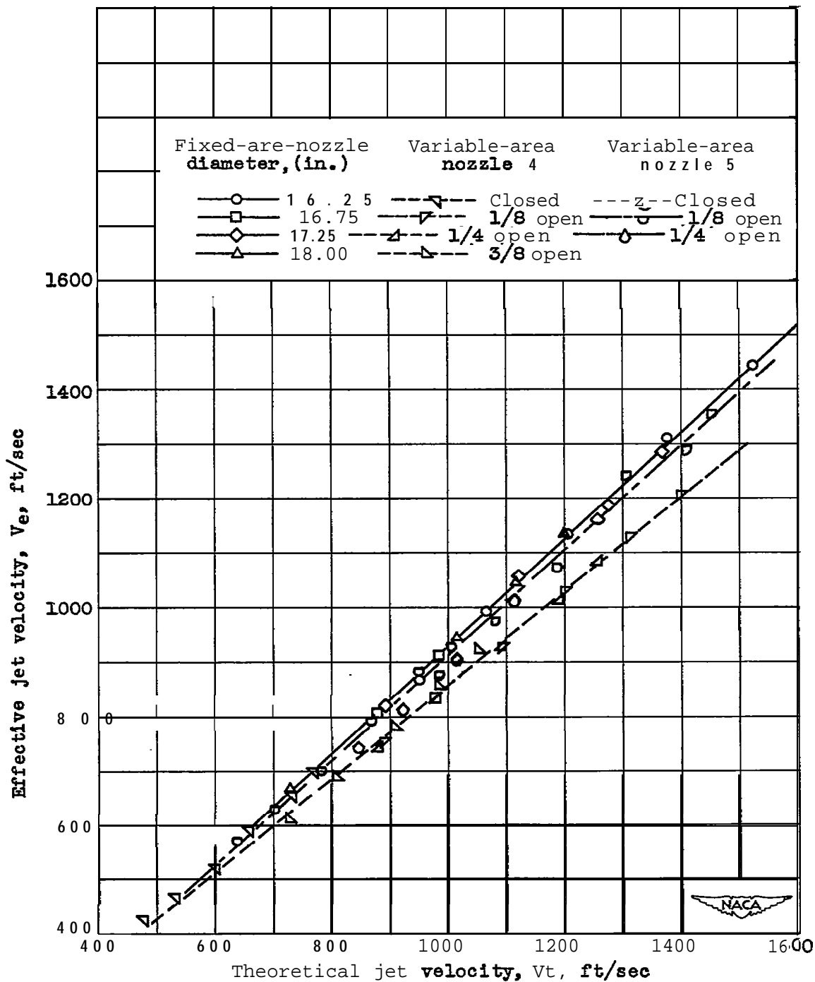
Figure 18. - Comparison of effective jet velocity with variable-area nozzles 4 and 5 and various fixed-area nozzles.
