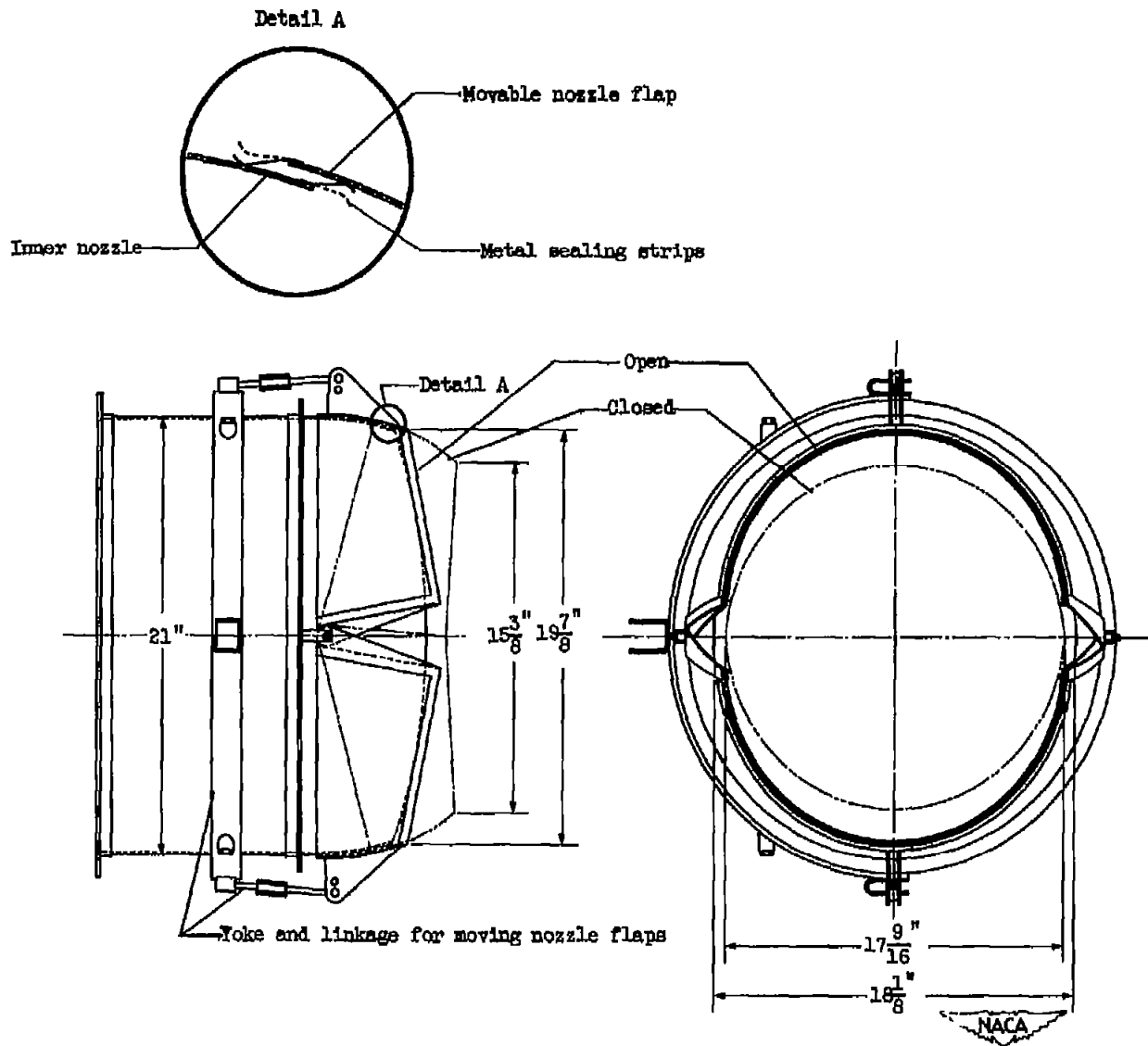
Figure 7. - Details of variable-area nozzle 2.
