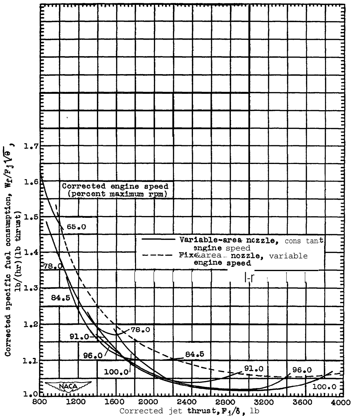
Figure 21. - Comparison of corrected specific fuel consumption of an axial-flow turbojet engine at zero-mm sea-level conditions with fixed- and variable-area nozzles.
