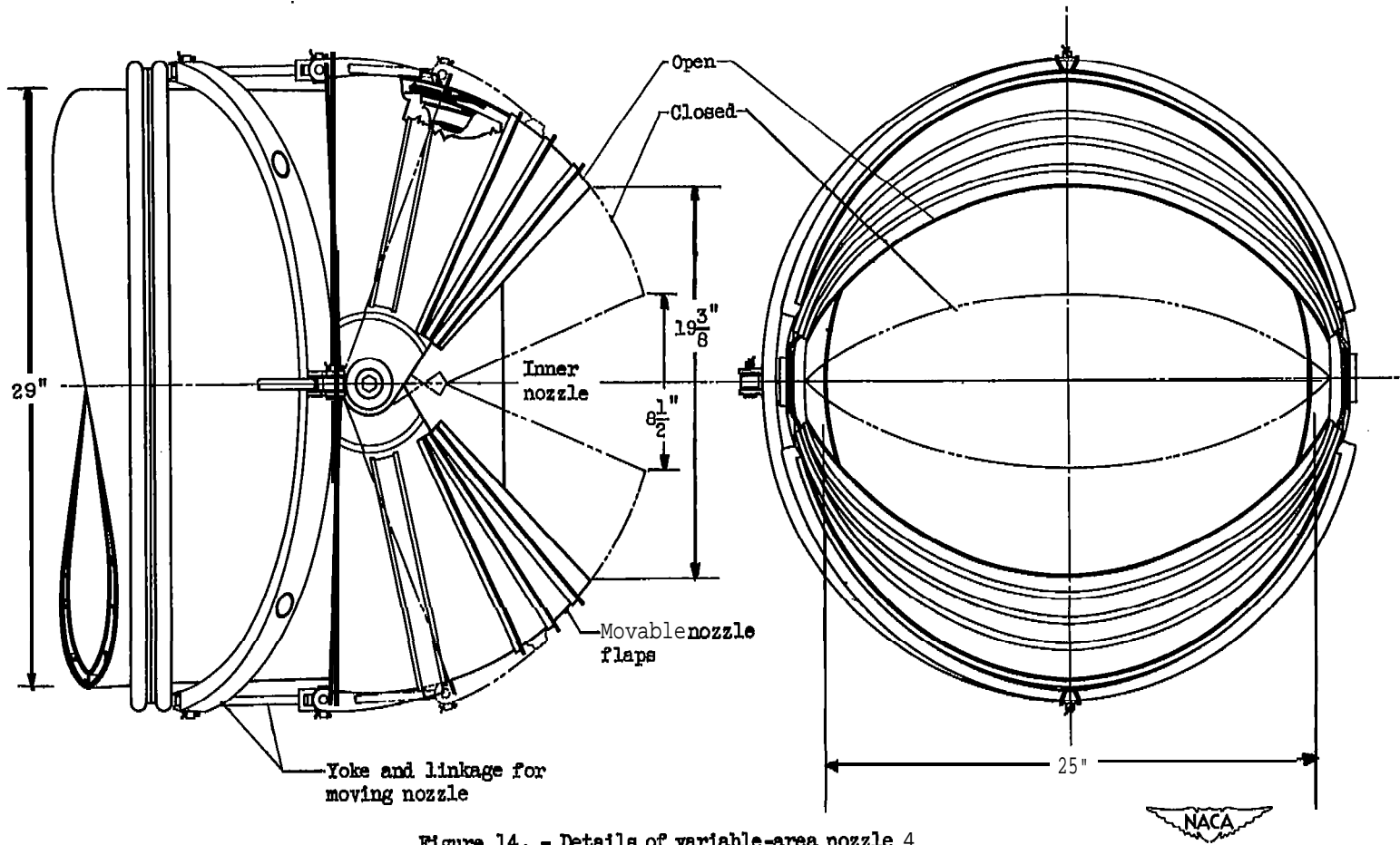
Figure 14. - Details of variable-area nozzle 4.
