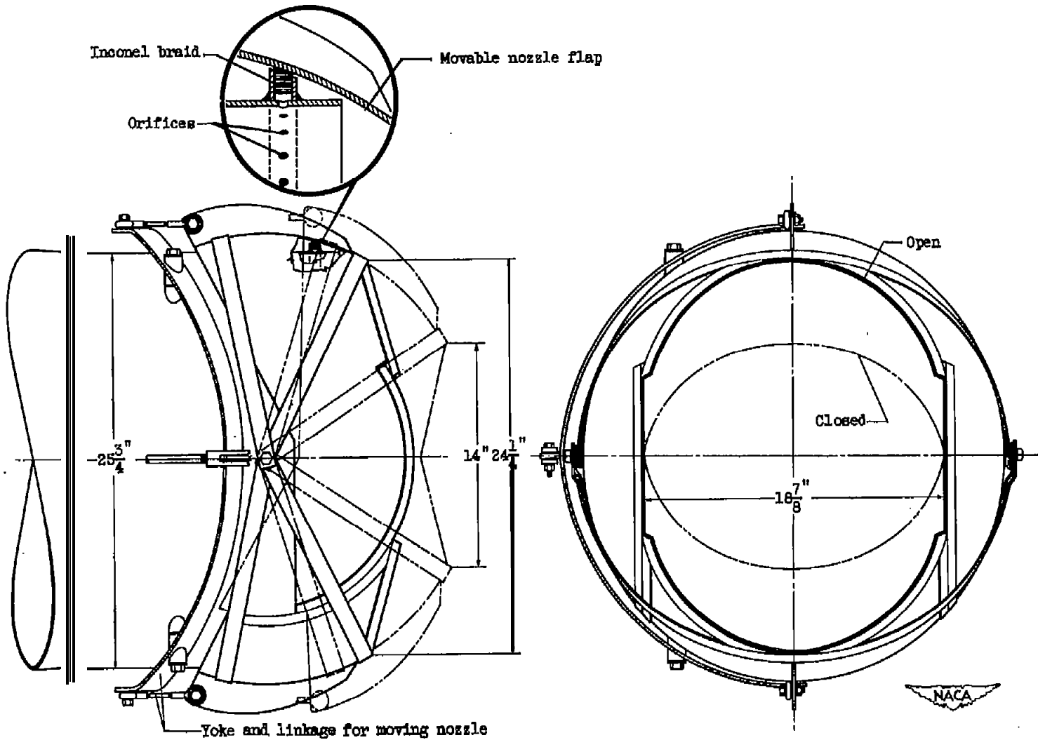
Figure 16. -Details of variable-area nozzle 5 .
