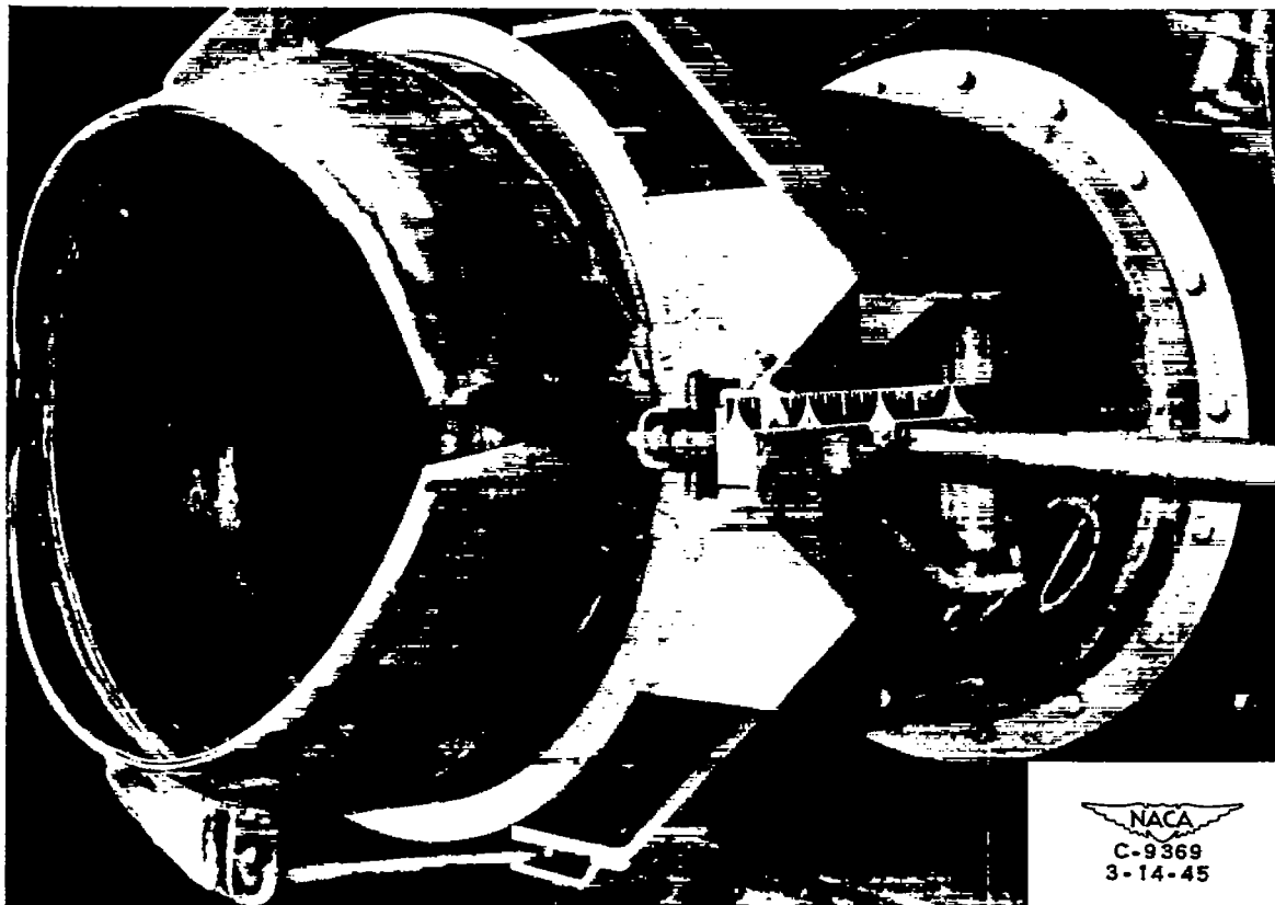
Figure 3. - Variable-area nozzle 1 installed on engine tail pipe.
