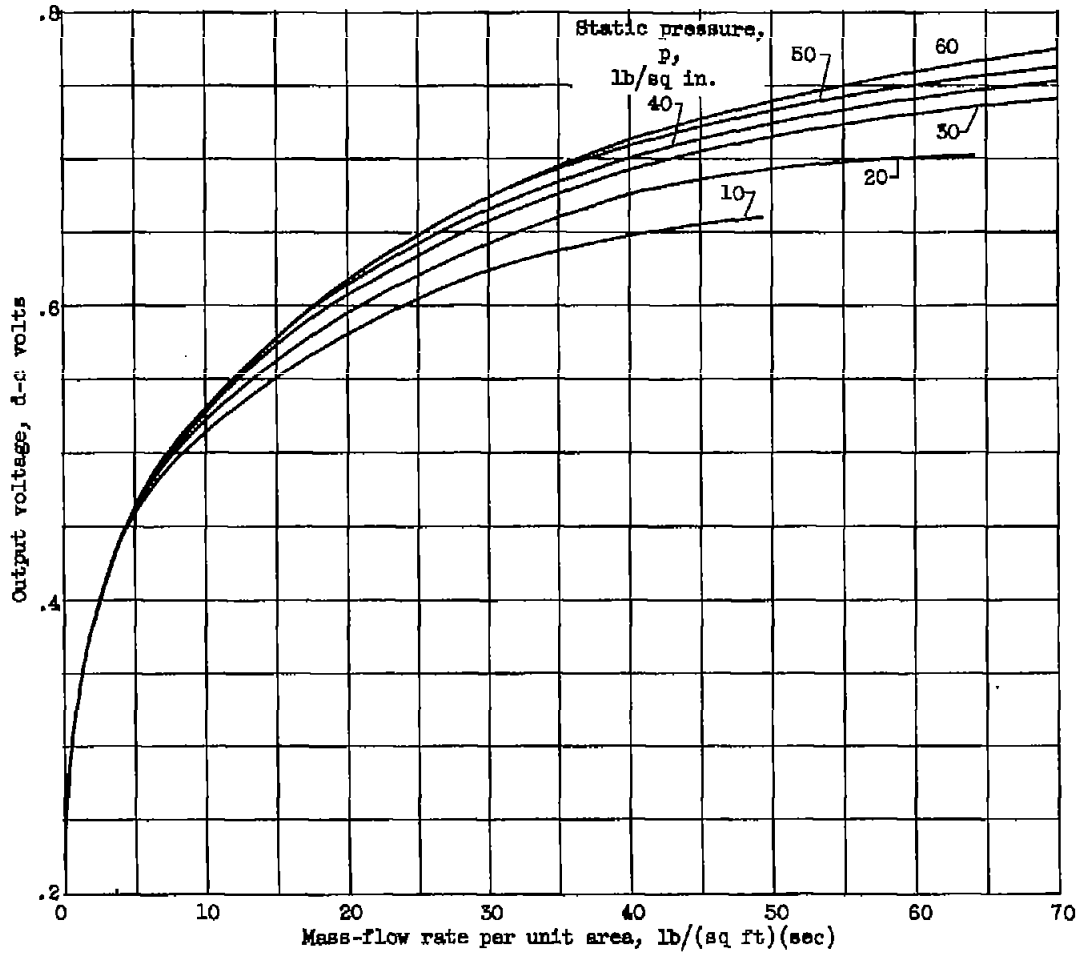
Figure 13. - Output voltage as a function of mass-flow rate for various static pressures. Air total temperature, 75° F.
