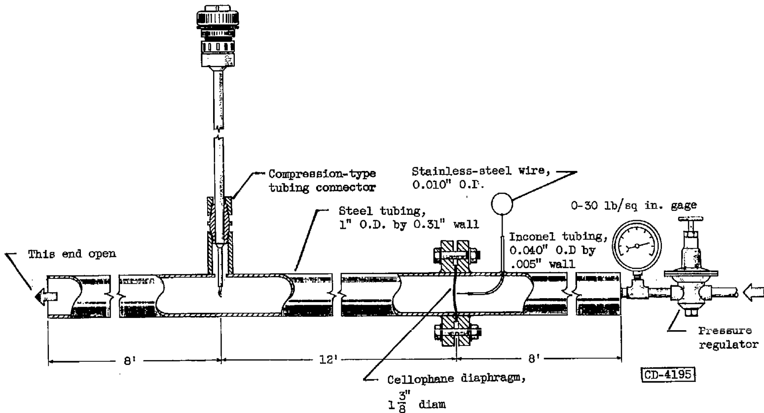
Figure 8. - Shock tube for determination of hot-wire anemometer response.
