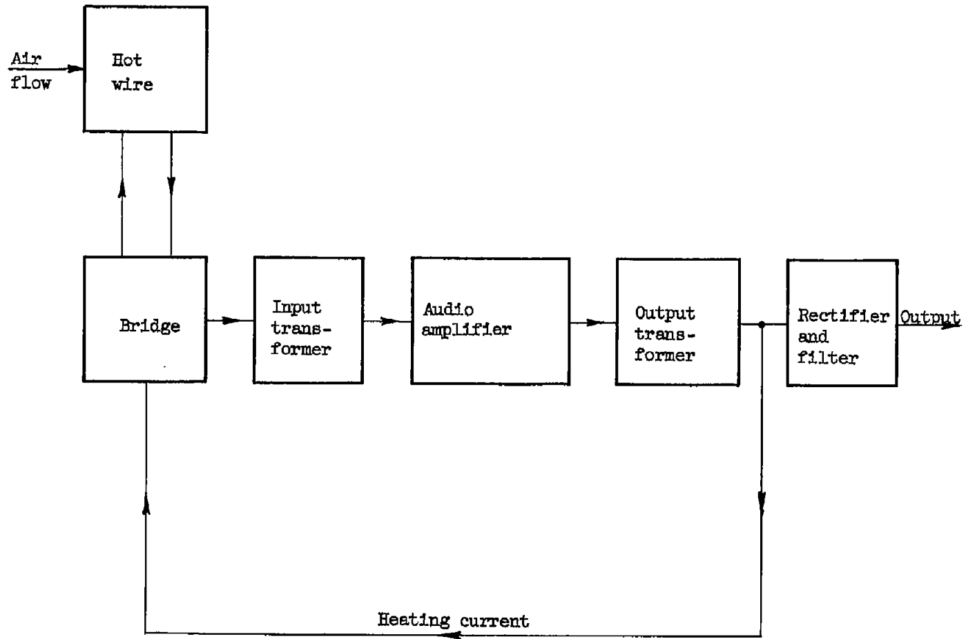
Figure 1. - Block diagram of self-excited, alternating-current, constant-temperature anemometer system.
