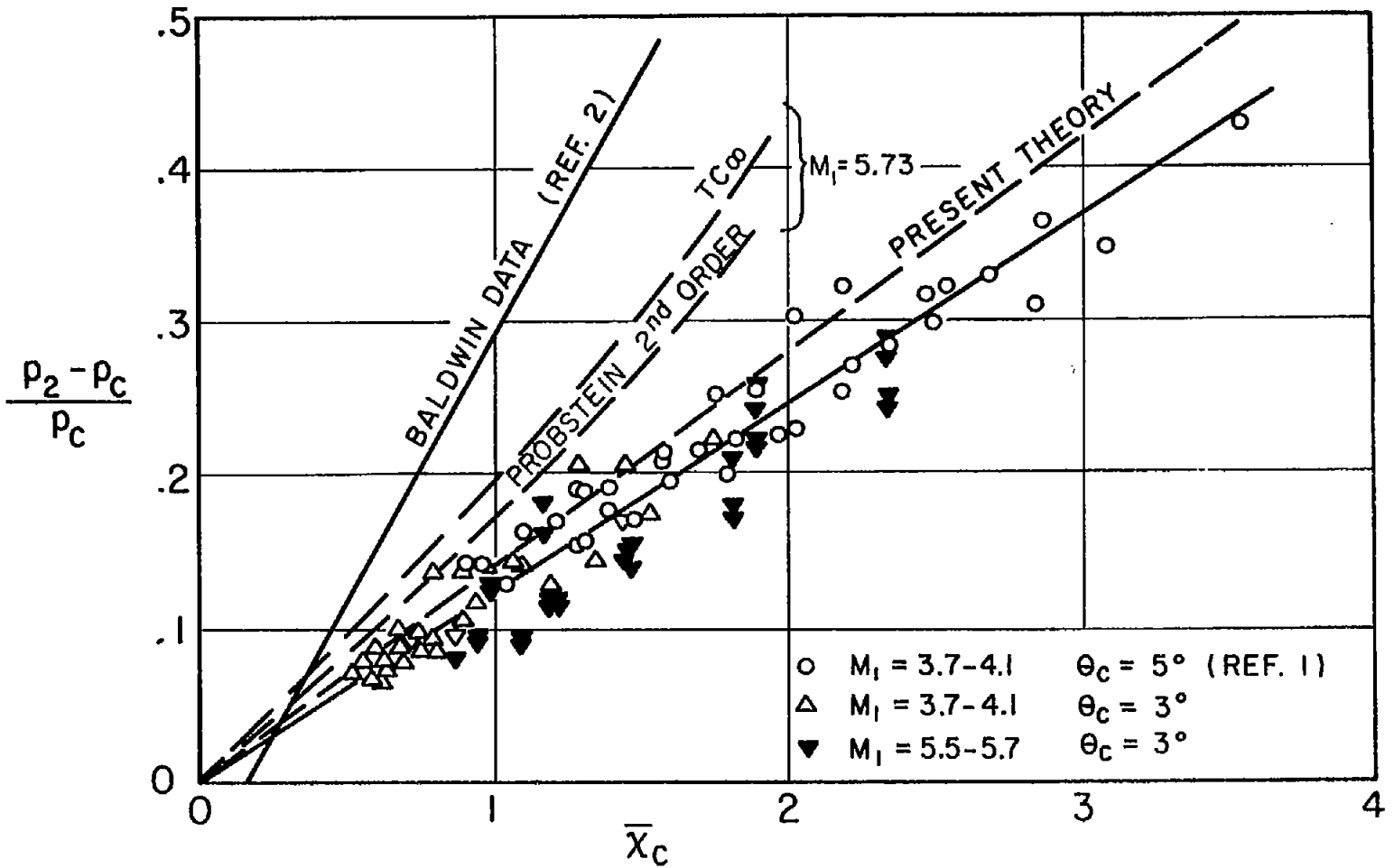
Figure 5. - Induced-pressure increment plotted against viscous-interaction parameter \bar{\chi}_c .
