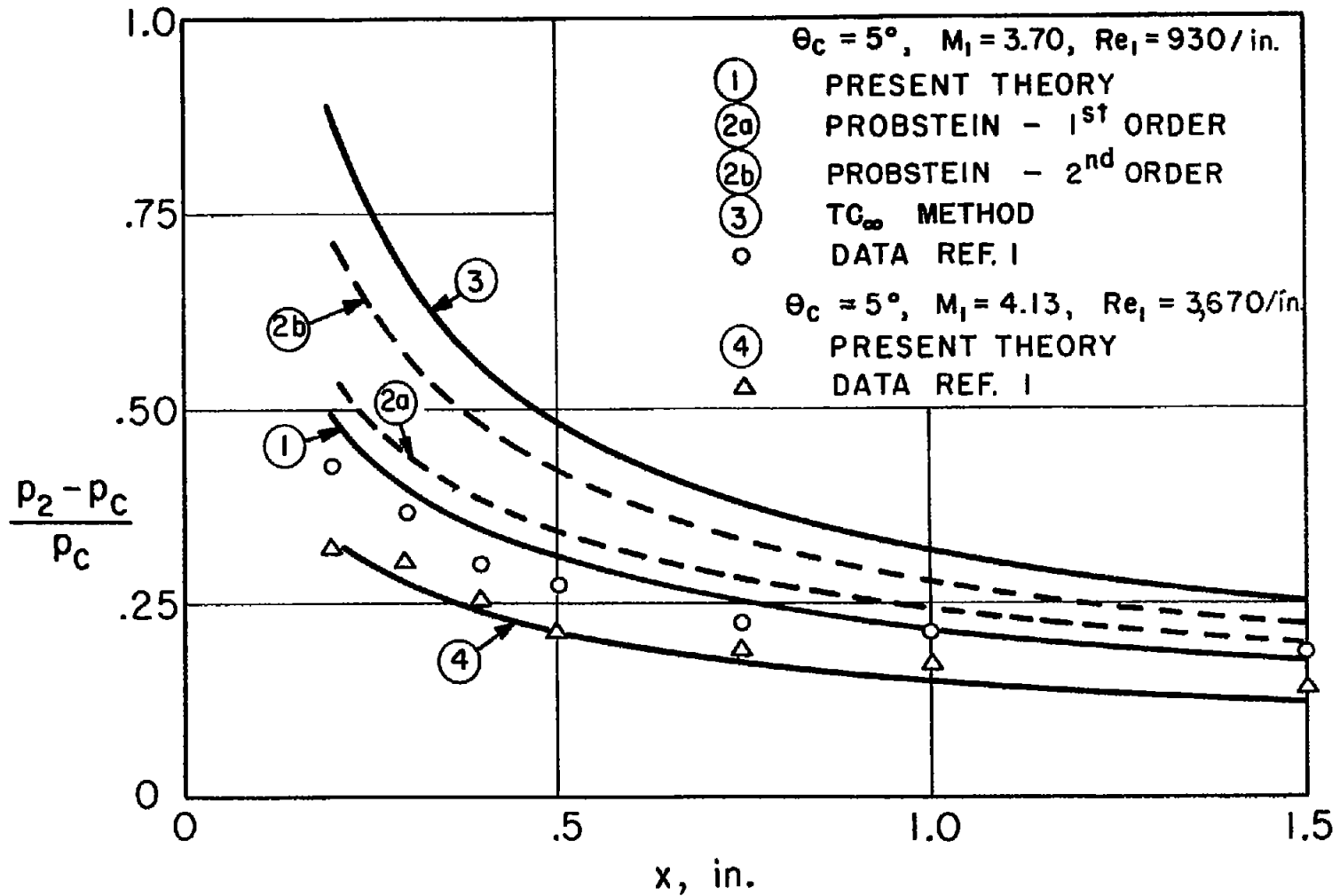
Figure 6. - Induced-pressure increment plotted against x for present data and data of reference 1.
