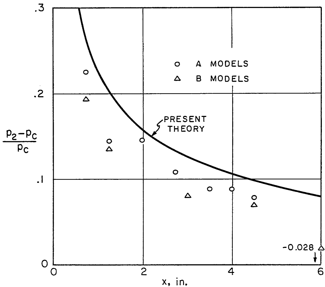
(a) Free-stream Mach number, 3.70; free-stream Reynolds number per inch, 880.
