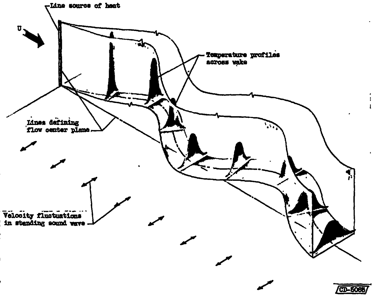
(a) Typical temperature profiles in molecular-diffusion wake at an instant. Figure 1. - Position of molecular-diffusion wake in mixing region.
