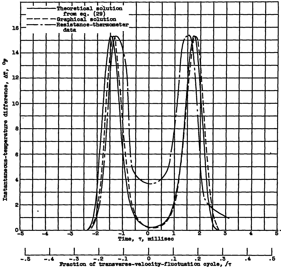
Figure 9. - Continued. Instantaneous temperature-time variation at various lateral positions. X = 2.98 inches or X/U = 1.47 .
