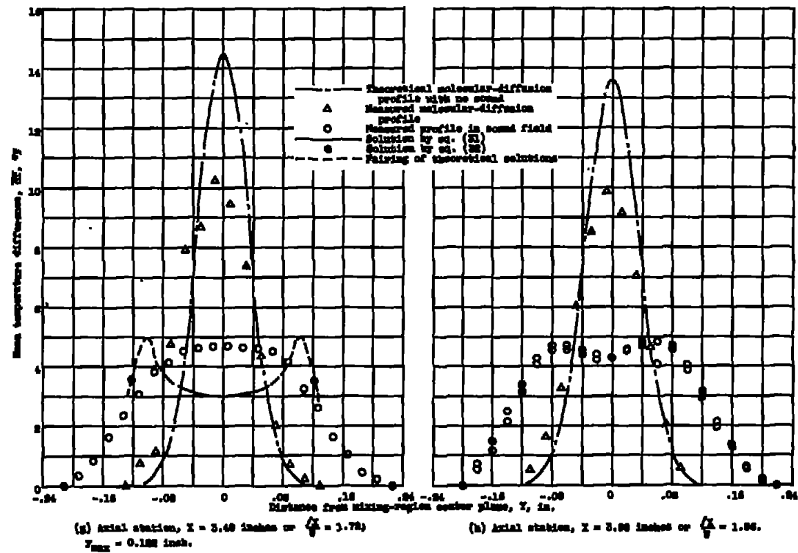
Figure 10. - Concluded. Comparison of theoretical and experimental time-mean temperature-difference profiles at various axial stations.
