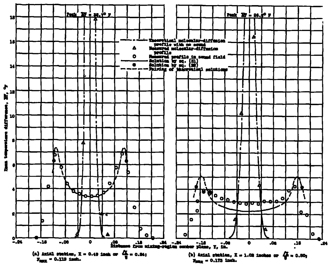
Figure 10. - Comparison of theoretical and experimental time-mean temperature-difference profiles at various axial stations.
