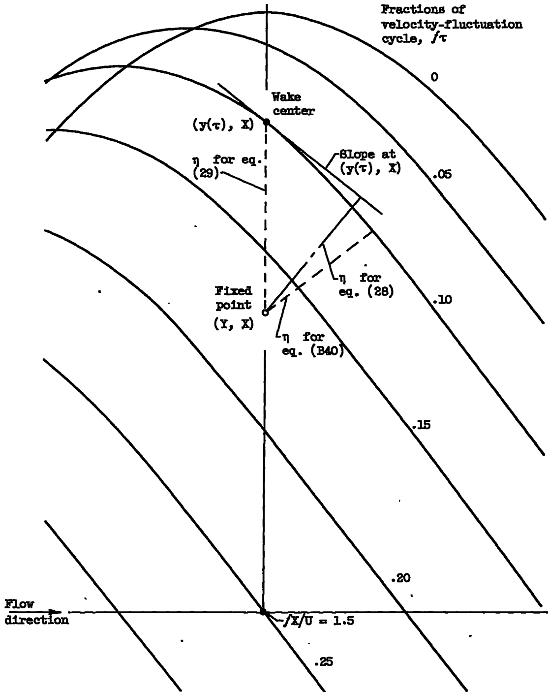
Figure 4. - Local diagram of position of molecular-diffusion-wake center at various times.
