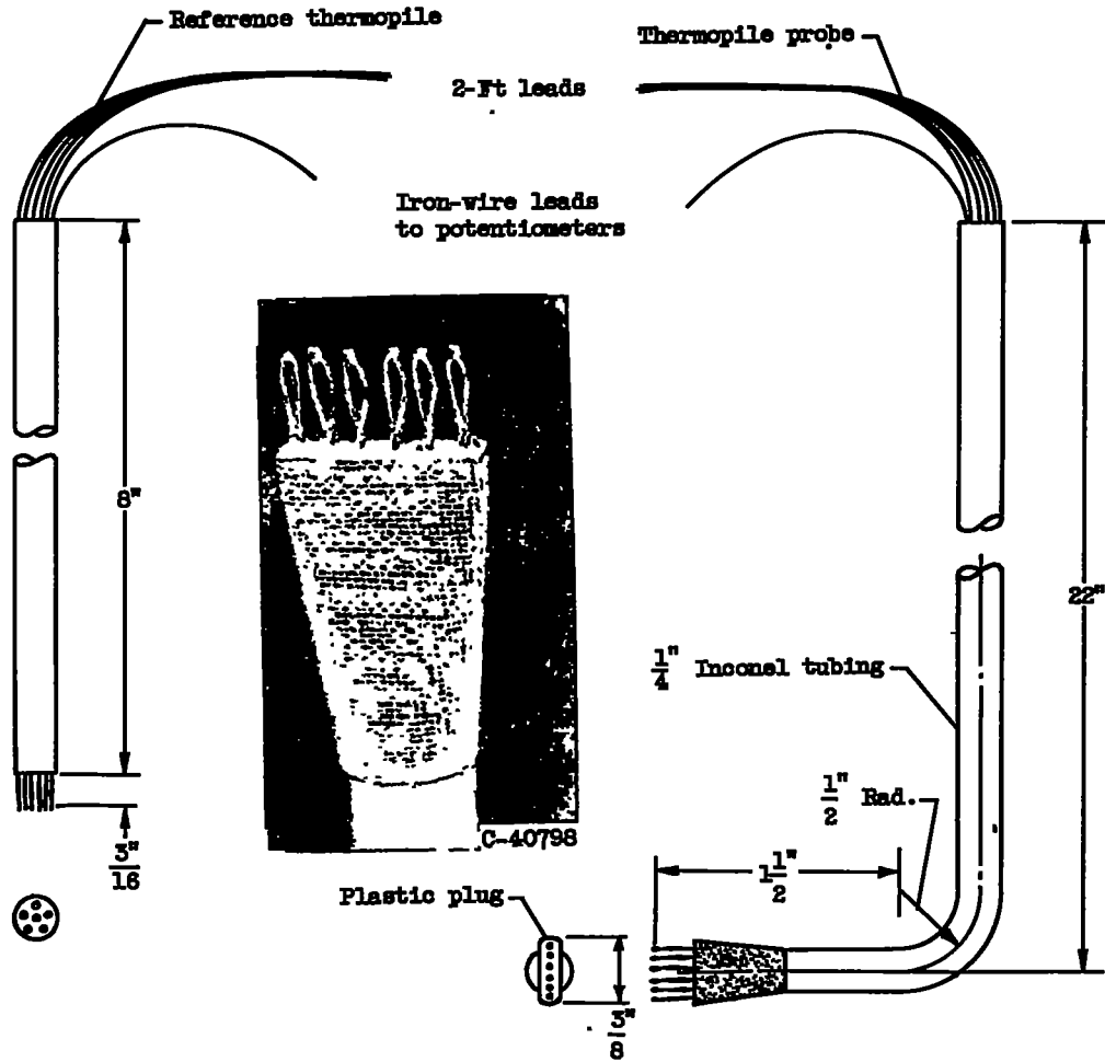
(a) Thermopile probe and reference thermopile.
