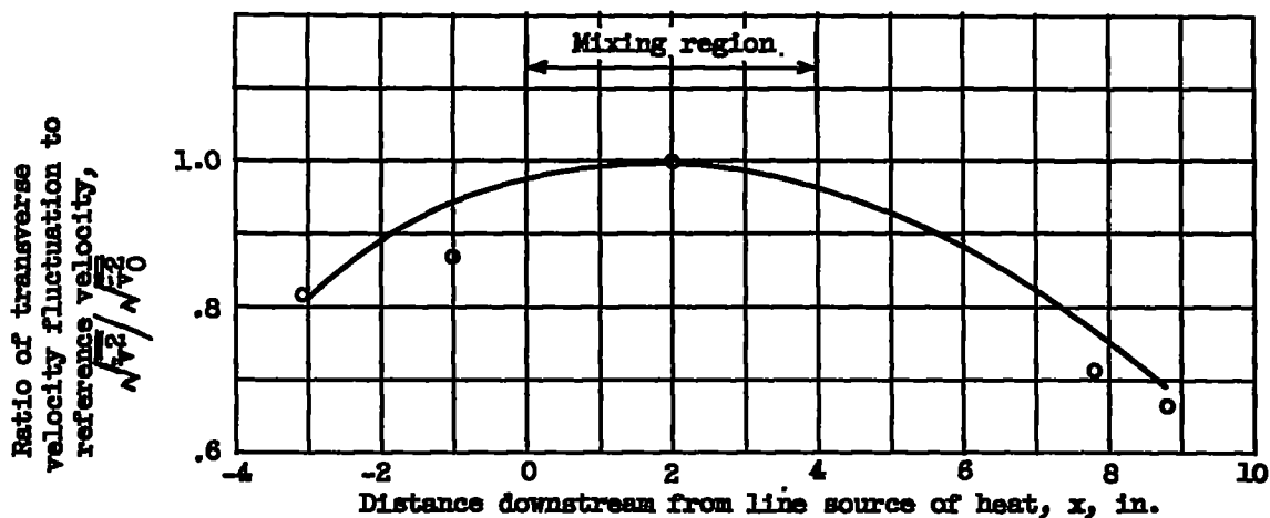
(b) Axial profile of velocity fluctuation in transverse standing sound wave. Reference root-mean-square transverse velocity fluctuation at x = 2 inches.
