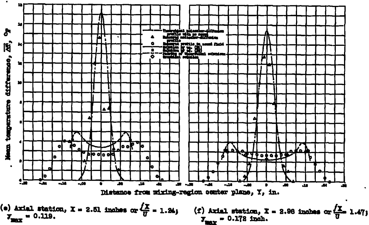
Figure 10. - Continued. Comparison of theoretical and experimental time-mean temperature-difference profiles at various axial stations.
