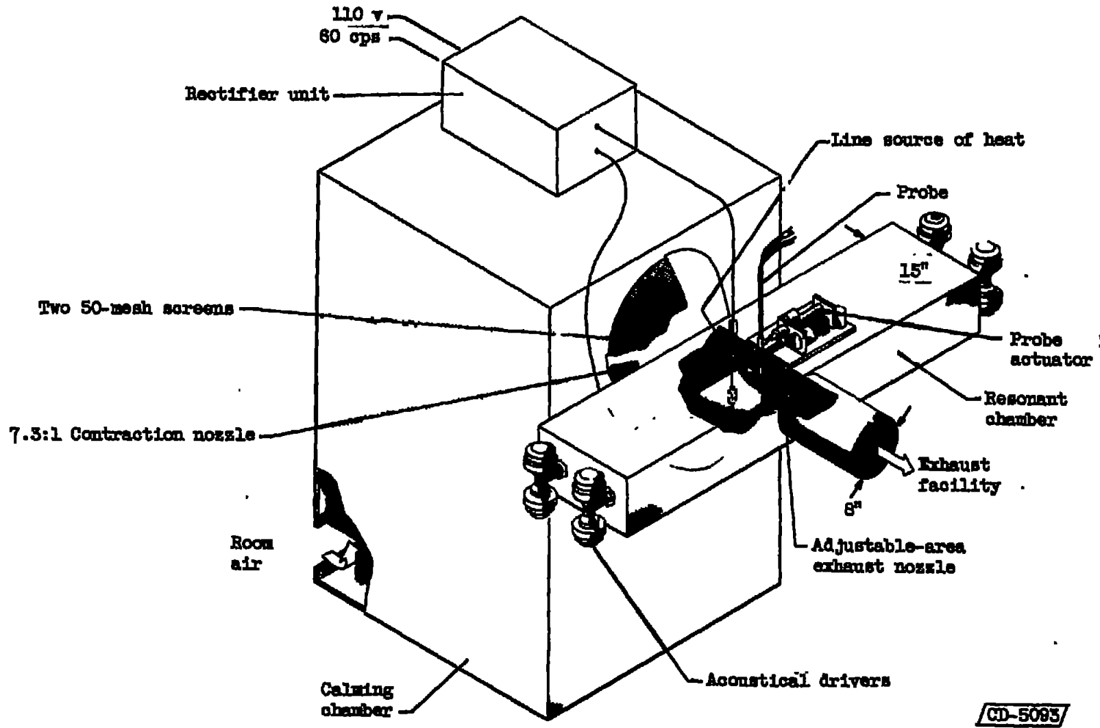
Figure 6. - Flow and sound-field apparatus.
