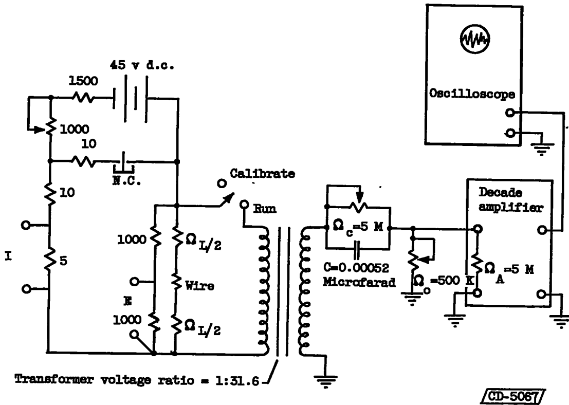
(b) Resistance-thermometer circuit.
