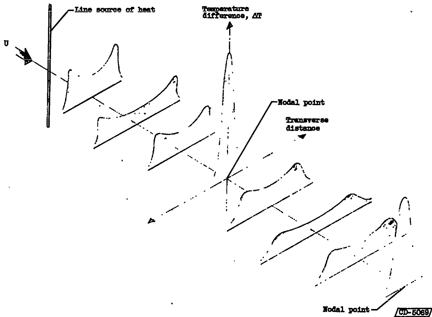
Figure 5. - Typical time-mean temperature profiles in mixing region for small deformation of the molecular-diffusion wake.
