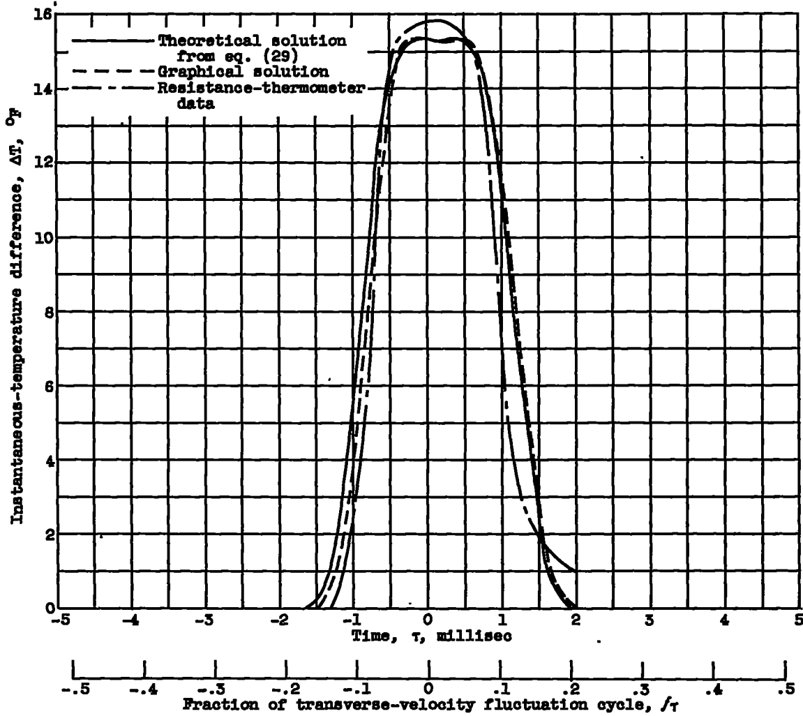
(c) Lateral position, Y = 0.17 inch or Y/y_{\max} = 0.98 .
