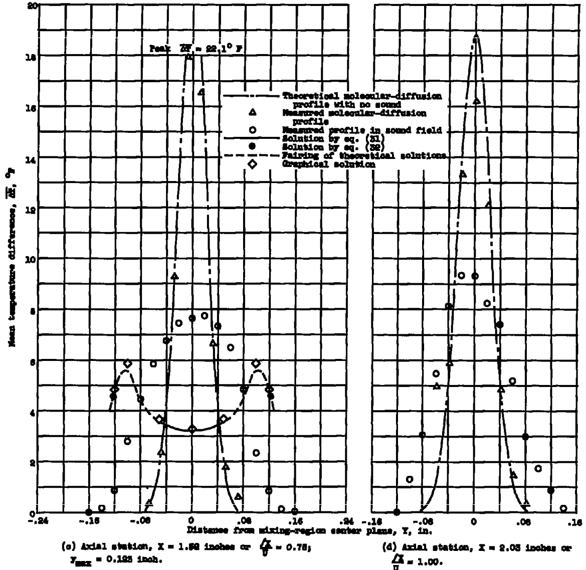
Figure 10. - Continued. Comparison of theoretical and experimental time-mean temperature-difference profiles at various axial stations.
