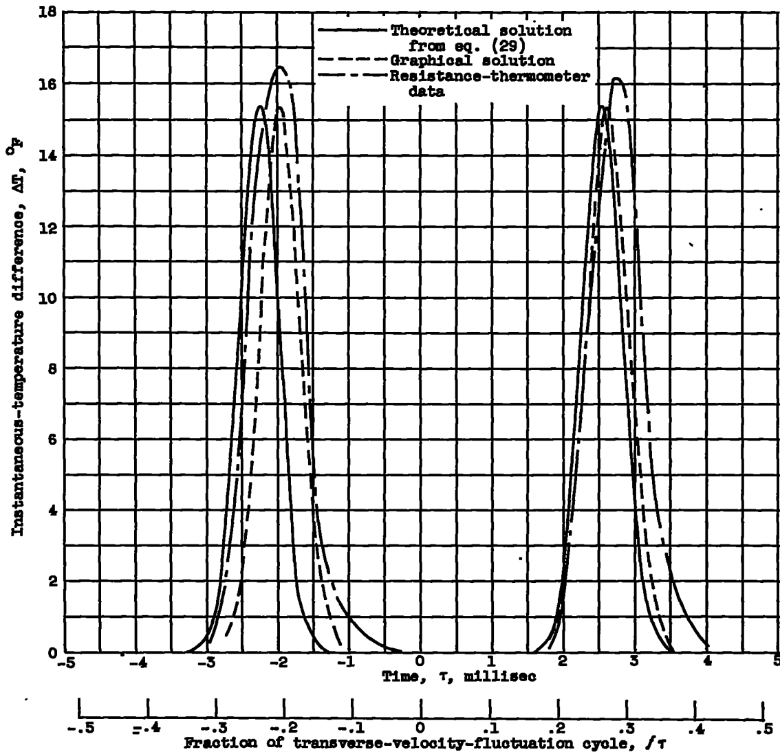
(a) Lateral position, Y = 0 inch.
