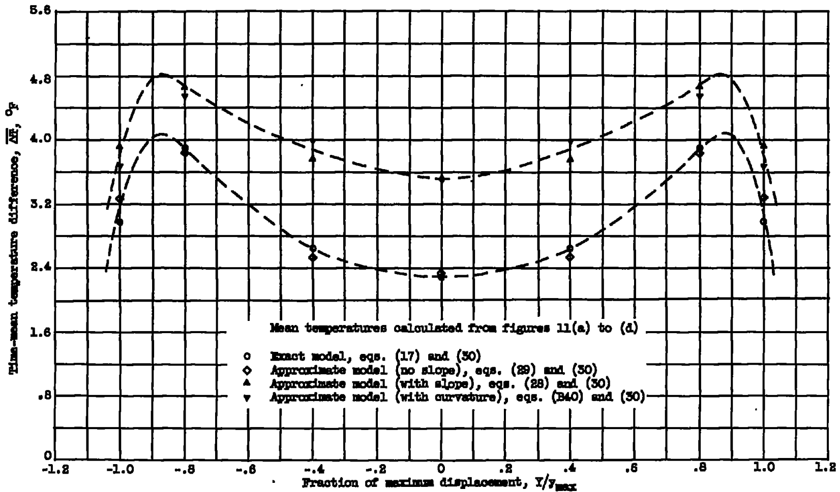
Figure 12. - Comparison of exact and approximate solutions for mean temperature. Dimensionless axial position, 7.5; coefficient of thermal diffusivity, 2.57 \times 10^{-4} square feet per second; stream-velocity - frequency ratio, 0.0358 foot; ratio of root-mean-square velocity fluctuation to stream velocity, 0.947; rate of heat release from line source per unit length, 0.0308 Btu per second per foot.
