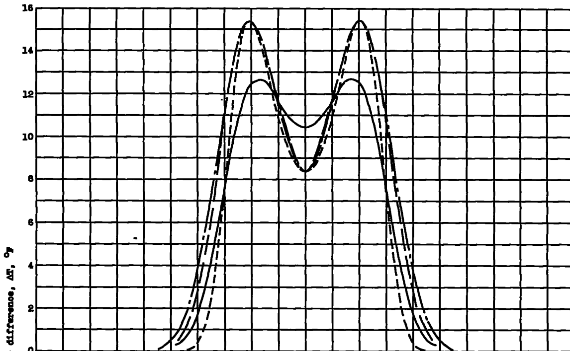
(c) Temperature-time variation at X/y_{max} = 0.8 .
