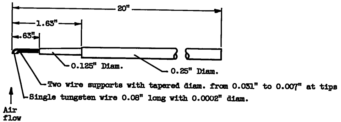
(a) Resistance-thermometer probe.
