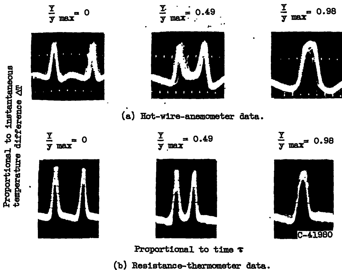
Figure 8. - Instantaneous-temperature-difference oscillograms. X = 2.98 inches or \frac{X}{U} = 1.47 .
