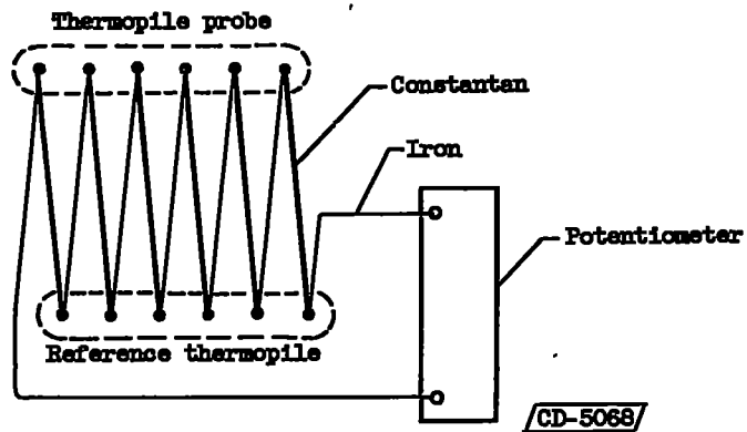
(b) Thermopile circuit.
