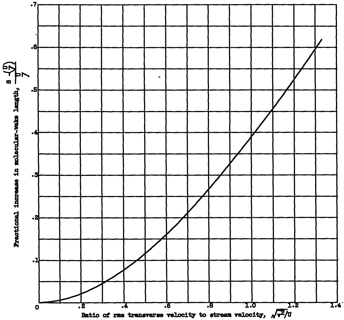
(a) Stretching of molecular-diffusion wake.
