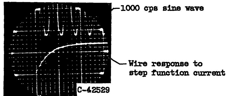
(a) Oscillogram
