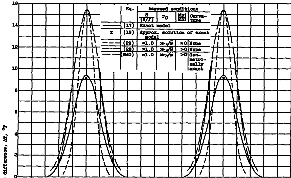
(a) Temperature-time variation at Y/y_{max} = 0 .
