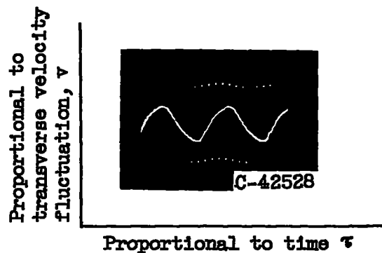
(a) Typical oscillogram of transverse velocity fluctuation.
