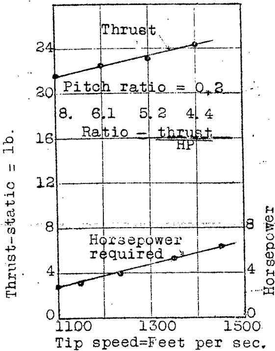
Fig. 8. Thrust & HP required for outer 3 1/2" of the 22" propeller.
