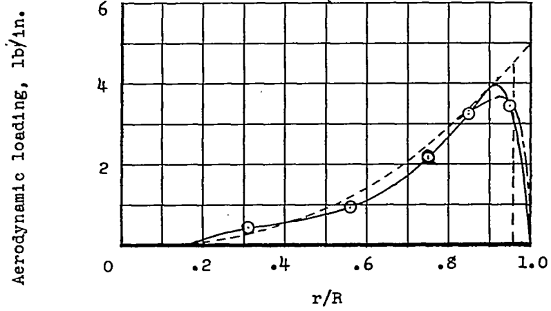
(a) \Omega R = 452 ft/sec; \theta = 5.6^\circ ; C_T = 0.00277 .
