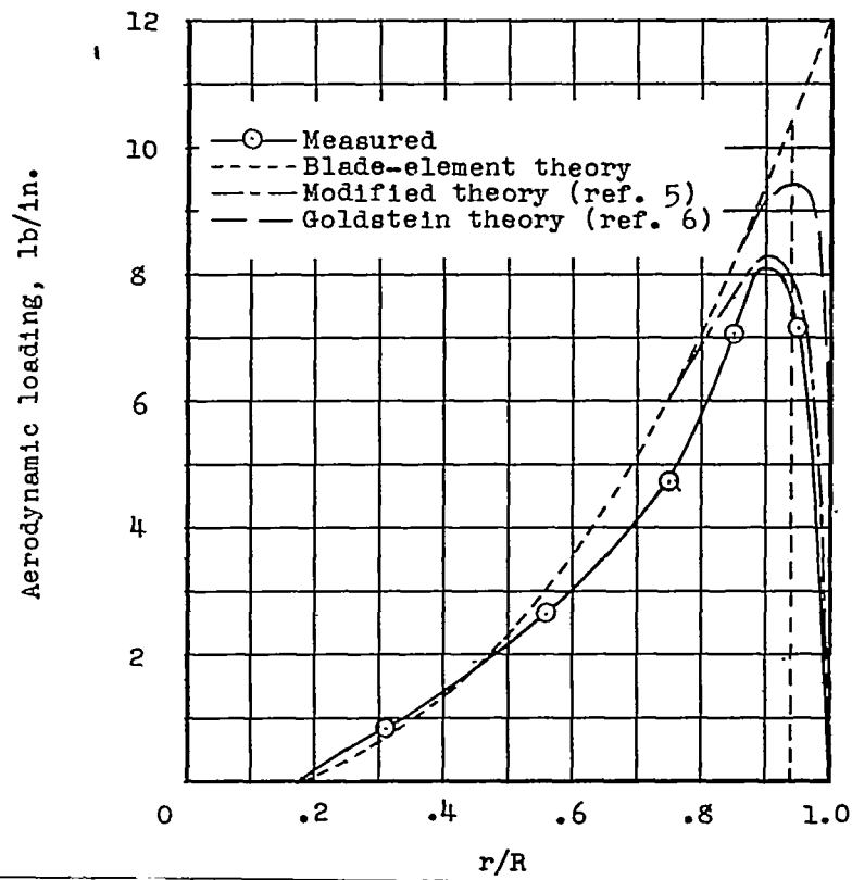
(a) \Omega R = 452 ft/sec; \theta = 5.6^\circ ; C_T = 0.00277 .
