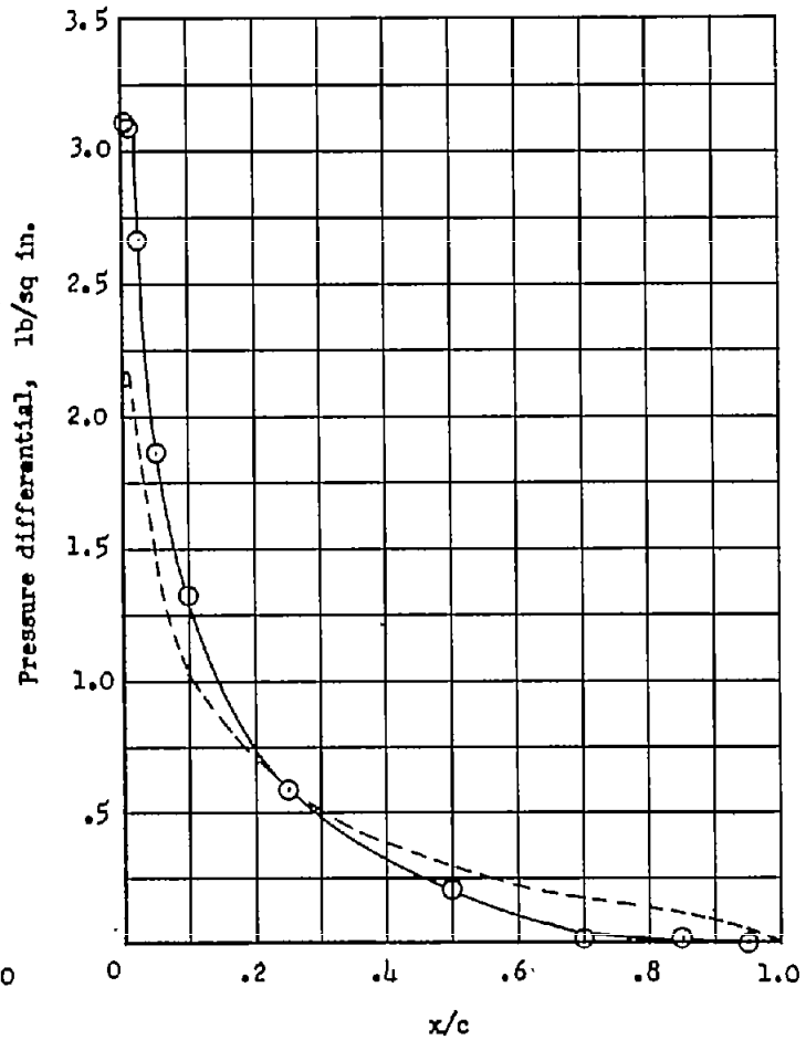
(b) r/R = 0.95 ; C_l = 0.264 .
