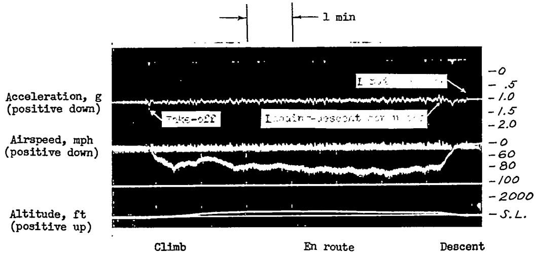
(a) Sample record identifying traces.
