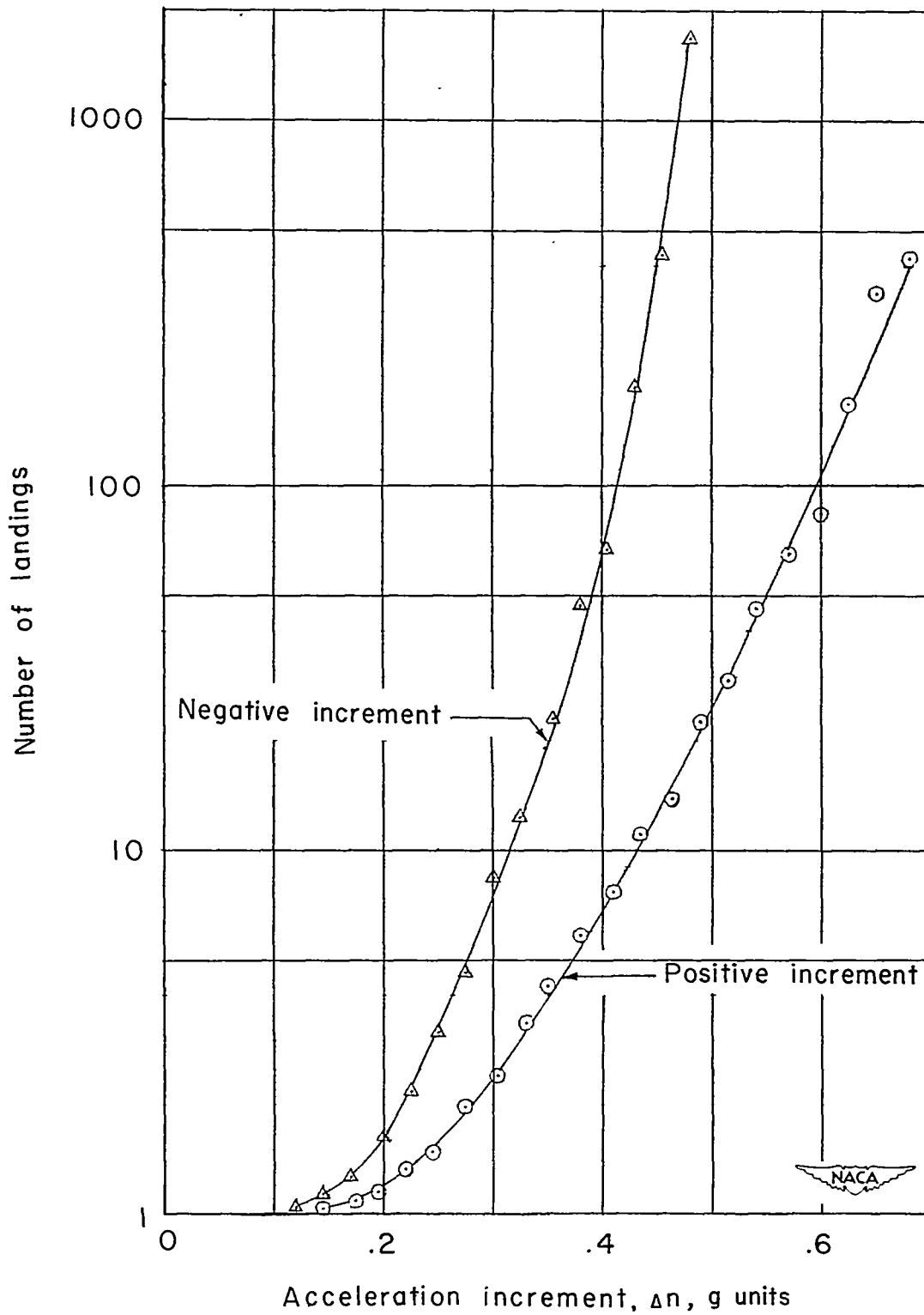
Figure 8.- Average number of landings required to equal or exceed a given value of acceleration increment.
