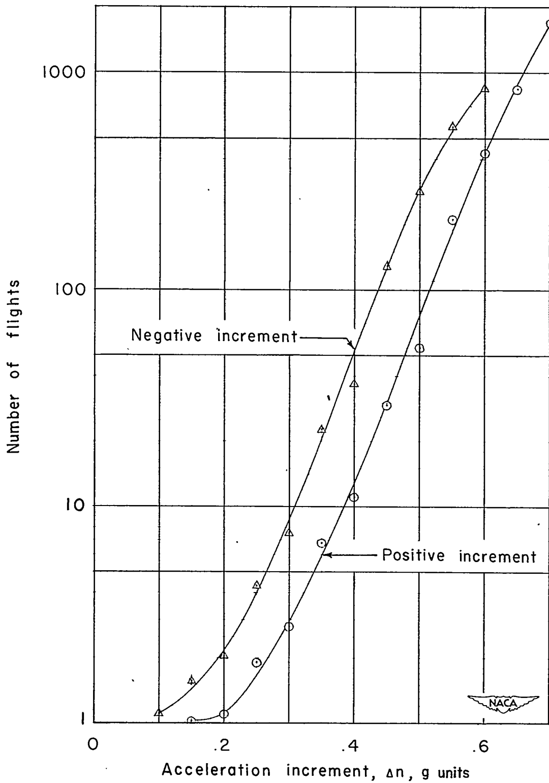
Figure 6.- Average number of flights required to equal or exceed a given value of acceleration increment.
