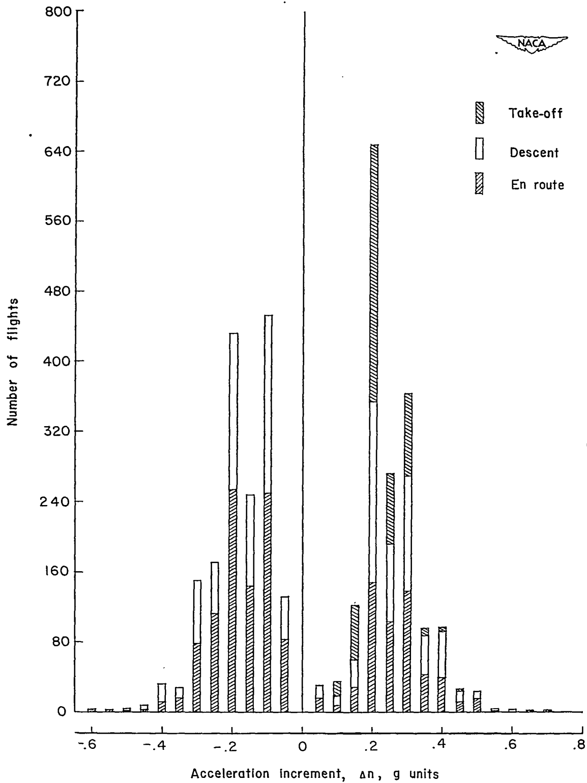
Figure 5.- Total number of flights in which the stated value of acceleration increment was the extreme reached.
