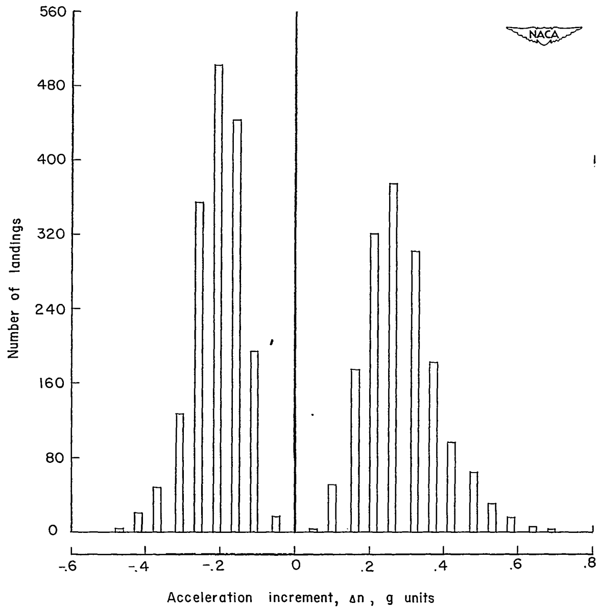
Figure 7.- Total number of landings in which the stated value of acceleration increment was the extreme reached.
