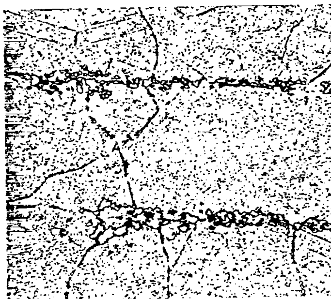
Interior, 1000X
