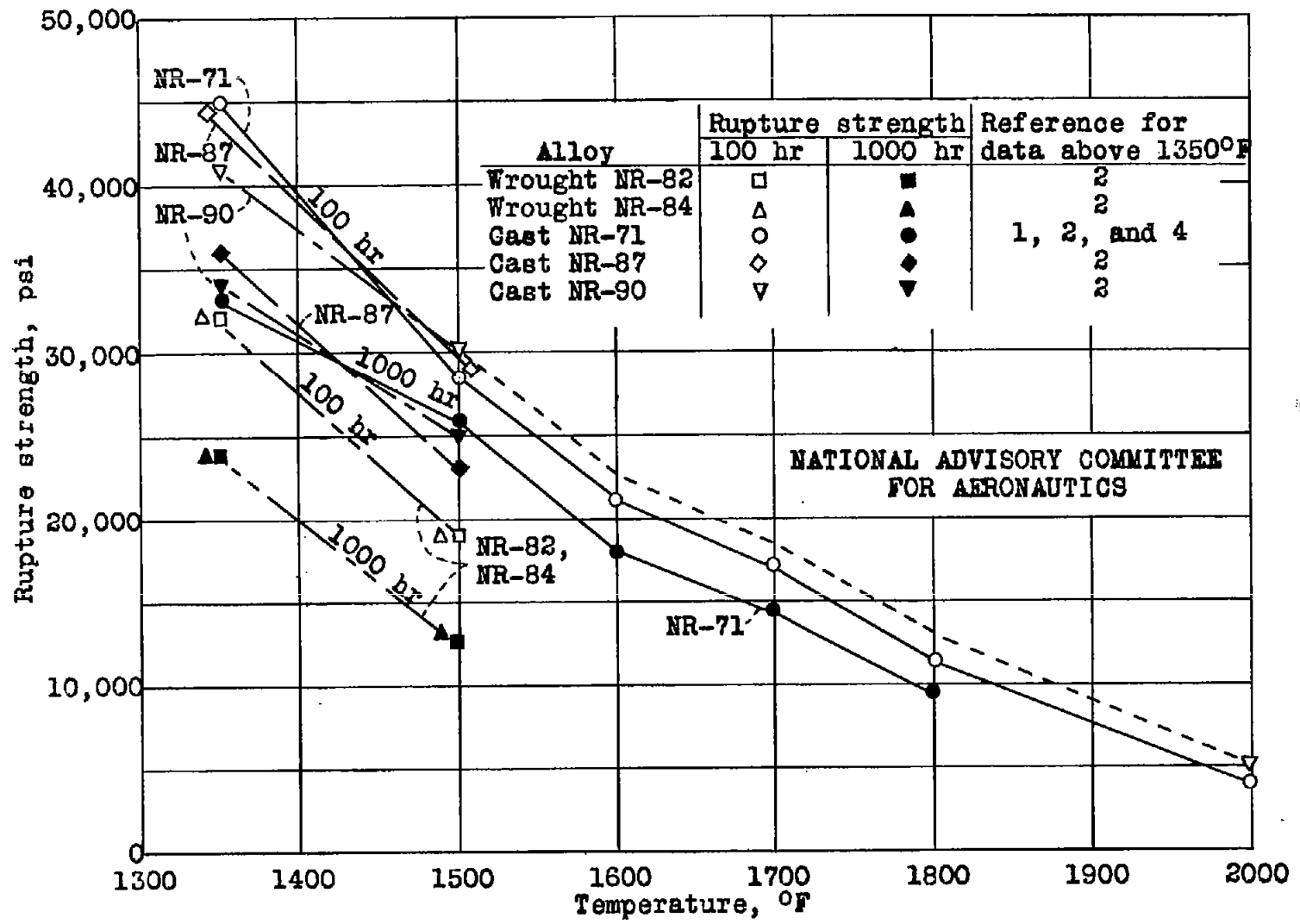
Figure 4.- Variation of rupture strengths with temperature for wrought alloys NR-82 and NR-84 and cast alloys NR-71, NR-87 and NR-90.
