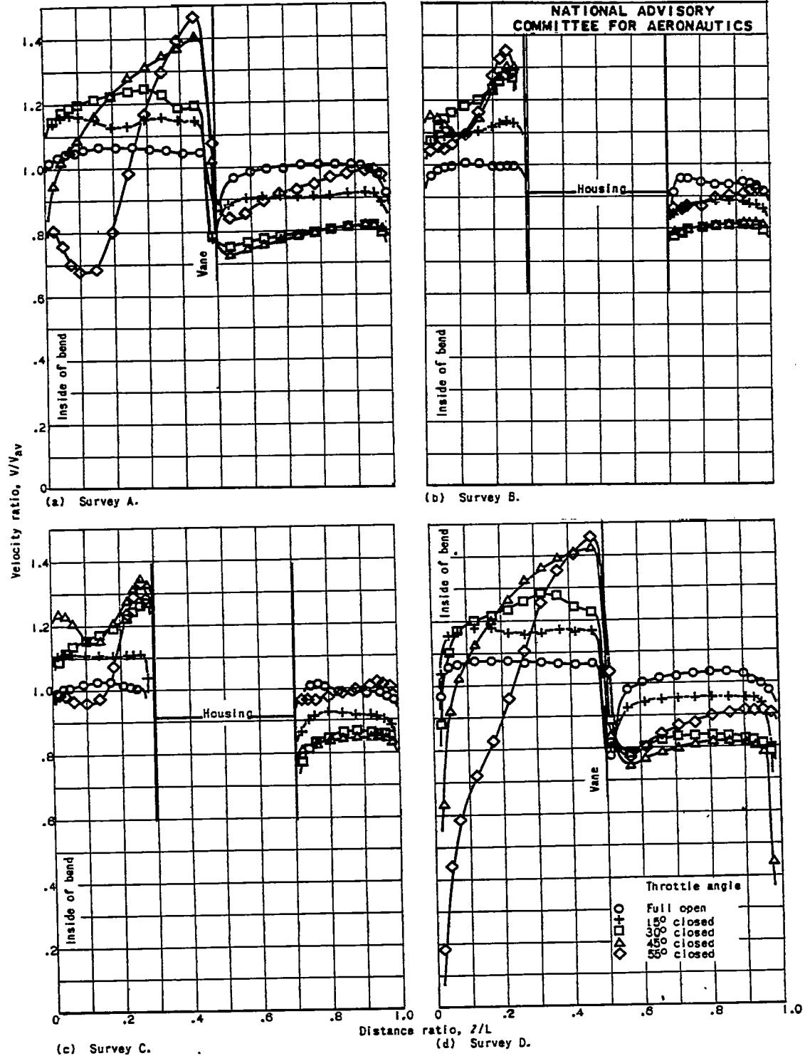
Figure 13. - Effect of carburetor-throttle angle on velocity profile at outlet of elbow with streamlined impeller-shaft housing and vane. Station 3.
