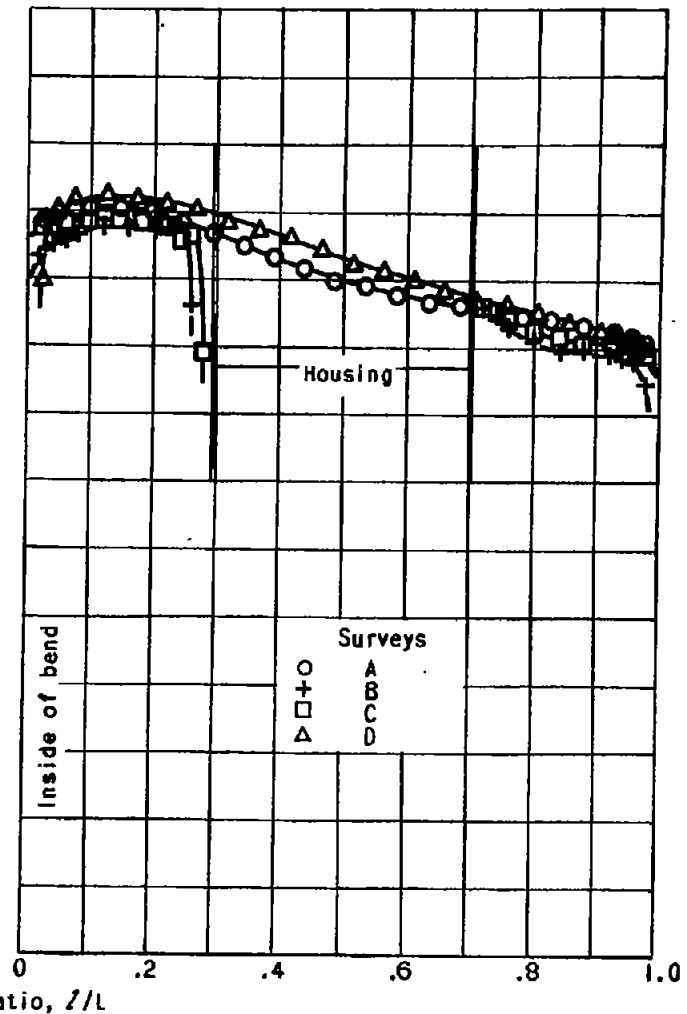
(b) With streamlined impeller-shaft housing.
