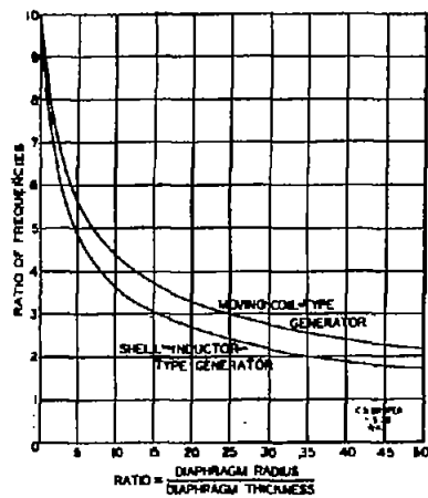
EFFECT OF ATTACHED PARTS ON NATURAL FREQUENCY OF GENERATING SYSTEM, COMPARISON WITH FLAT DIAPHRAGM.
