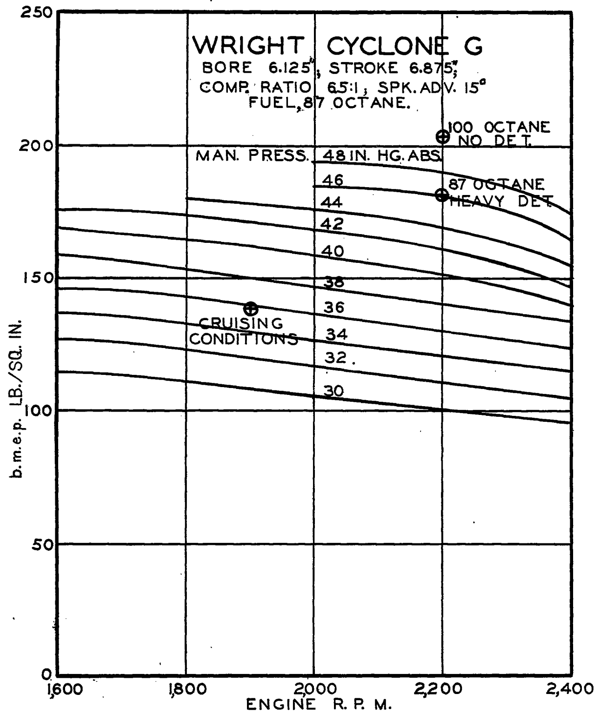
PERFORMANCE CURVES.
