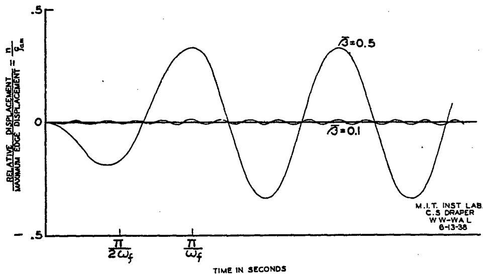
DISPLACEMENT OF DIAPHRAGM CENTER RELATIVE TO ITS EDGES VS. TIME. FIG. 10
