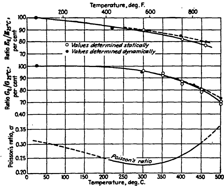
Variation of modulus of elasticity E , modulus of rigidity G , and Poisson's ratio \sigma with temperature, for a medium-carbon steel.
