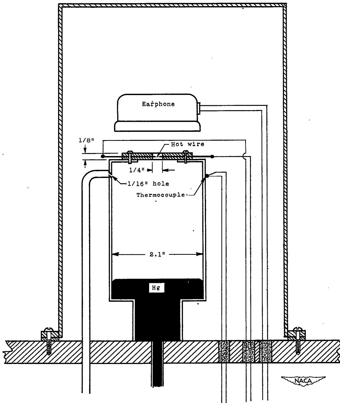
Figure 2.- Helmholtz resonator and chamber.
