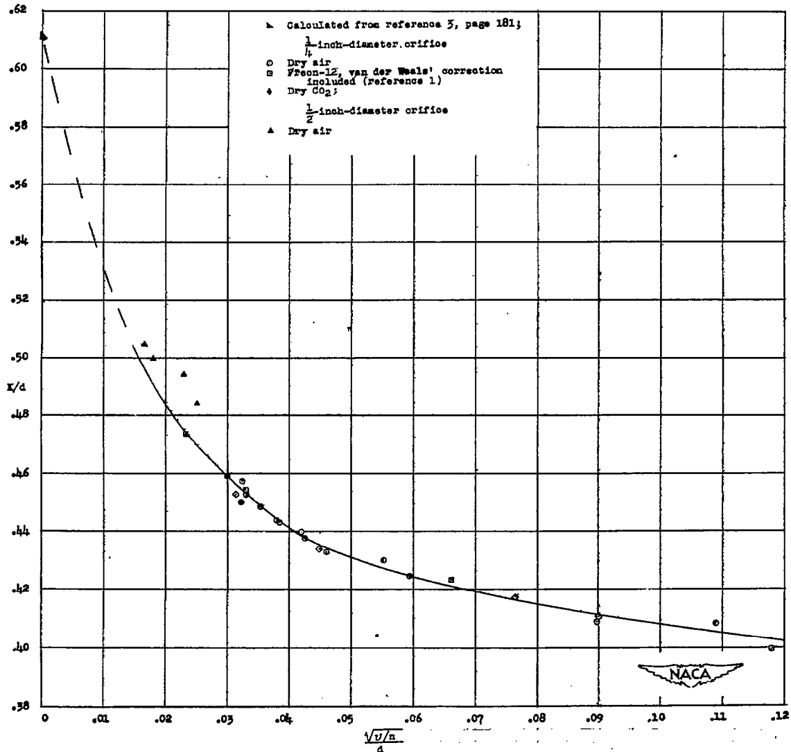
Figure 3.- Effect of the variation of kinematic viscosity and sound frequency in a Helmholtz resonator on the parameter K/d for the resonator orifice. Measurements on each gas were taken over a range of pressures from 0.1 to 1 atmosphere and over a range of frequencies of 200 to 400 cycles per second.
