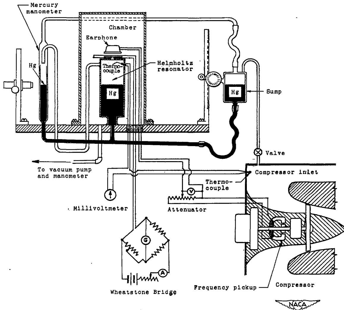
Figure 1.- Schematic arrangement of instrument for measuring sonic velocity and compressor Mach number.
