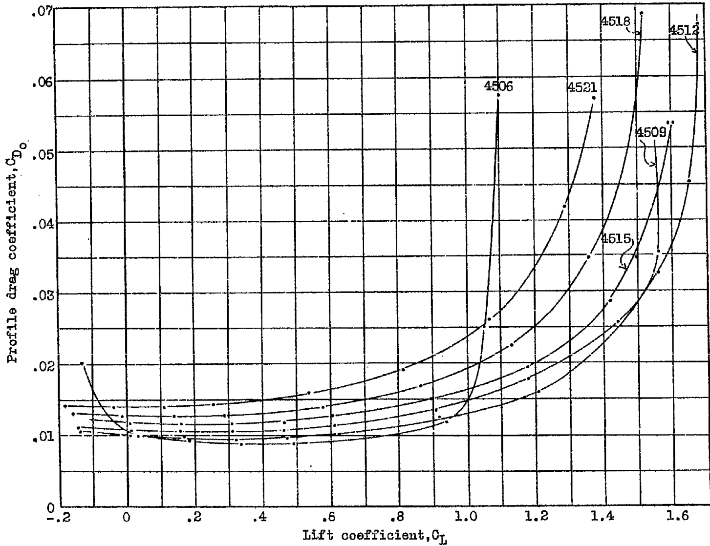
Fig. 2 Profile drag curves for N.A.C.A. 45 series airfoils.
