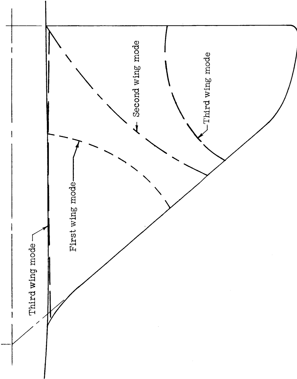
Figure 9.- Wing node lines for the first three wing modes obtained from shake tests.
