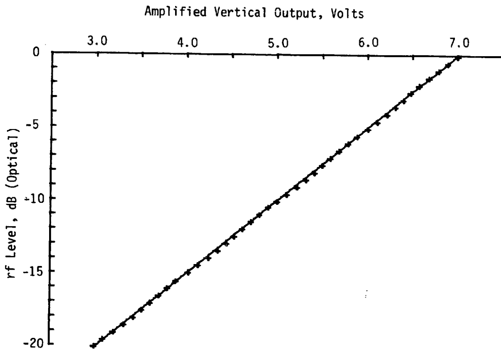
Figure 5-16. Vertical calibration data.
