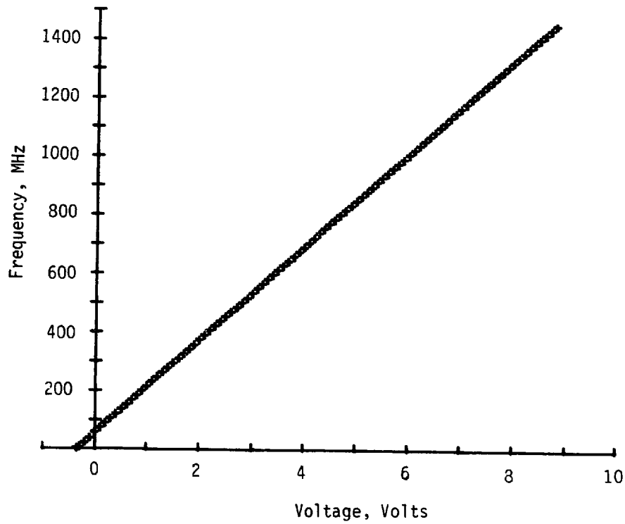
Figure 5-15. Frequency calibration data.
