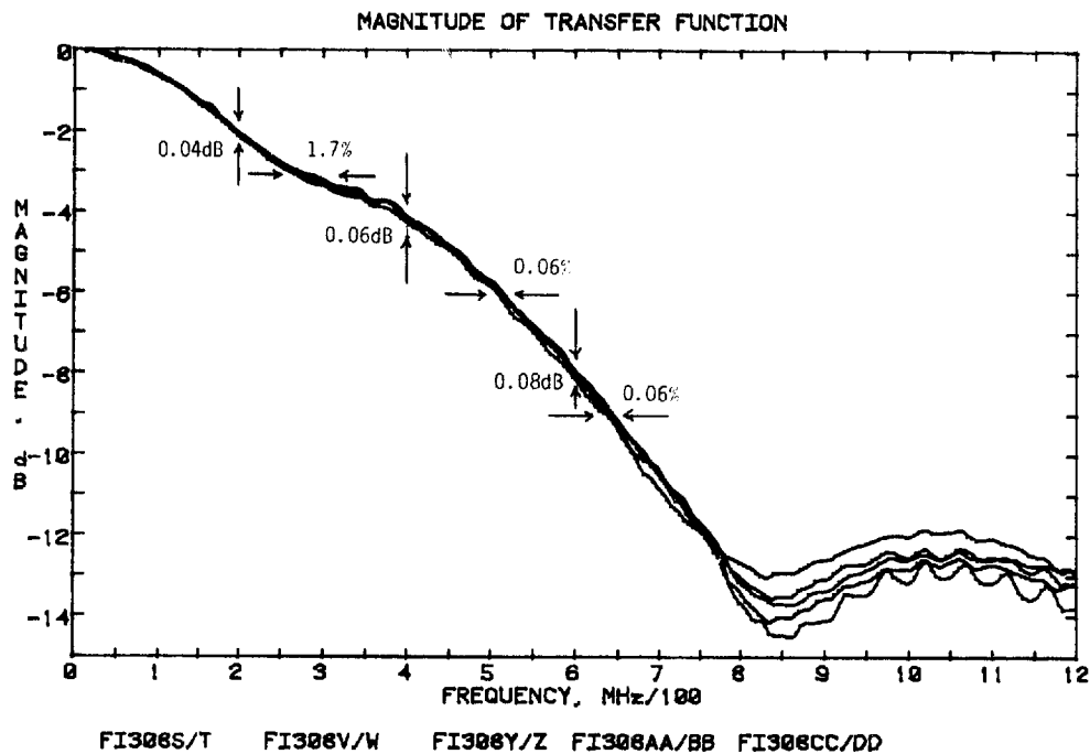
Figure 6-1. Superposition of the results of five independent measurements on fiber I308. Arrows indicate the one standard deviation imprecision at the -3, -6, and -9 dB levels in percent and at frequencies of 200, 400, and 600 MHz in dB.
