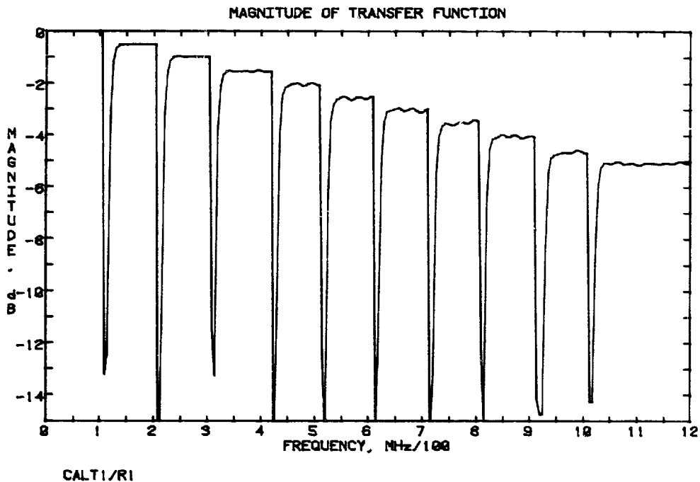
Figure 5-18. Result of replacing test system with a set of precision, step-variable attenuators and switching at intervals during scan.
