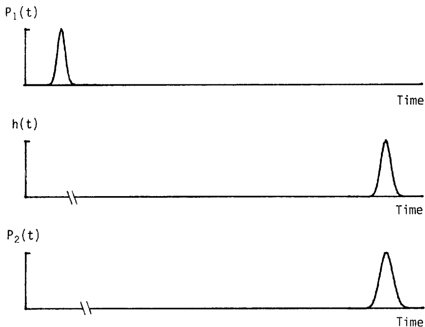
Figure 2-1. The output waveform of a linear system, p_2(t) , can be described as the convolution of the input waveform, P_1(t) and the impulse response, h(t) , of the system. In a transmission medium the impulse response, that is the response to an impulse at t=0 , is characterized by a delay corresponding to the propagation time and distortion.
