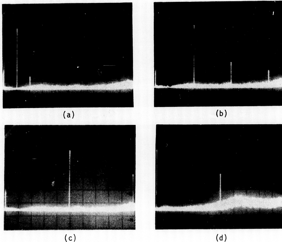
Figure 5-5. Distortion in source output. Drive level was approximately 0 dBm and the vertical scale 10 dB (electrical)/div in each case. (a) Drive: 100 MHz, Scale: 0-1000 MHz; (b) Drive: 300 MHz, Scale: 0-1000 MHz; (c) Drive: 500 MHz, Scale: 0-1000 MHz; (d) Drive: 500 MHz, Scale: 500-1000 MHz.
