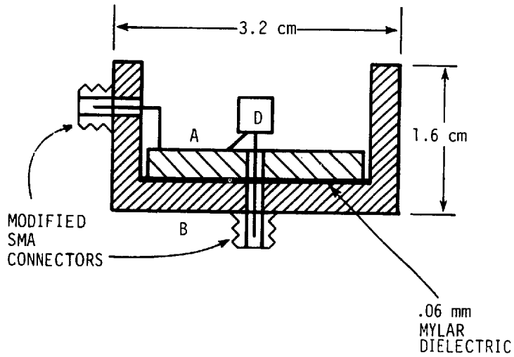
Figure 5-11. Diagram of detector mount.
