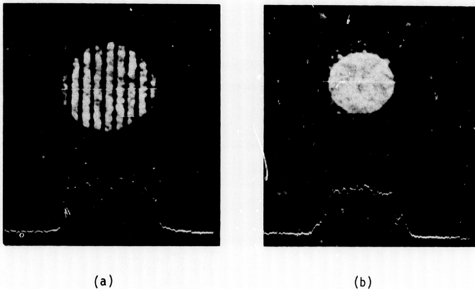
Figure 5-8. (a) Image of stage micrometer placed where specimen input would normally be placed, to verify size of launch spot. Line spacing is 10 \mu\text{m} . (b) Image of short step-index specimen. The core appears brighter because of reflected light from output end of fiber.
