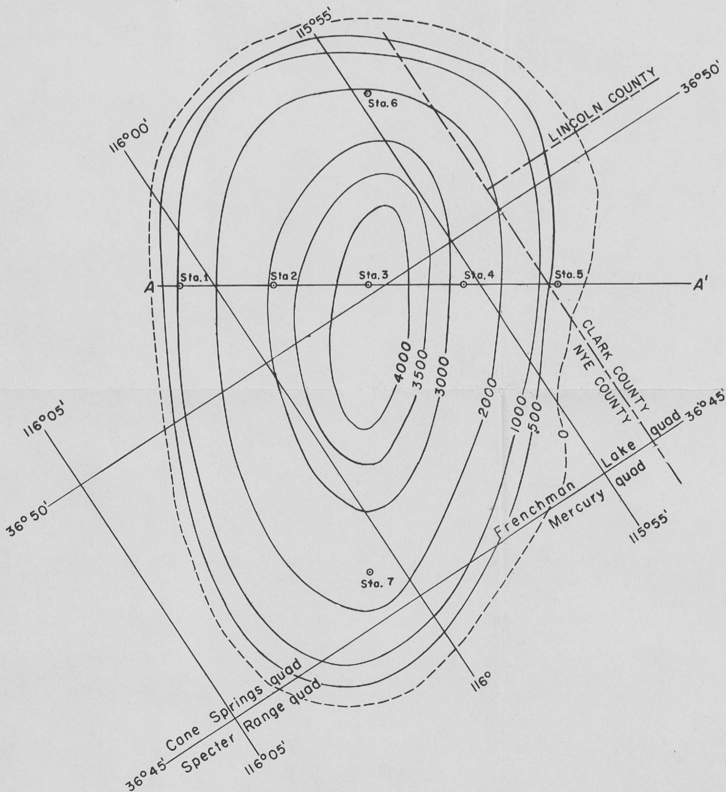
FIGURE 6 - A PRELIMINARY THREE-DIMENSIONAL INTERPRETATION OF GRAVITY DATA, FRENCHMAN VALLEY, NYE, LINCOLN, AND CLARK COUNTIES, NEVADA
