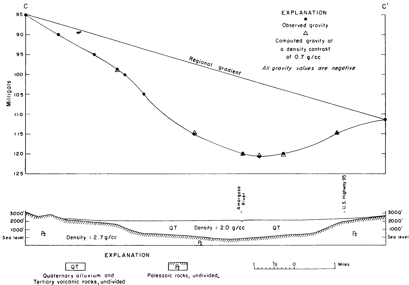
Figure 8.--A two-dimensional graticule analysis of gravity data across the Amargosa Desert, Nye County, Nev. Line of section shown on figure 5.
