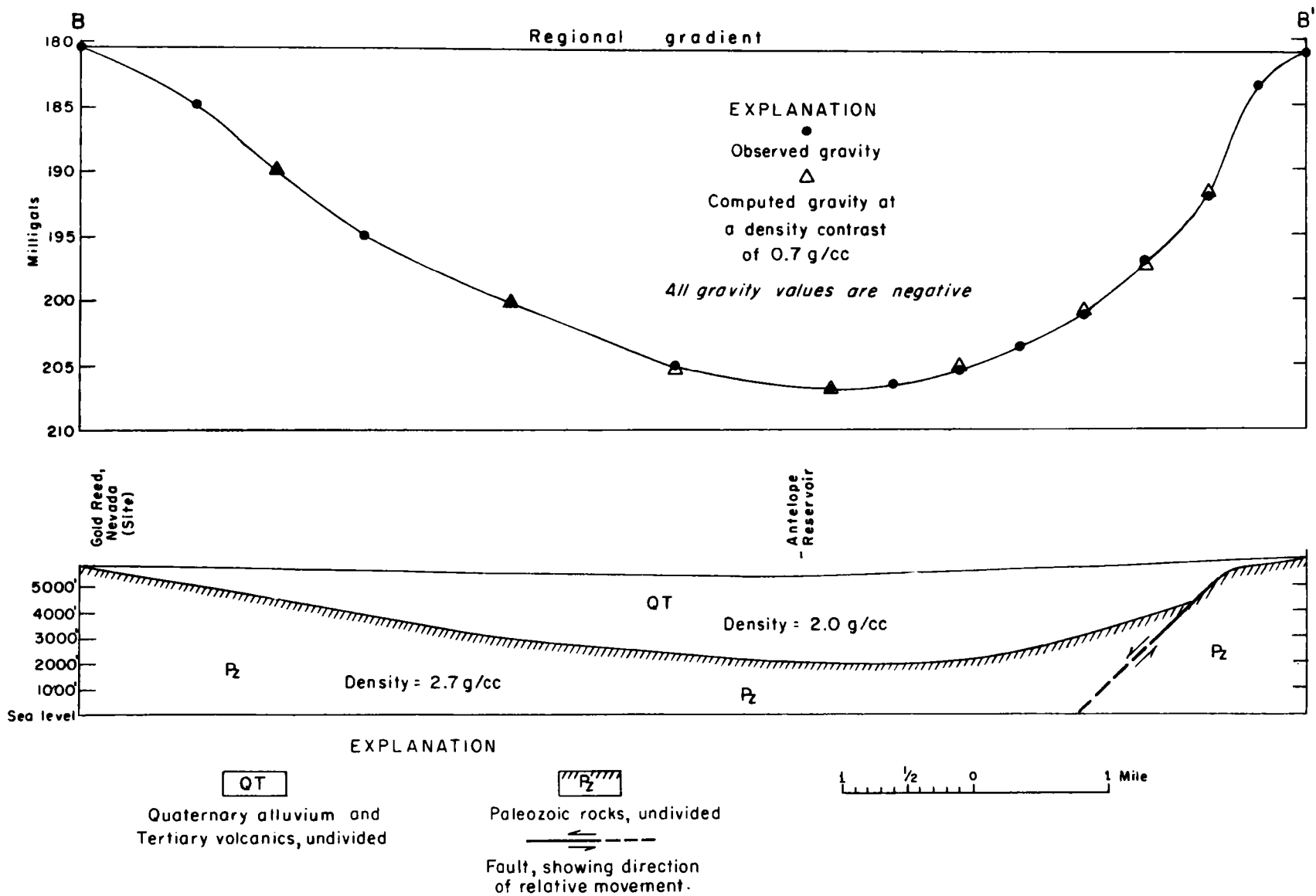
Figure 7.--A two-dimensional graticule analysis of gravity data across Kawich Valley, Nye County, Nev. Line of section shown on figure 5.
