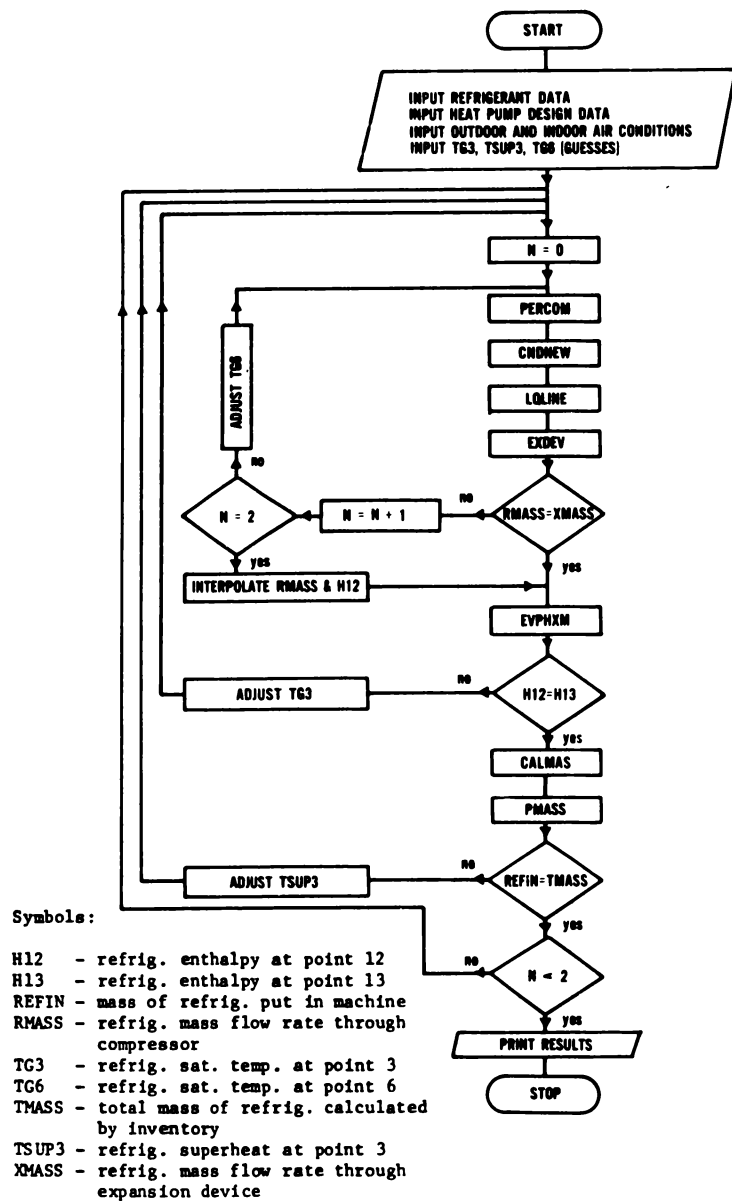
Figure H1. Heat pump simulation program HPSIM flow chart
