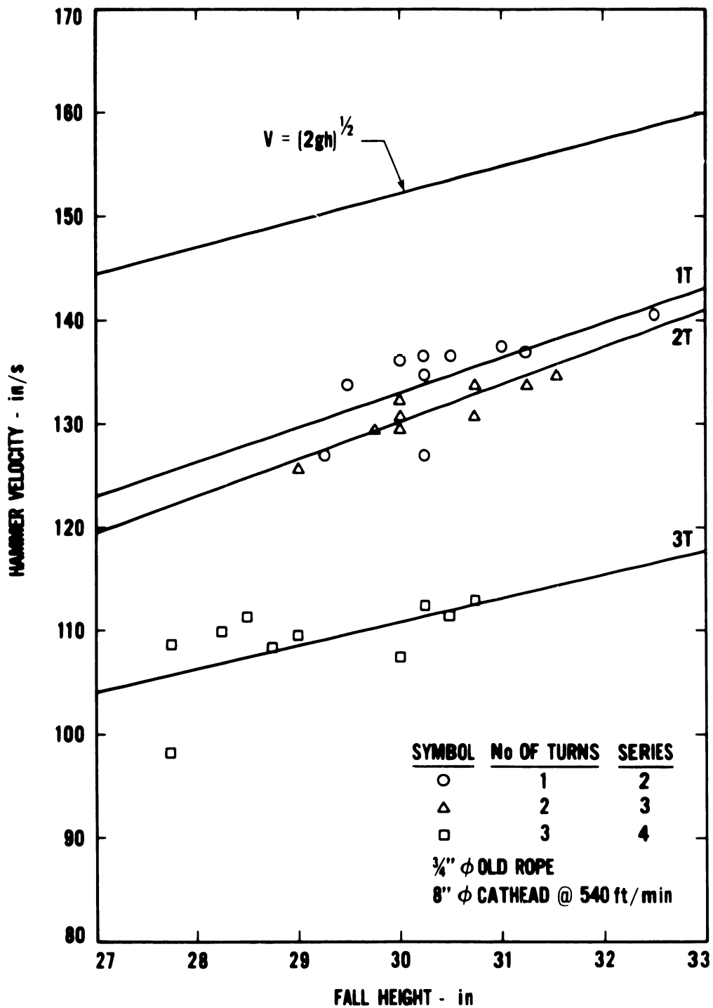
Figure 3-2. Hammer velocity just before impact versus fall height for Series 2, 3, and 4 data (least squares fit of data in table A-1).
