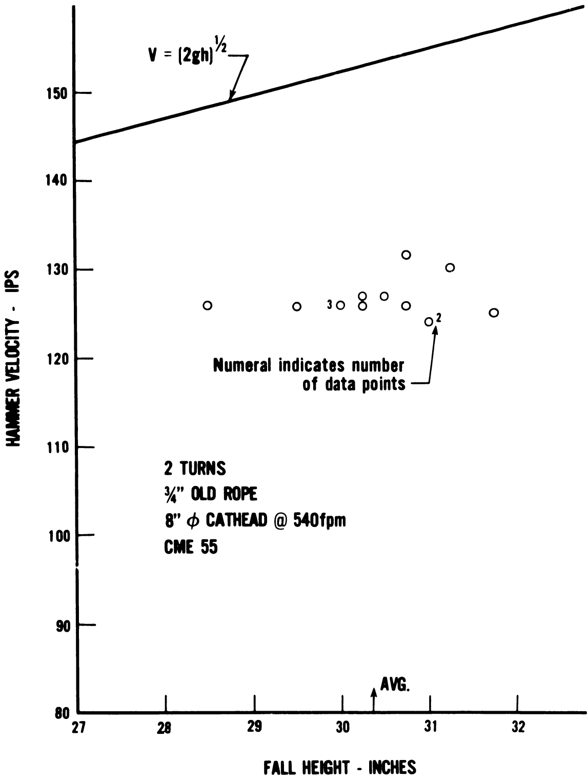
Figure 3-1. Hammer velocity just before impact versus fall height for Series 1 data.
