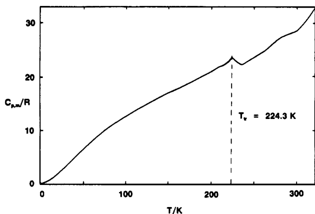
Figure 1. Temperature dependence of C_{p,m}/R of 2,4,6-trimethylbenzointrile N -oxide. The vertical line indicates the temperature of the phase transition. The solid curve represents the "smoothed" heat capacity data.
