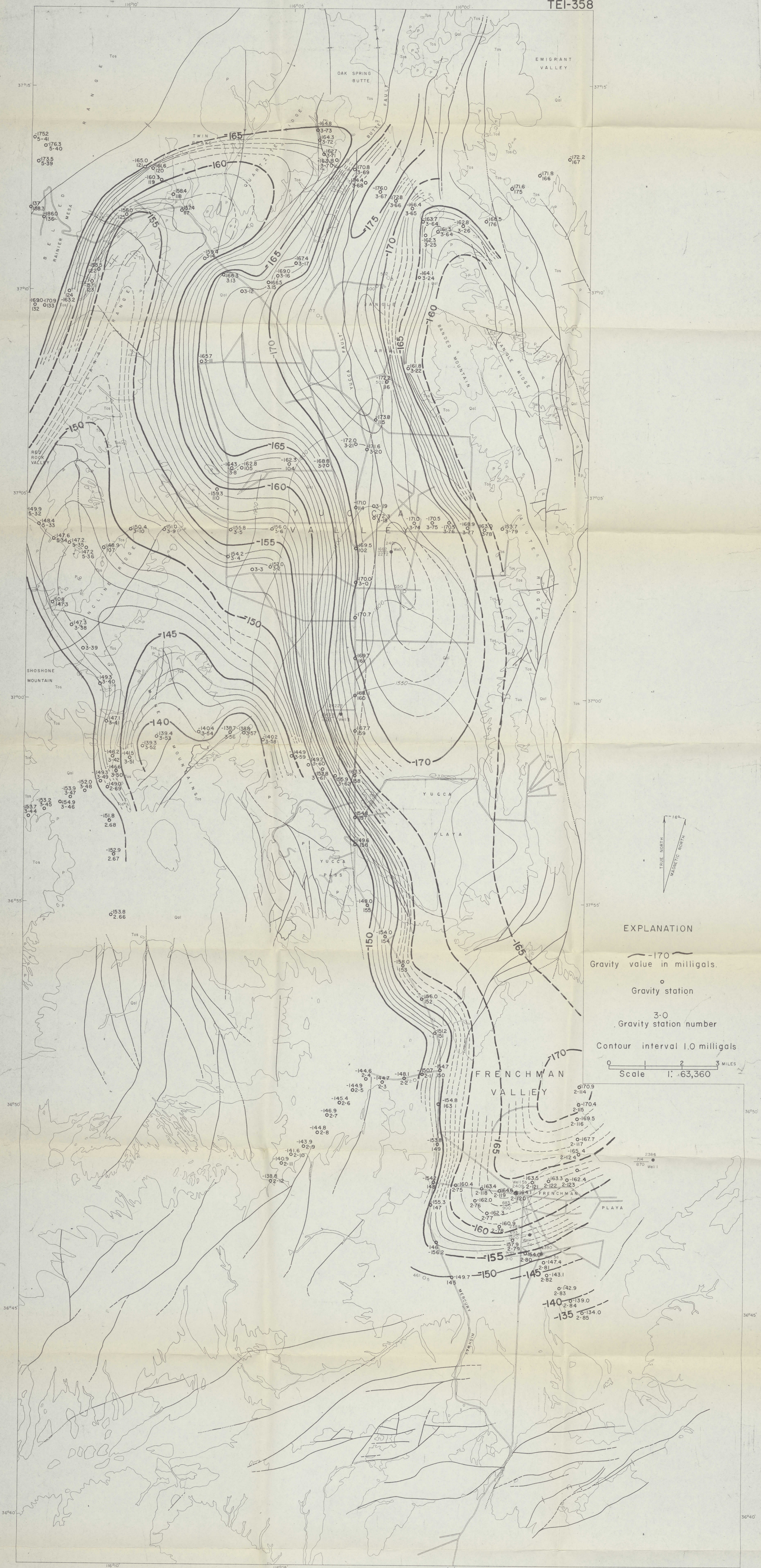
FIGURE 2. BOUGUER GRAVITY MAP OF YUCCA AND FRENCHMAN VALLEYS, NEVADA TEST SITE, NYE AND CLARK COUNTIES, NEVADA
