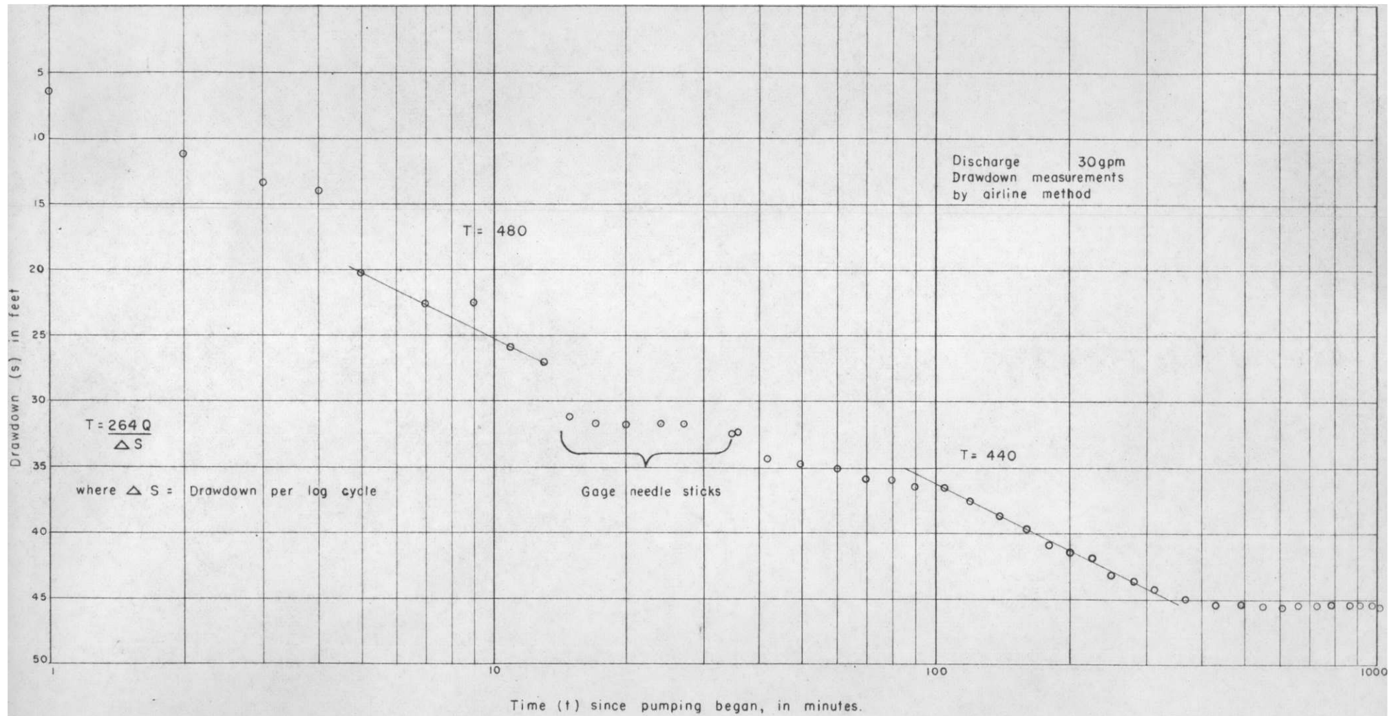
FIGURE 4 — DRAWDOWN DURING PUMPING OF WELL 3 (December 1 and 2, 1958)
