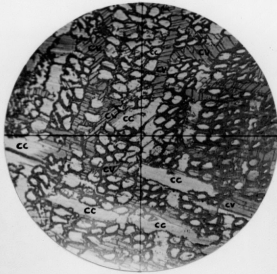
Figure 3A. --Photomicrograph of a part of a copper sulfide nodule showing plant cell structure. Chalcocite (cc), covellite (cv). Cell walls are composed of vitrain. X 132.
