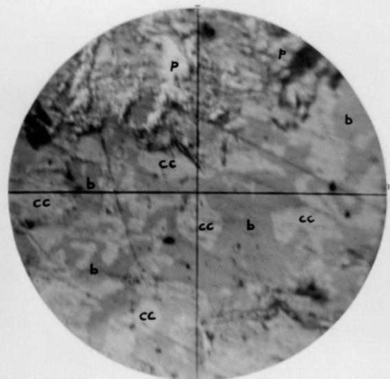
Figure 3C. --Graphic association of bornite (b) and chalcocite (cc) in a copper sulfide nodule. Pyrite (p) is present in upper part of photomicrograph. X 380.
