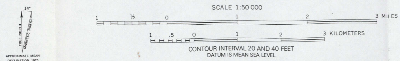
MINERAL RESOURCE POTENTIAL AND GEOLOGIC MAP OF THE OREGON BUTTES WILDERNESS STUDY AREA, SWEETWATER COUNTY, WYOMING
