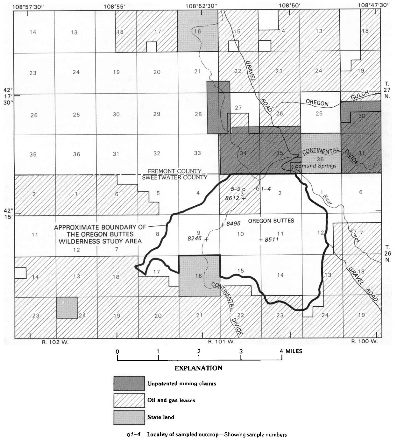
Figure 3. Mining claims, oil and gas leases, and sample localities in the Oregon Buttes Wilderness Study Area.
