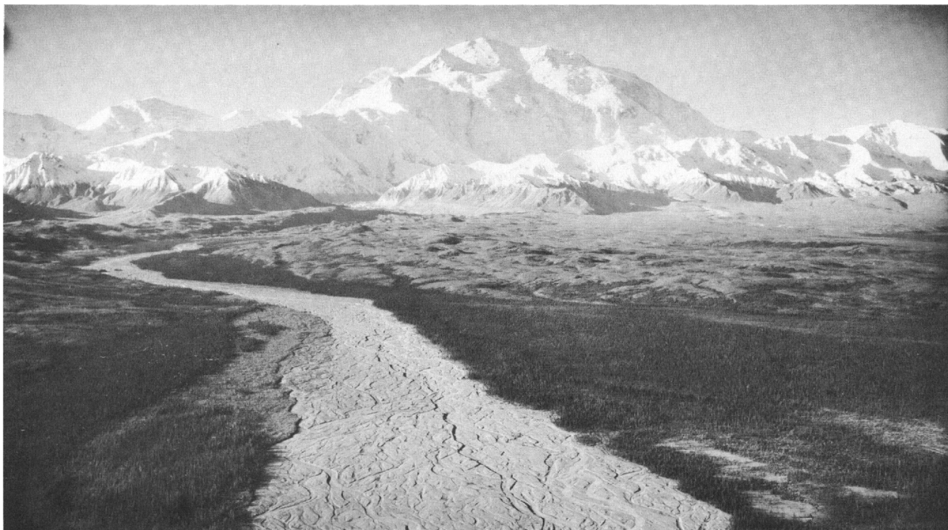
FIGURE 4.—View south up the Muddy River to Peters Glacier and Mount McKinley. The Denali fault lies in the trench between the low mountains and Mount McKinley. Muddy River in the foreground is a typical braided stream flowing on an outwash plain between morainal hills. Photograph by Bradford Washburn, August 15, 1949.
