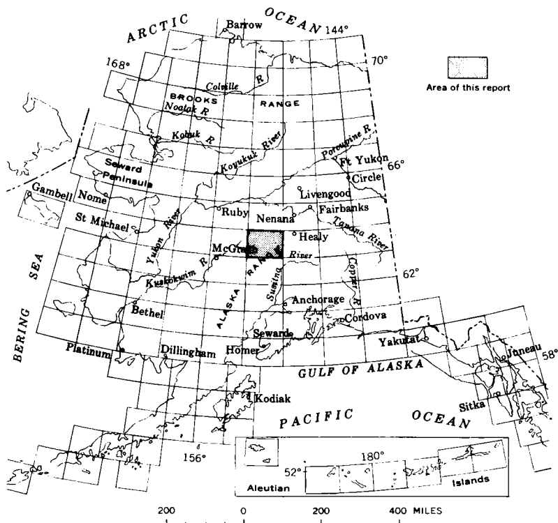
FIGURE 1.—Index map of part of Alaska, showing location of the Mount McKinley quadrangle.
