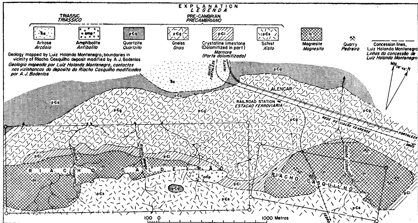
FIGURE 8.—Geologic map of the magnesite deposits at Alencar, Ceará.
