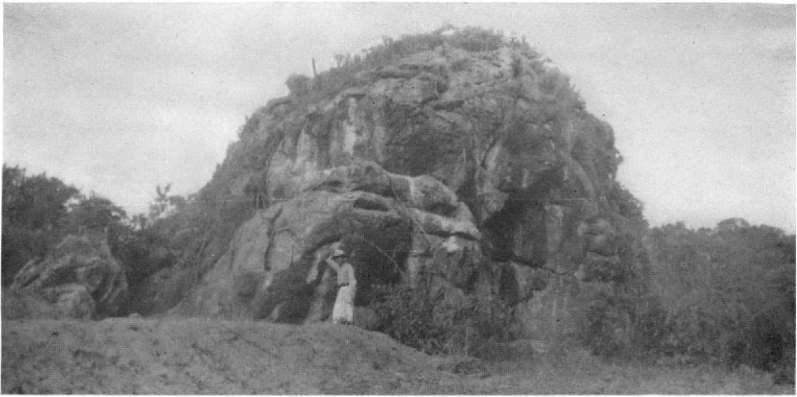
A. LARGE MAGNESITE OUTCROP AT THE RIACHO FUNDO DEPOSIT.
