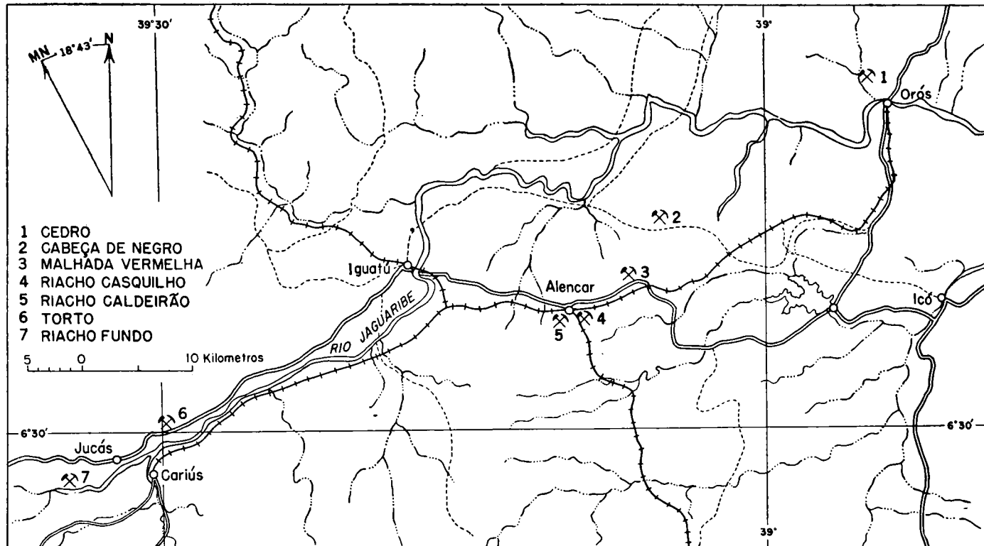
FIGURE 7.—Index map of central Ceará, showing locations of the magnesite deposits.
