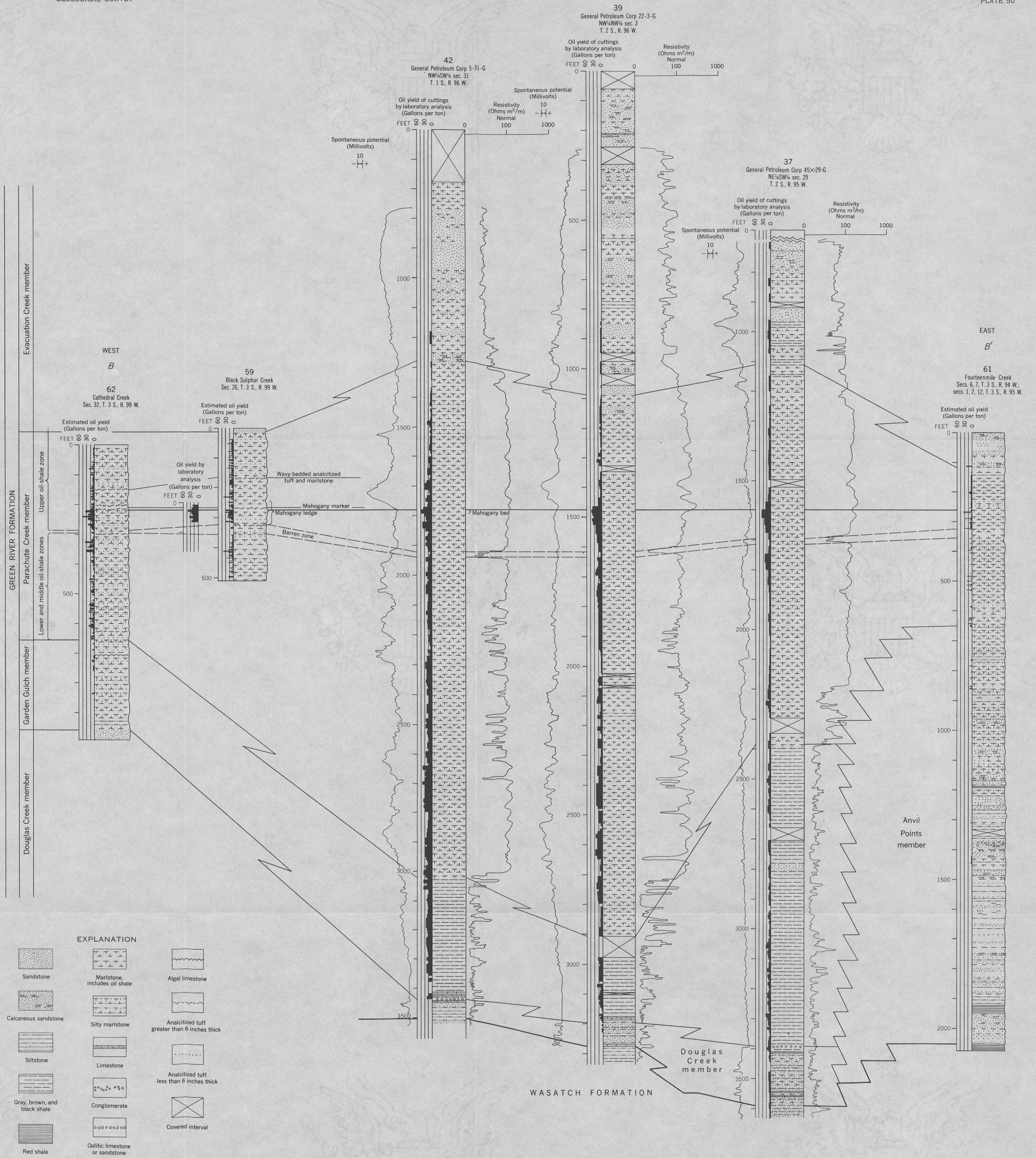
COLUMNAR SECTIONS ALONG LINE B-B', CENTRAL PART OF THE PICEANCE CREEK BASIN, COLORADO
