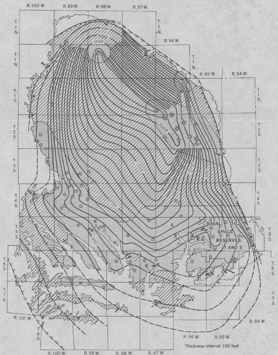
D. MAP SHOWING THE THICKNESS OF OIL SHALE THAT YIELDS AN AVERAGE OF 15 GALLONS OF OIL PER TON
