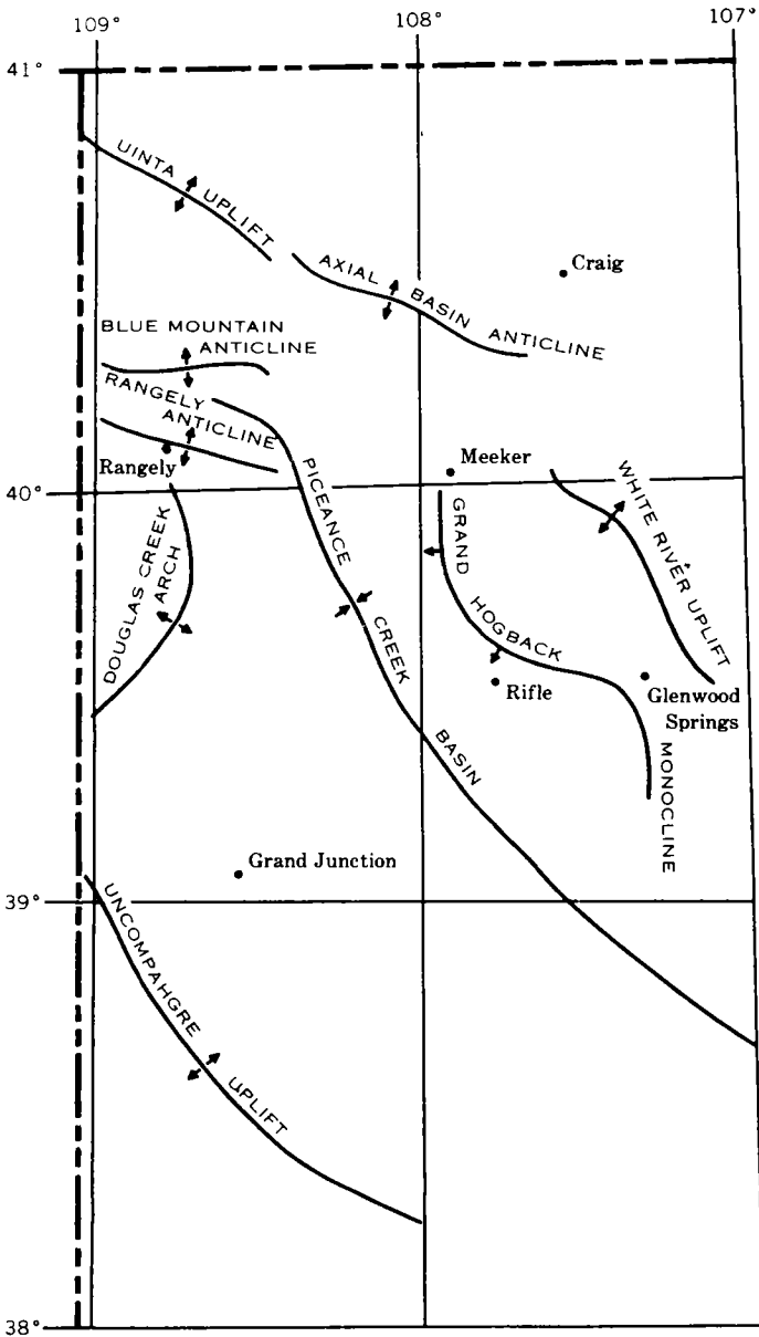
FIGURE 73.—Structural features in northwestern Colorado.
