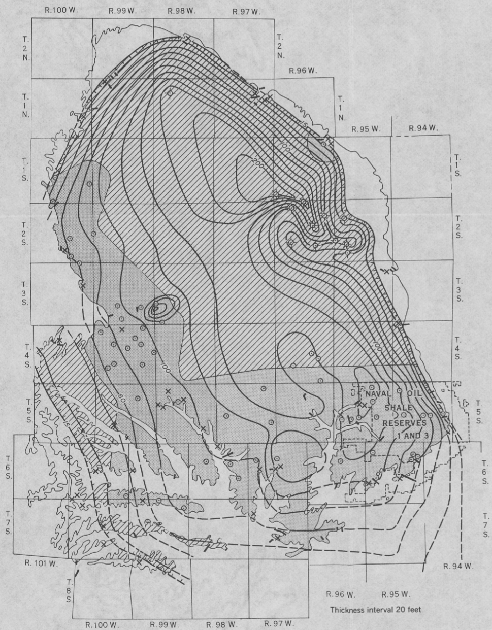
C. MAP SHOWING THE THICKNESS OF SHALE IN AND ADJACENT TO THE MAHOGANY ZONE THAT YIELDS AN AVERAGE OF 25 GALLONS OF OIL PER TON
