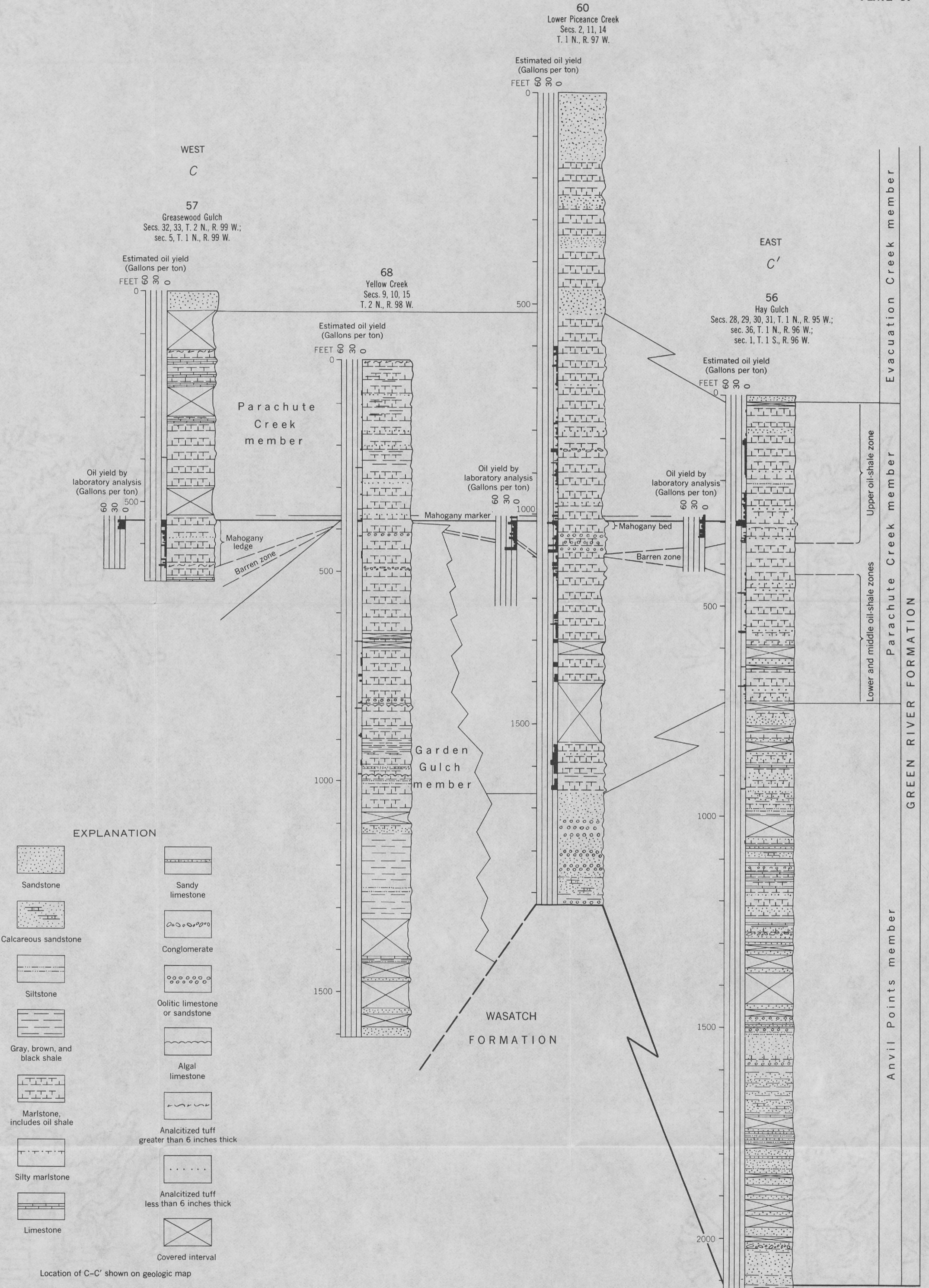
COLUMNAR SECTIONS ALONG LINE C-C' NORTH MARGIN OF THE PICEANCE CREEK BASIN, COLORADO
