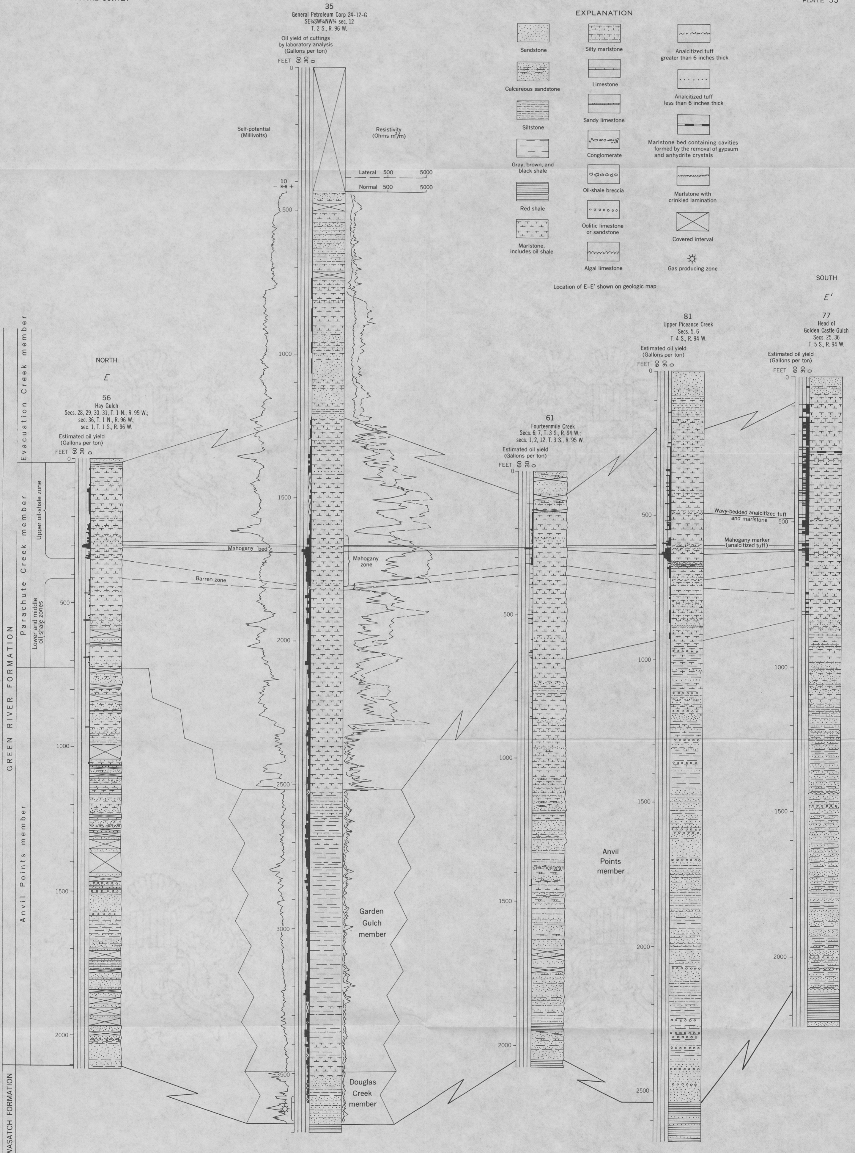
COLUMNAR SECTIONS ALONG LINE E-E', EAST MARGIN OF THE PICEANCE CREEK BASIN, COLORADO
