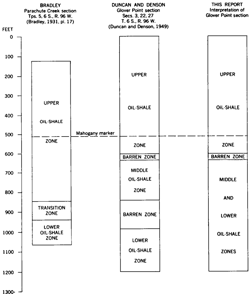
FIGURE 72.—Terminology of oil-shale zones, Piceance Creek basin, as used in this and in previous reports.
