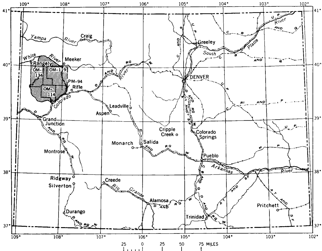
FIGURE 71.—Index map of Colorado showing location of mapped area.
