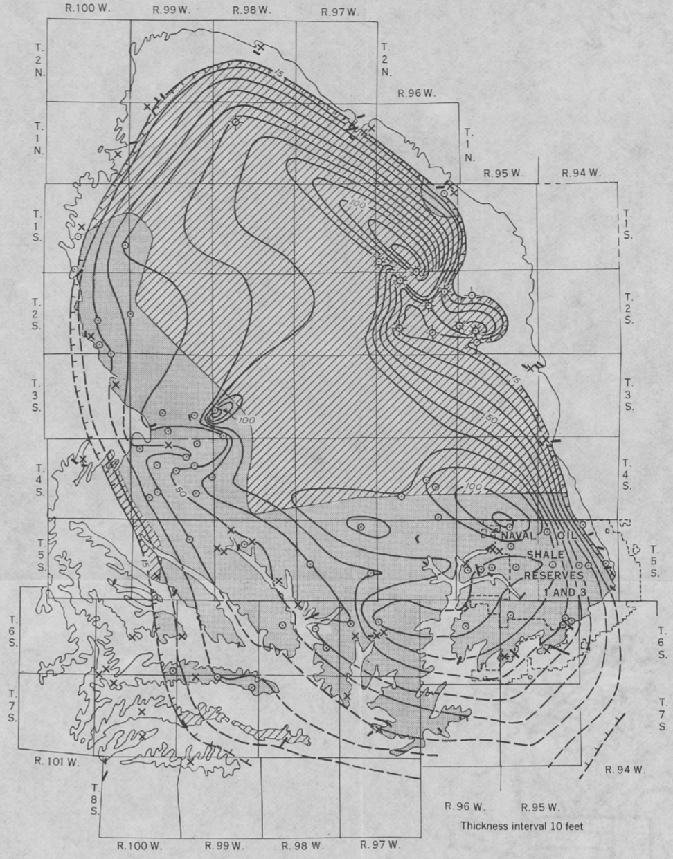
B. MAP SHOWING THE THICKNESS OF SHALE IN AND ADJACENT TO THE MAHOGANY ZONE THAT YIELDS AN AVERAGE OF 30 GALLONS OF OIL PER TON
