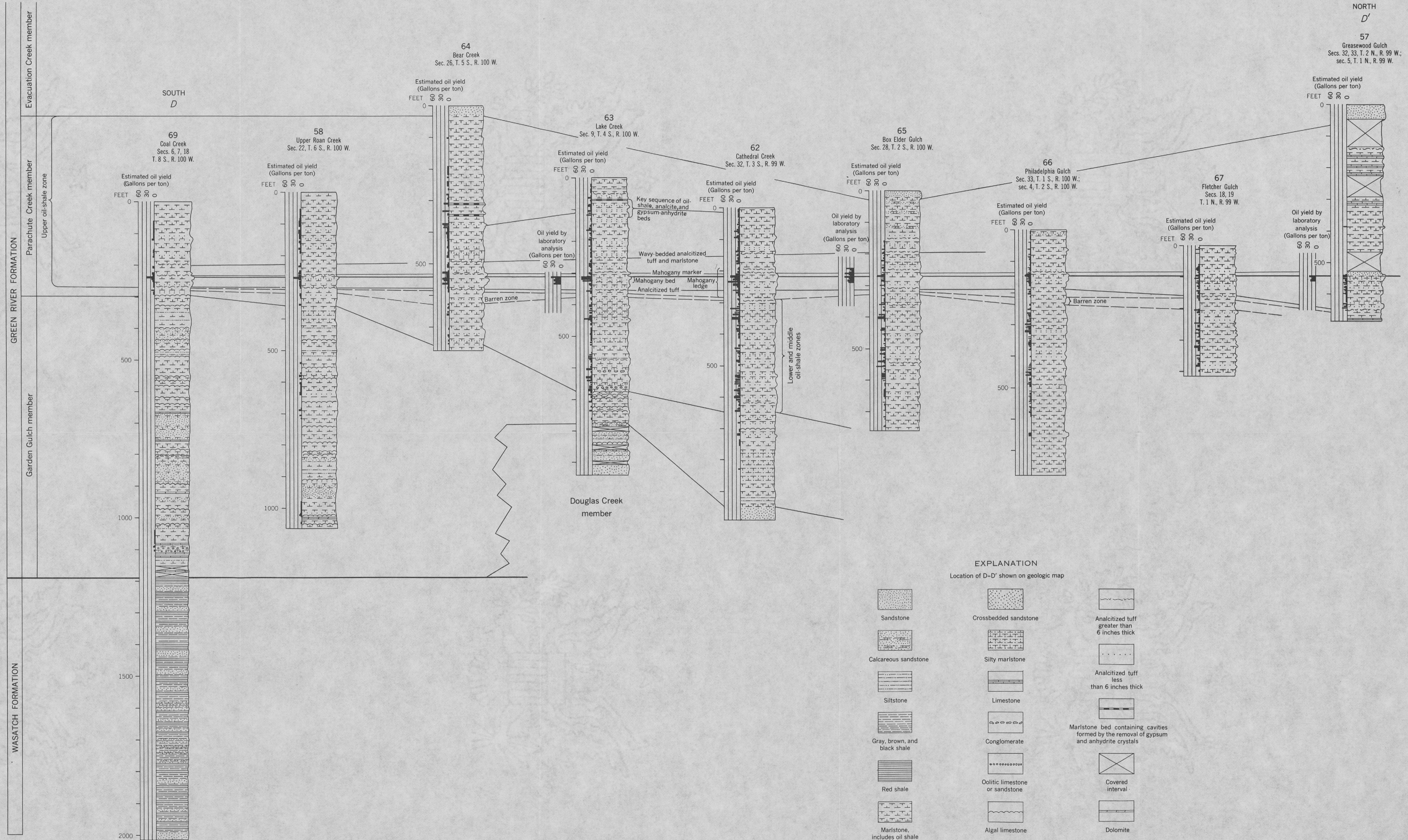
COLUMNAR SECTIONS ALONG LINE D-D', WEST MARGIN OF THE PICEANCE CREEK BASIN, COLORADO
