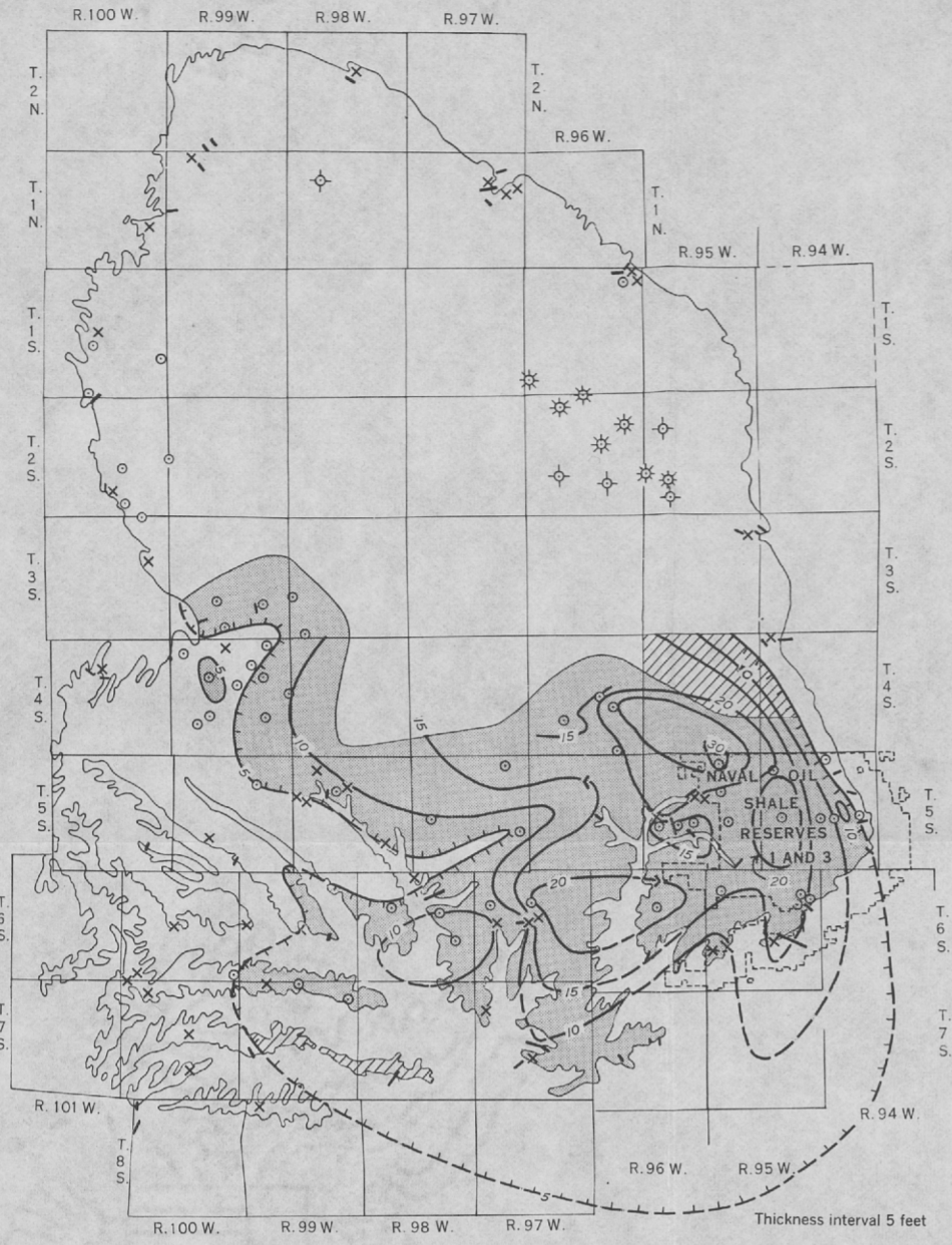
A. MAP SHOWING THE THICKNESS OF THE PART OF THE MAHOGANY ZONE THAT YIELDS AN AVERAGE OF 45 GALLONS OF OIL PER TON
