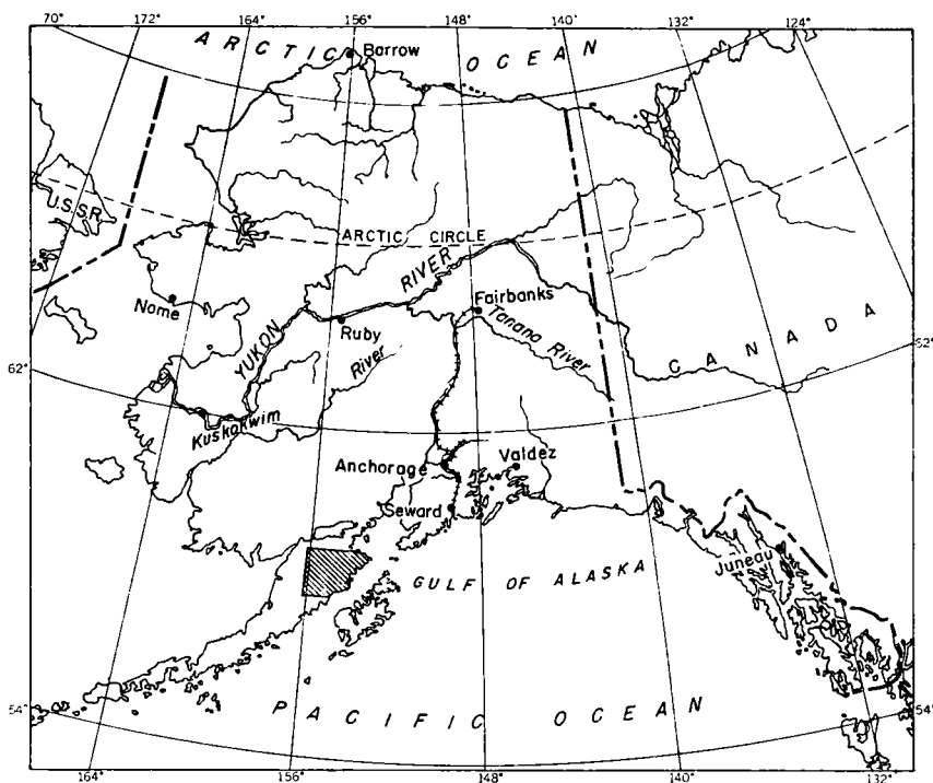
FIGURE 44.—Index map of Alaska, showing location of Mount Katmai area (shaded).
