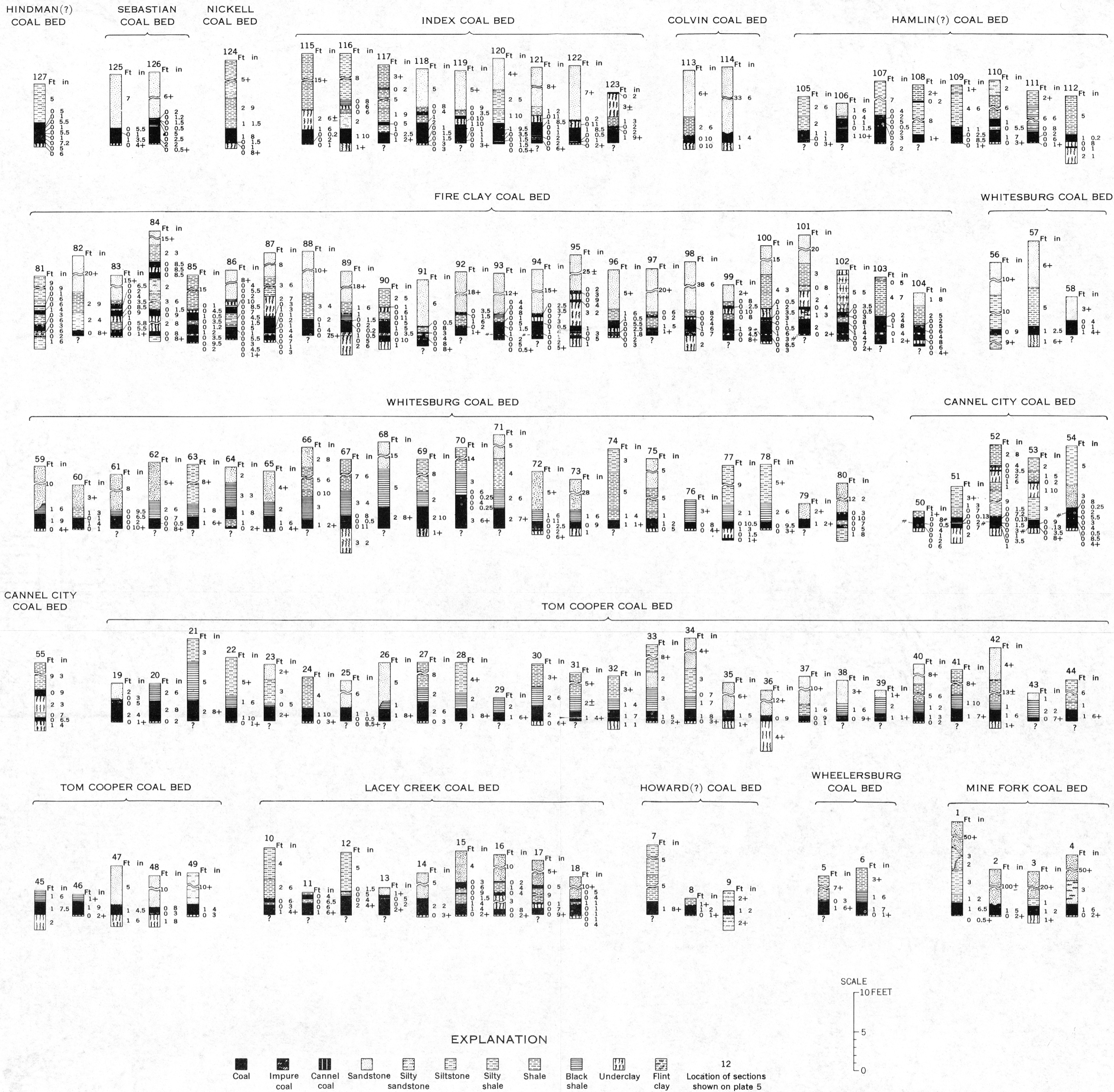
SECTIONS OF COAL BEDS EXPOSED IN THE SALYERSVILLE NORTH QUADRANGLE, MAGOFFIN MORGAN, AND JOHNSON COUNTIES, KENTUCKY
