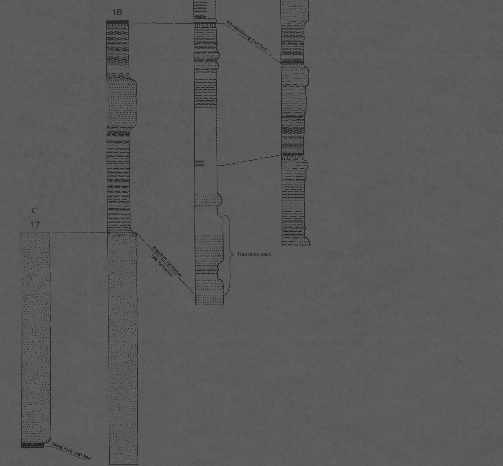
STRATIGRAPHIC SECTIONS OF THE LEE AND BREATHTITT FORMATIONS IN THE SALYERSVILLE NORTH QUADRANGLE, KENTUCKY
