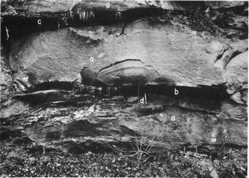
FIGURE 12.—Exposure of strata 18 feet below the Fire Clay coal bed (pl. 6, basal part of section 2) about 0.15 mile southwest of the mouth of Wesley Fork showing (a) massive sandstone, (b) coal lens 8 inches thick, (c) gray silty shale wedge, and (d) hammer and steel tape.
