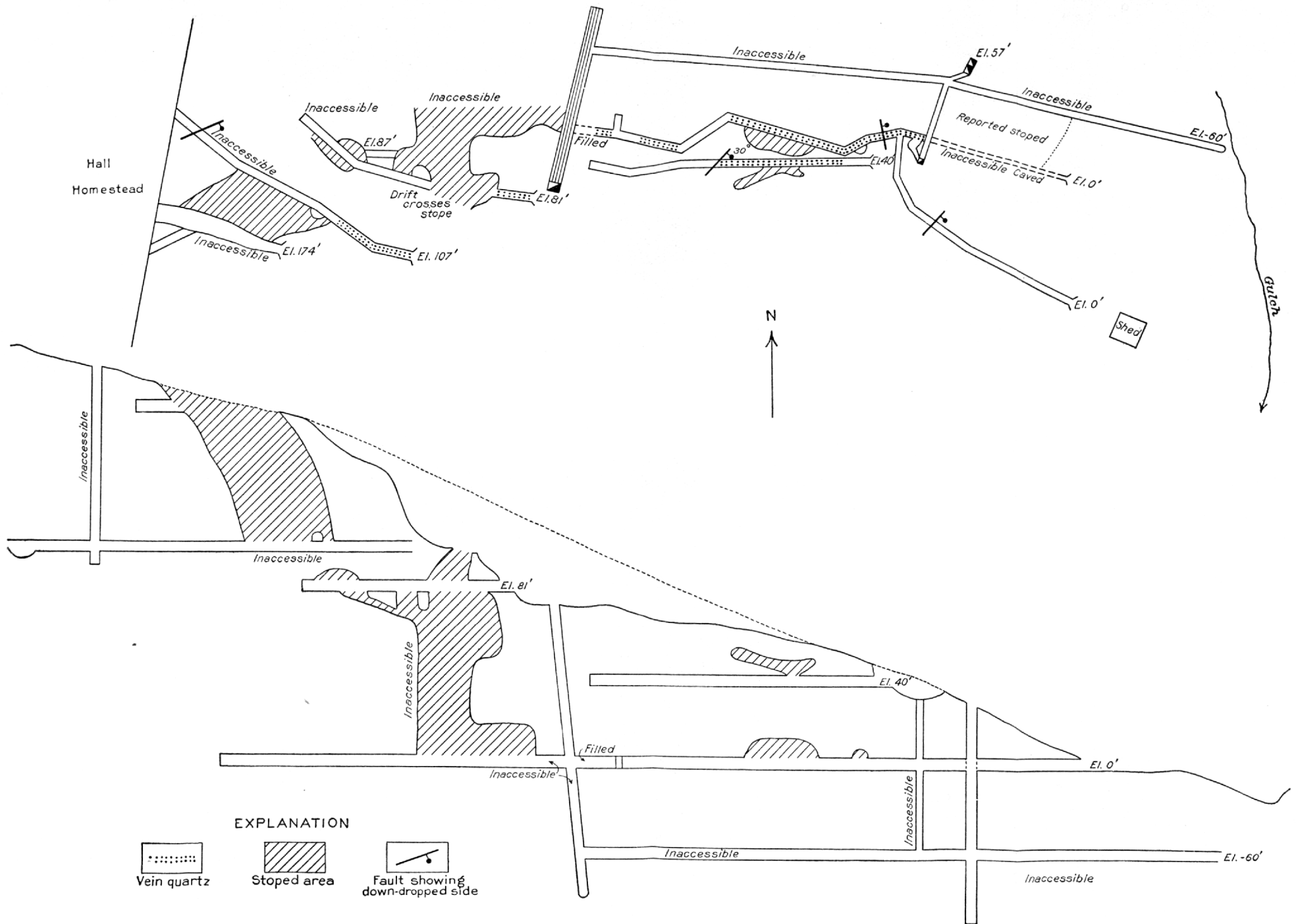
MAP OF CONTINENTAL MINE, DOUGLAS COUNTY, OREG.
