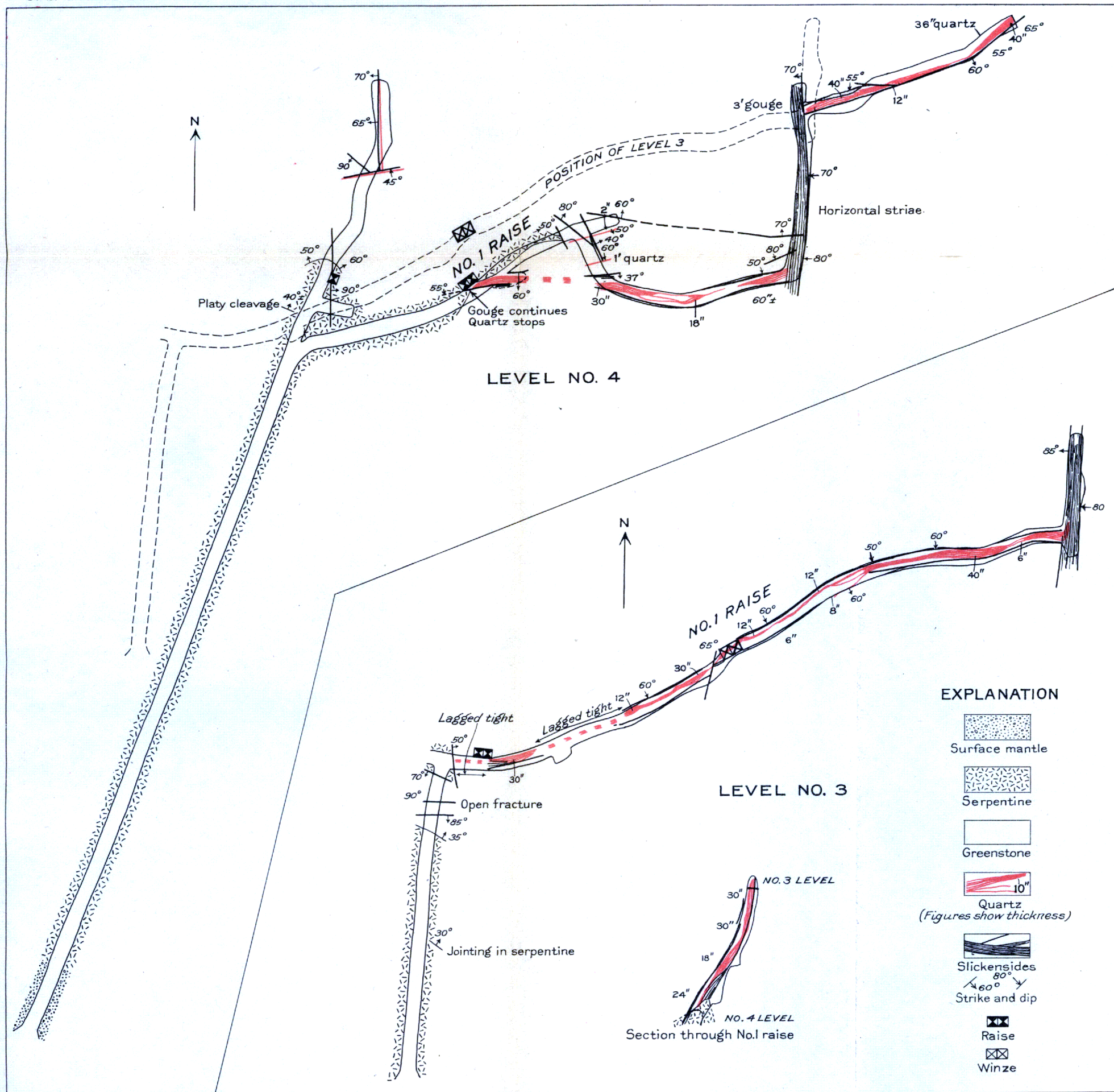
PLAN OF LEVELS 3 AND 4 AND SECTION THROUGH No. 1 RAISE ROBERT E. MINE, CURRY COUNTY, OREGON
