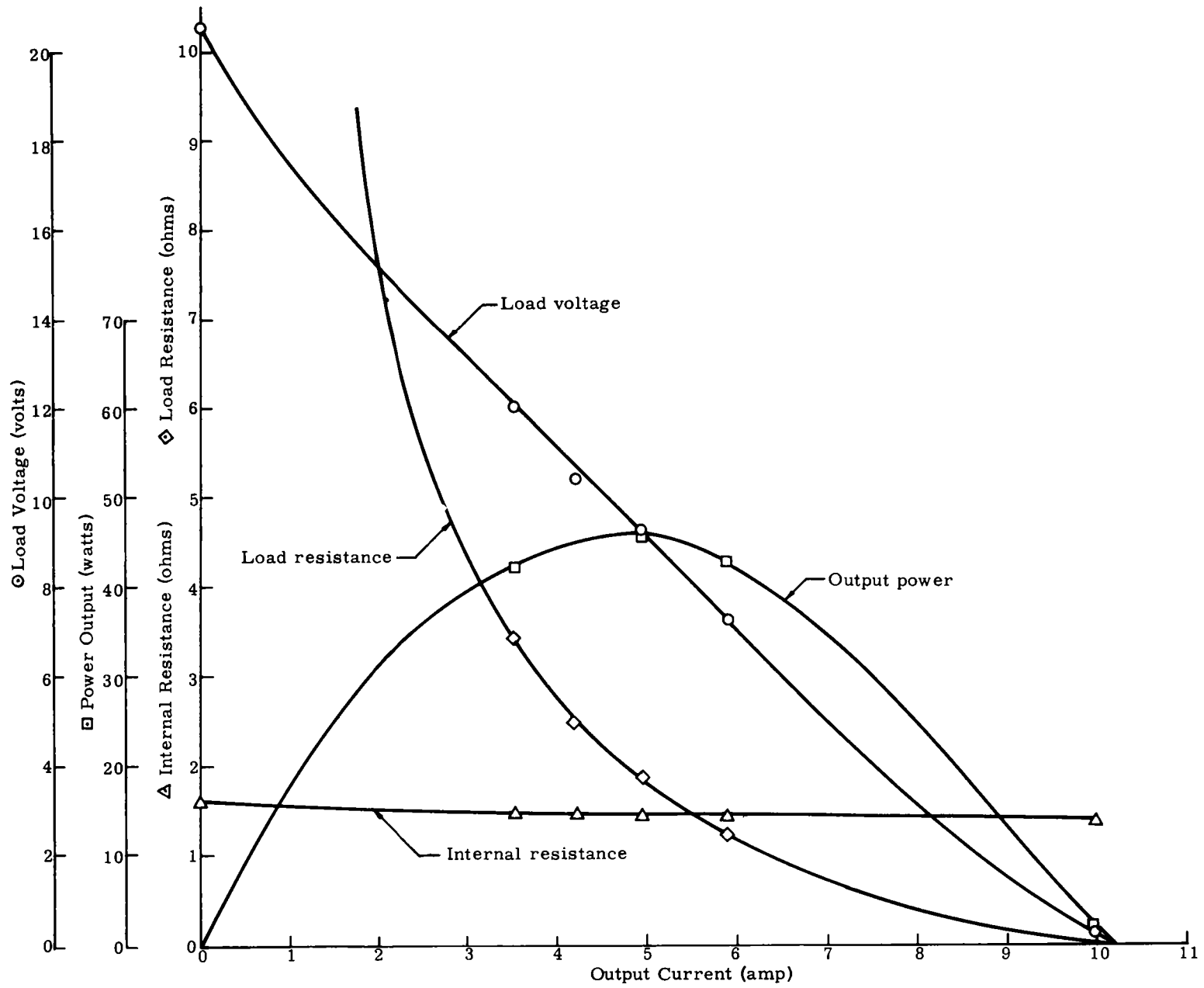
Fig. 8. SNAP 7D 60-Watt Generator--Parametric Data at End of Life (electrical power input: 1080 watts; internal gas: pure argon)
