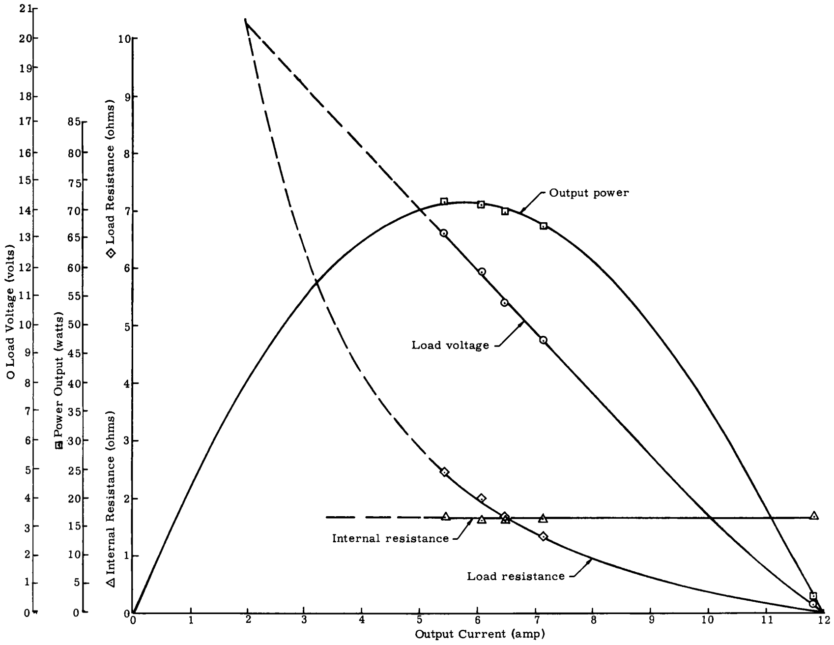
Fig. 6. SNAP 7D 60-Watt Generator--Parametric Data at Start of Life (electrical power input: 1480 watts; internal gas: pure helium)
