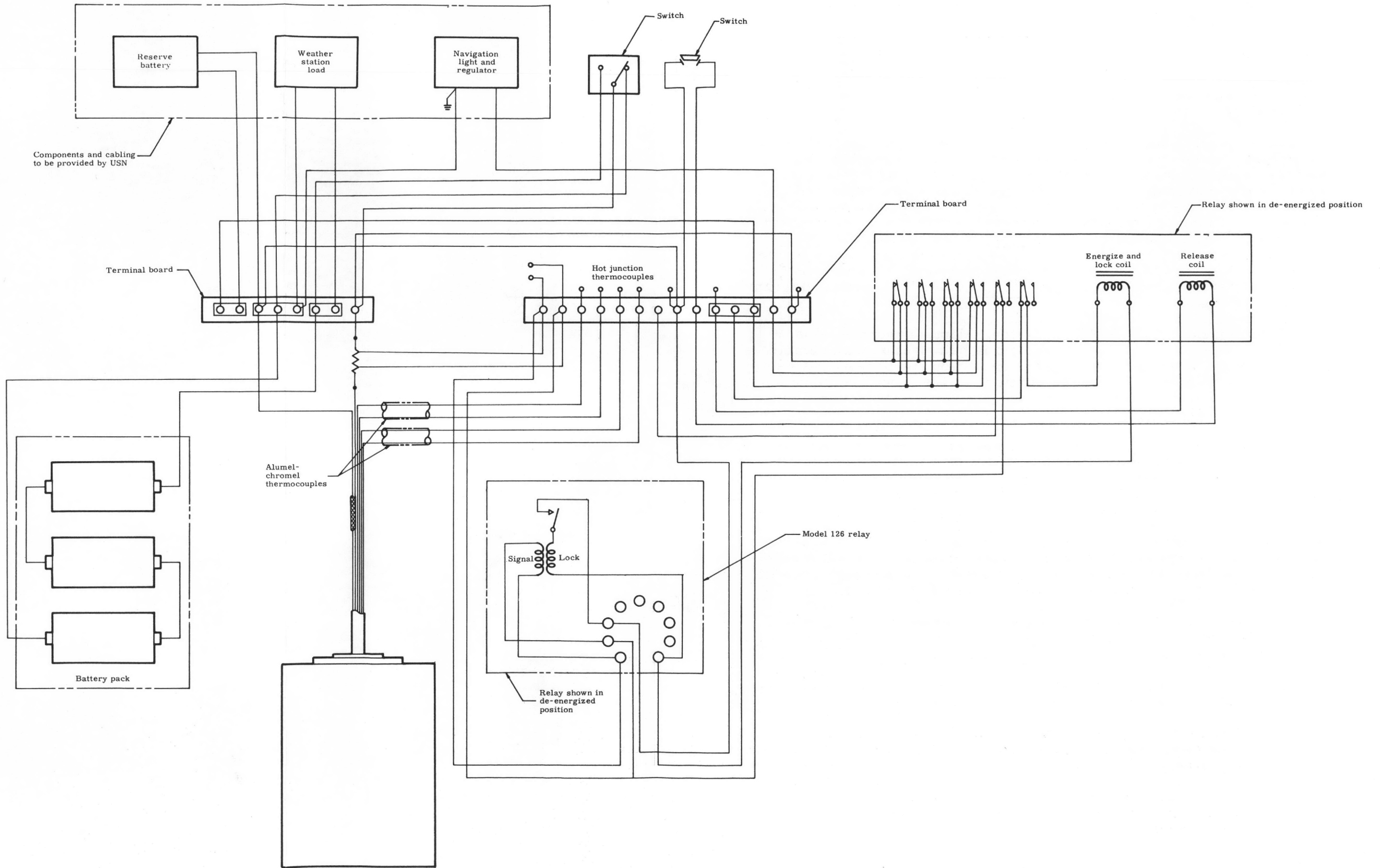
Fig. 9. SNAP 7D System--Schematic Diagram of Electrical System
