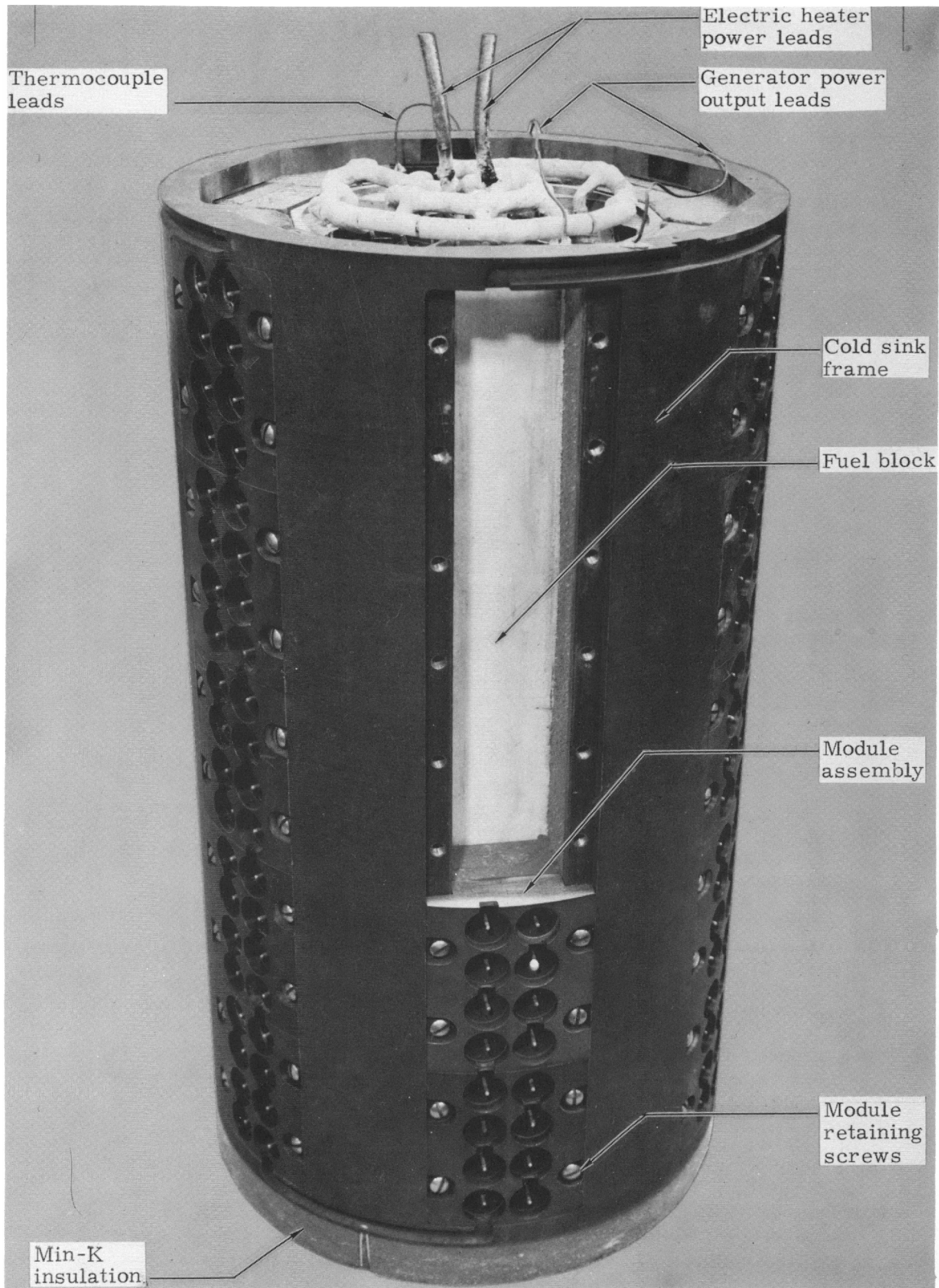
Fig. 5. SNAP 7B-D Thermoelectric Modules Assembled in Electrically Heated Generator (60-watt)
