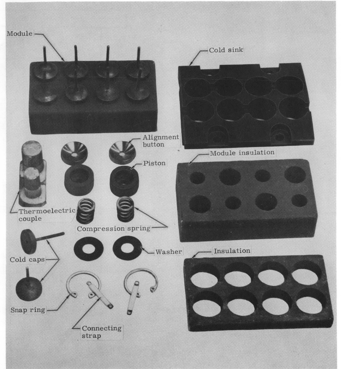
Fig. 4. SNAP 7B-D Thermoelectric Module Components
