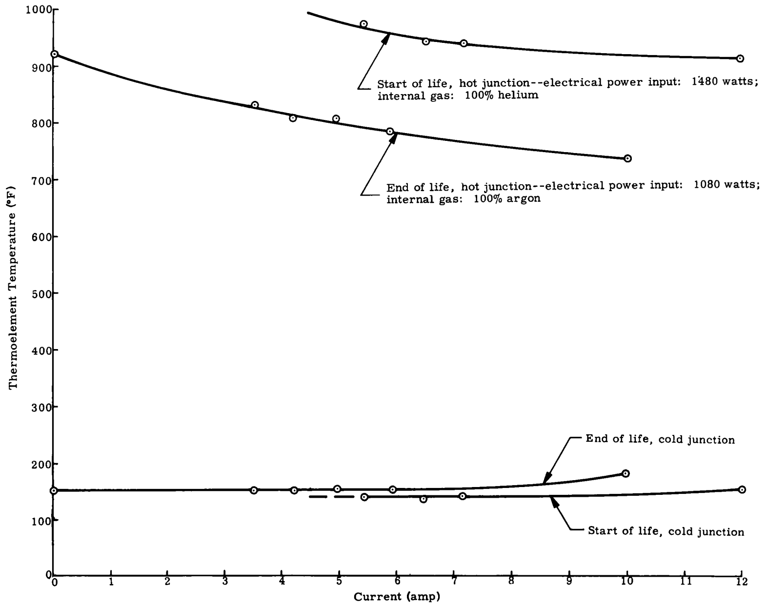
Fig. 7. SNAP 7D 60-Watt Generator--Thermolement Temperature Versus Current
