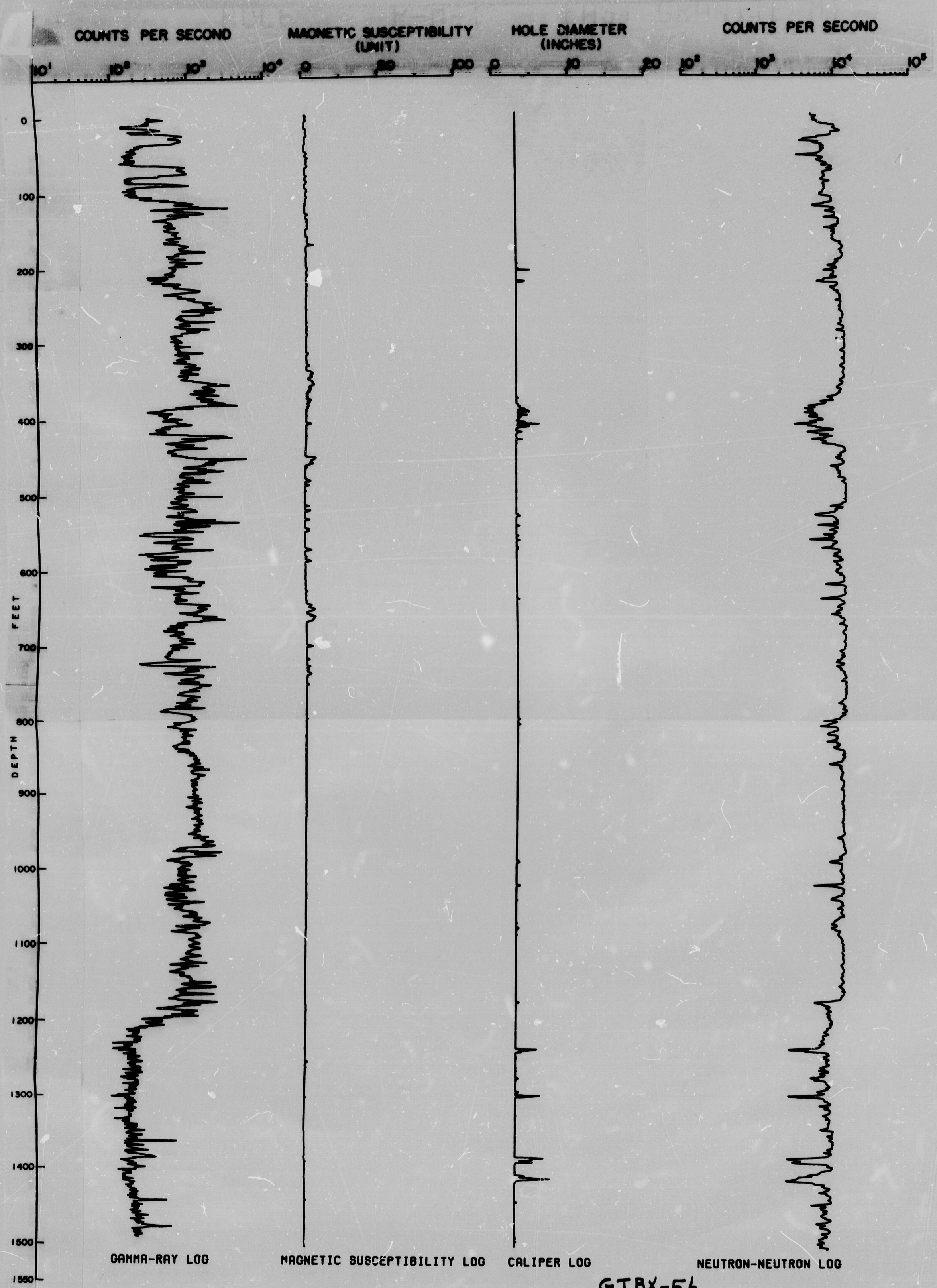
Plate 9. BFEC caliper, gross gamma, neutron-neutron, and magnetic susceptibility logs.
