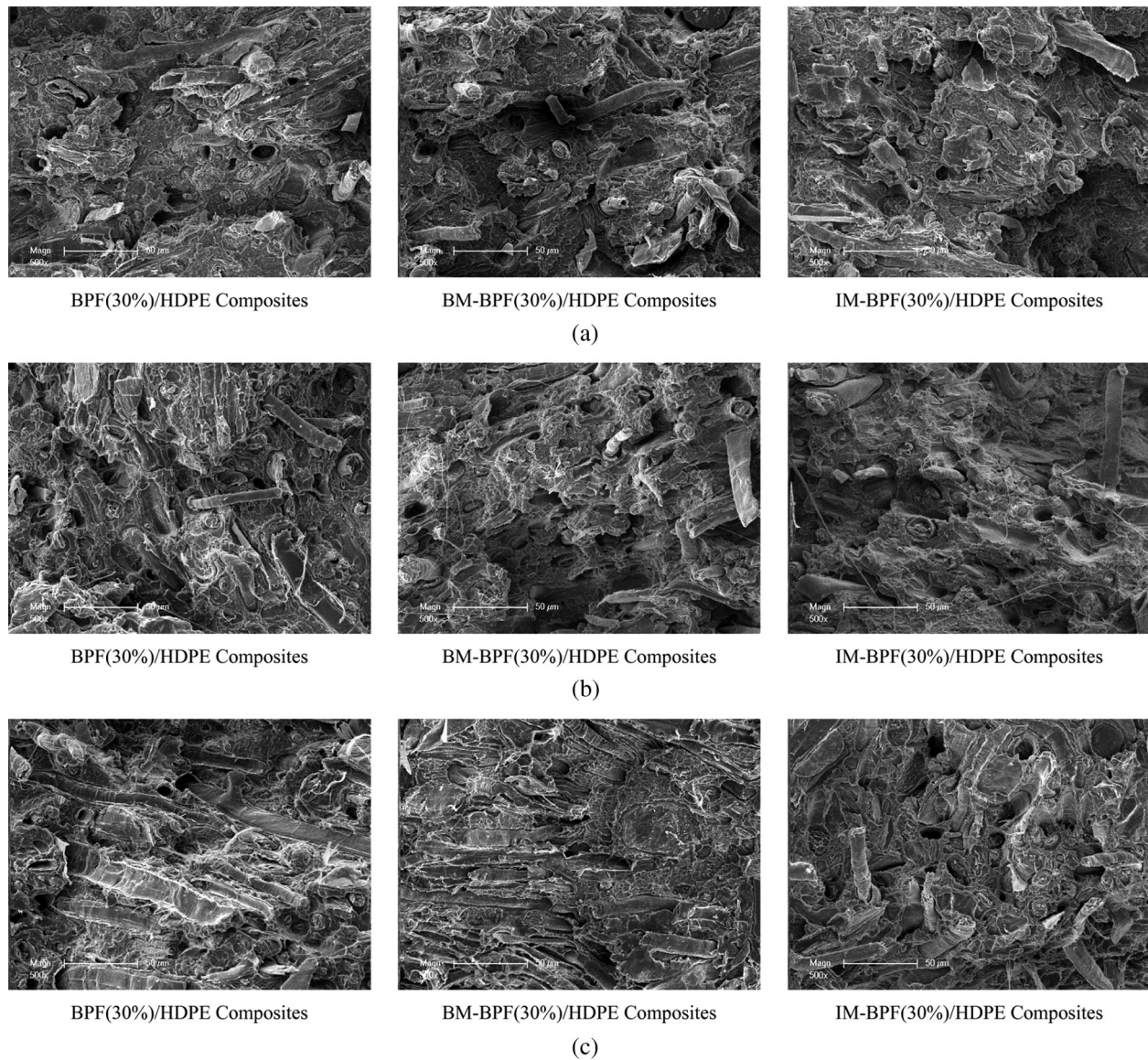
Figure 6: ESEM micrographs ( \times 500 ) of BPF/HDPE, BM-BPF/HDPE IM-BPF/HDPE composites fracture surfaces subjected to manufacturing process, for (a) EMP; (b) IMP; (c) HPMP
