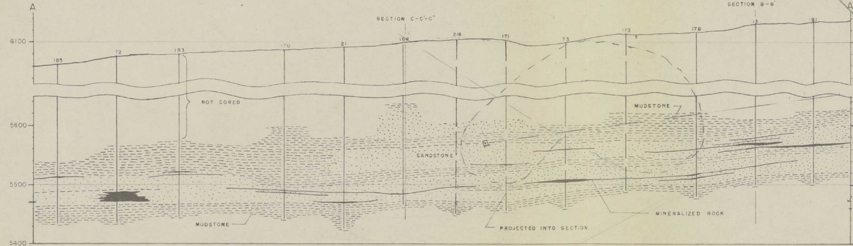
GEOLOGIC SECTION A-A'
