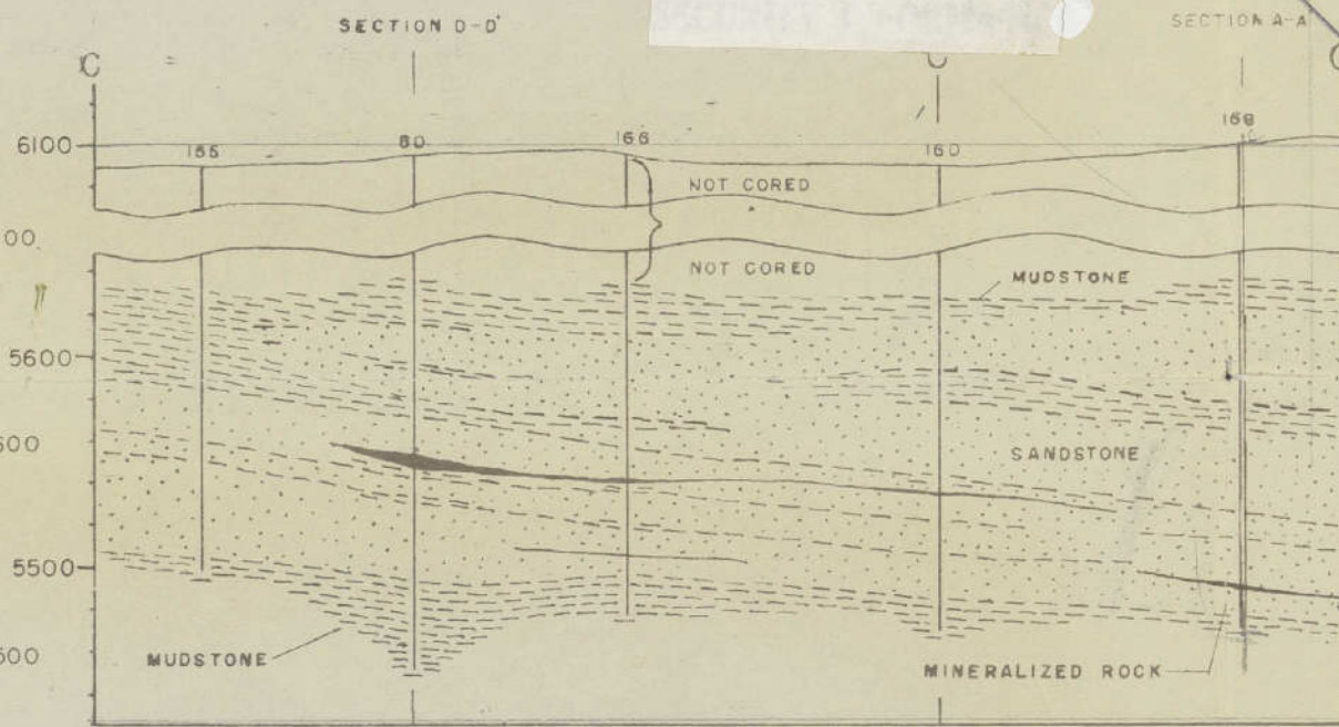
GEOLOGIC SECTION C-C'-C''
