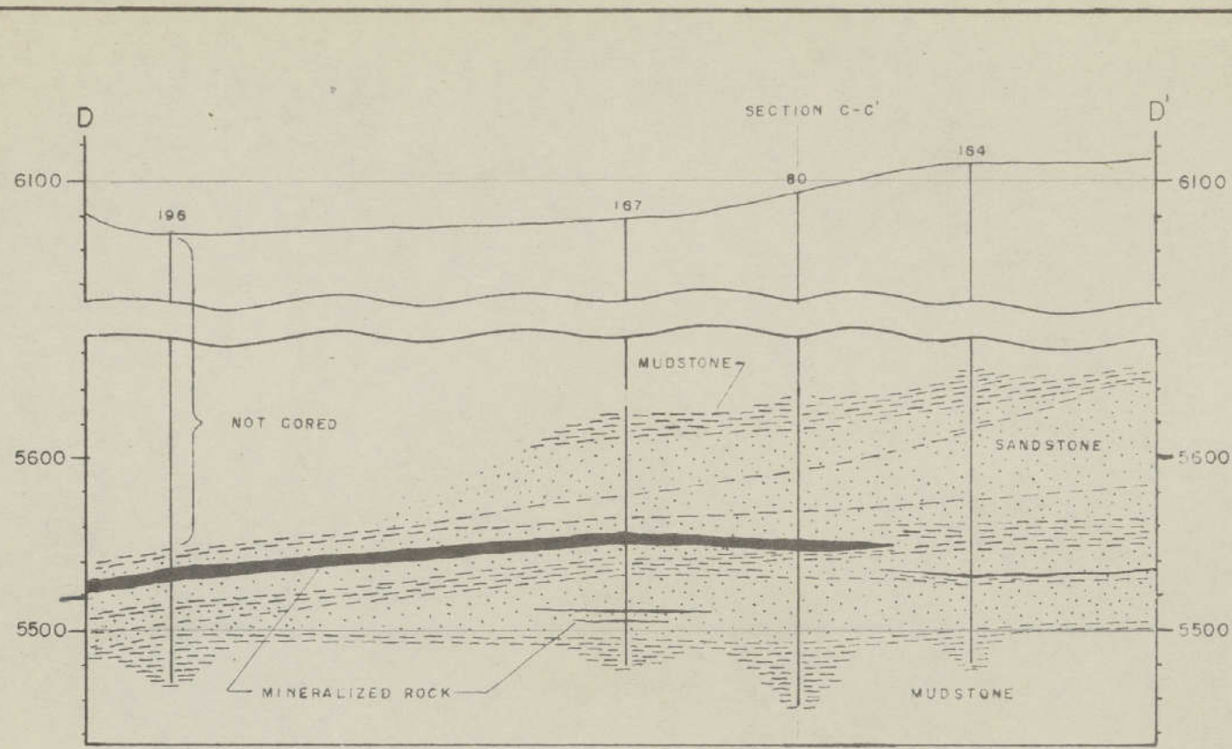
GEOLOGIC SECTION D-D'
