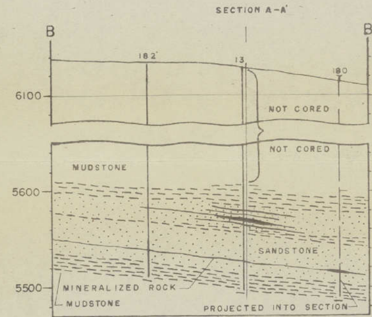
GEOLOGIC SECTION B-B'
