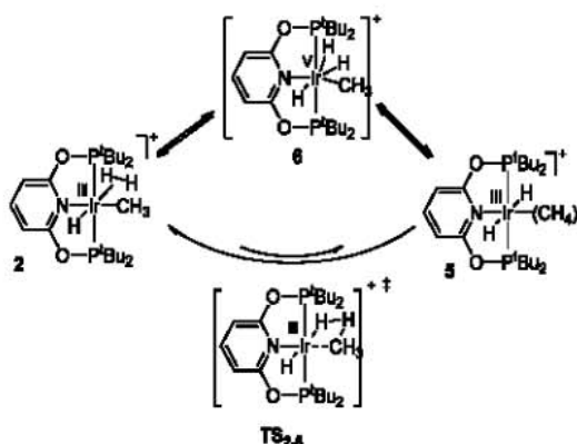
Scheme 4. Two Potential Mechanisms for Interconversion of 2 and 5
