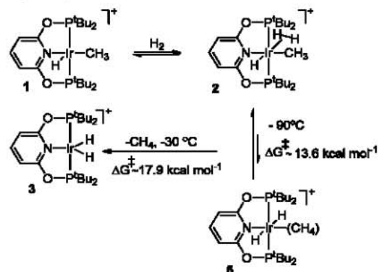
Scheme 3. Hydrogenolysis of Complex 1 and Formation of -CH 4 Complex 5
