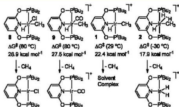
Figure 4. Experimentally determined \Delta G values for CH 4 elimination from Ir complexes 1 , 2 , 8 , and 9 .
