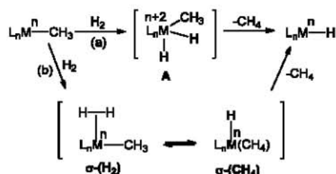
Scheme 1. Two Possible Pathways for Hydrogenolysis of a M–CH 3 Bond
