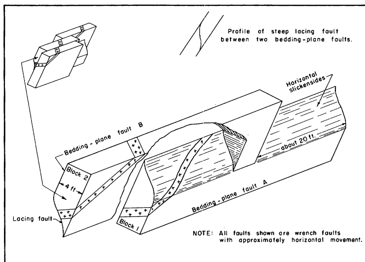
FIGURE 3. - Schematic Diagram of a Steep Lacing Fault, Red Devil Mine.
