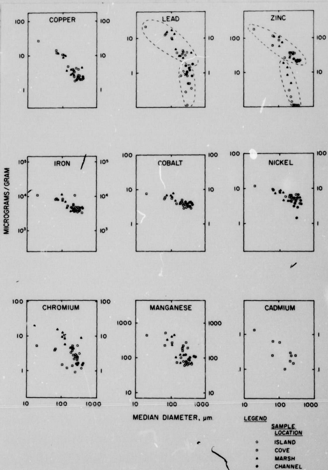
Figure 11. Acid-leached trace metal concentrations versus median particle diameter in Miller Sands soil and sediment samples collected in summer 1975
