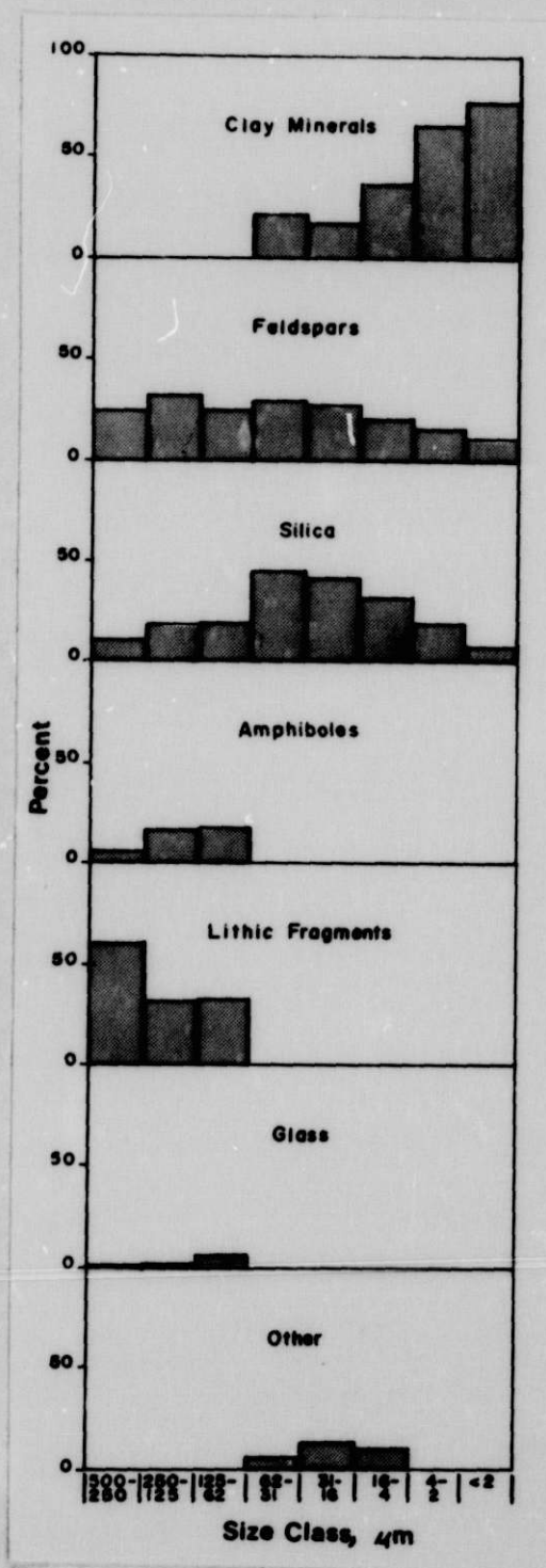
Figure 7. Distribution of major mineral groups among size classes of lower Columbia River sediment at St. Helens station. Percentages in each size class sum to 100%. (Summarized from Glenn, 1973.)
