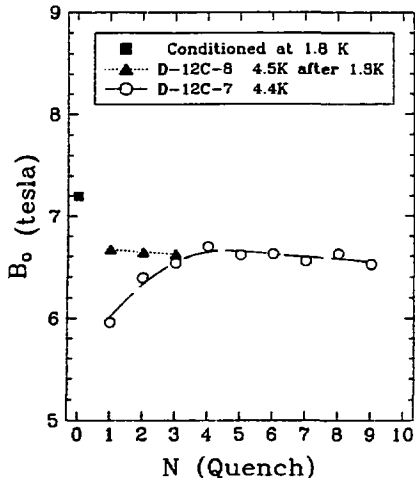
Fig. 2. Training at 4.4 K vs. 1.8 K Conditioning
