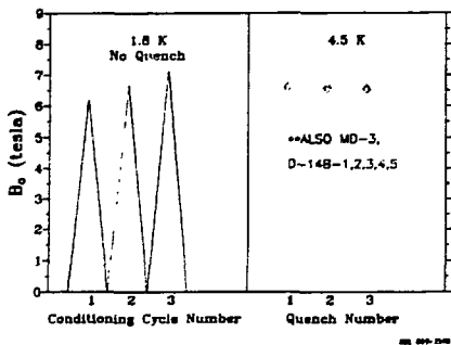
Fig. 1. Low Temperature Conditioning of D-12C-8
