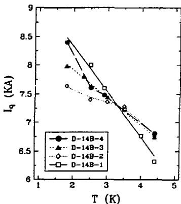
Fig. 5. Reduced Temperature Conditioning Training LBL-SSC Dipole Models
