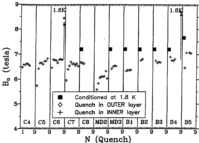
Fig. 4. Training of 12 LBL-SSC Dipole Models
