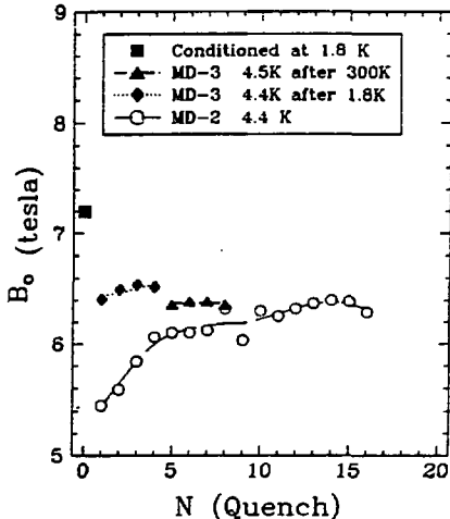
Fig. 3. Training of MD-2; Conditioning of MD-3
