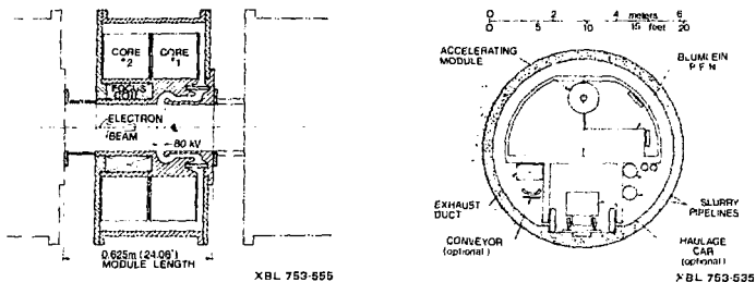
Fig. 3. Schematic of one of the 64 accelerator modules. Fig. 4. Section at accelerator unit.
