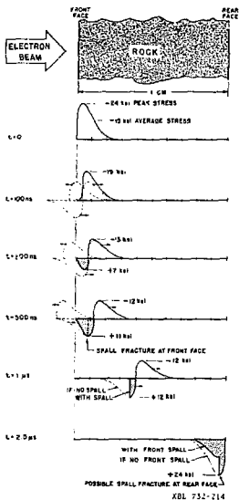
Fig. 1. Stress wave propagation. Fig. 2. Example one-shot spall.
