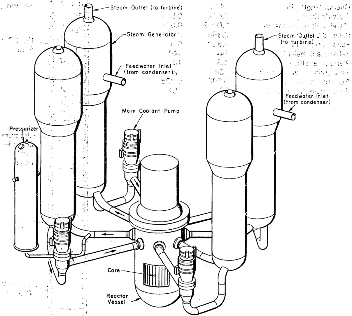
FIGURE 3-3 Schematic of Reactor Coolant System for PWR
