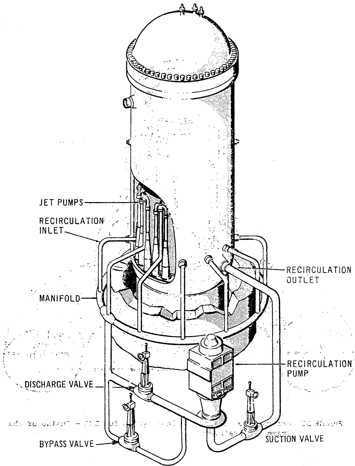
FIGURE 3-4 Schematic of BWR Reactor Coolant System
