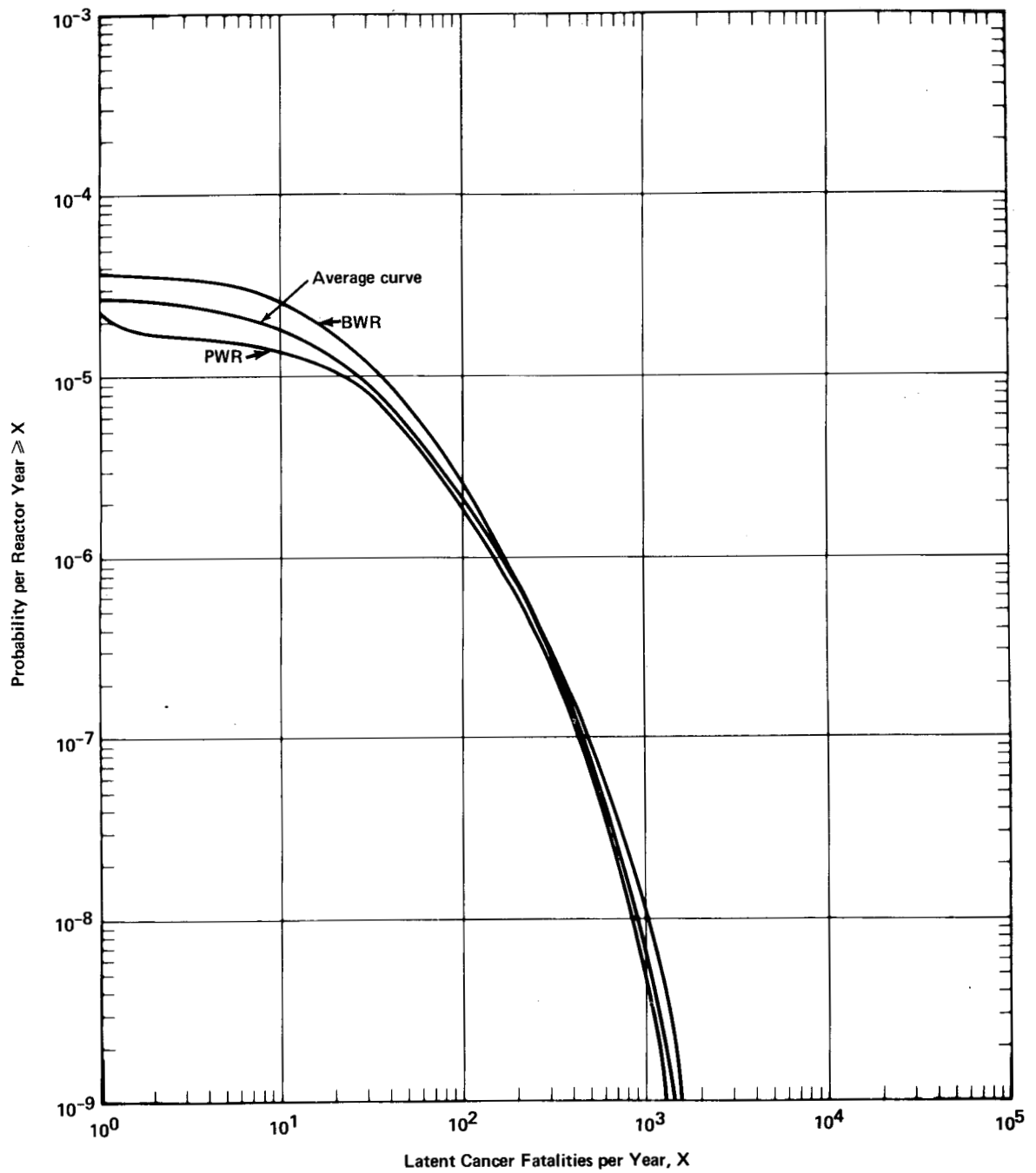
FIGURE 5-5 Probability Distribution for Latent Cancer Fatality Incidence per Reactor Year
