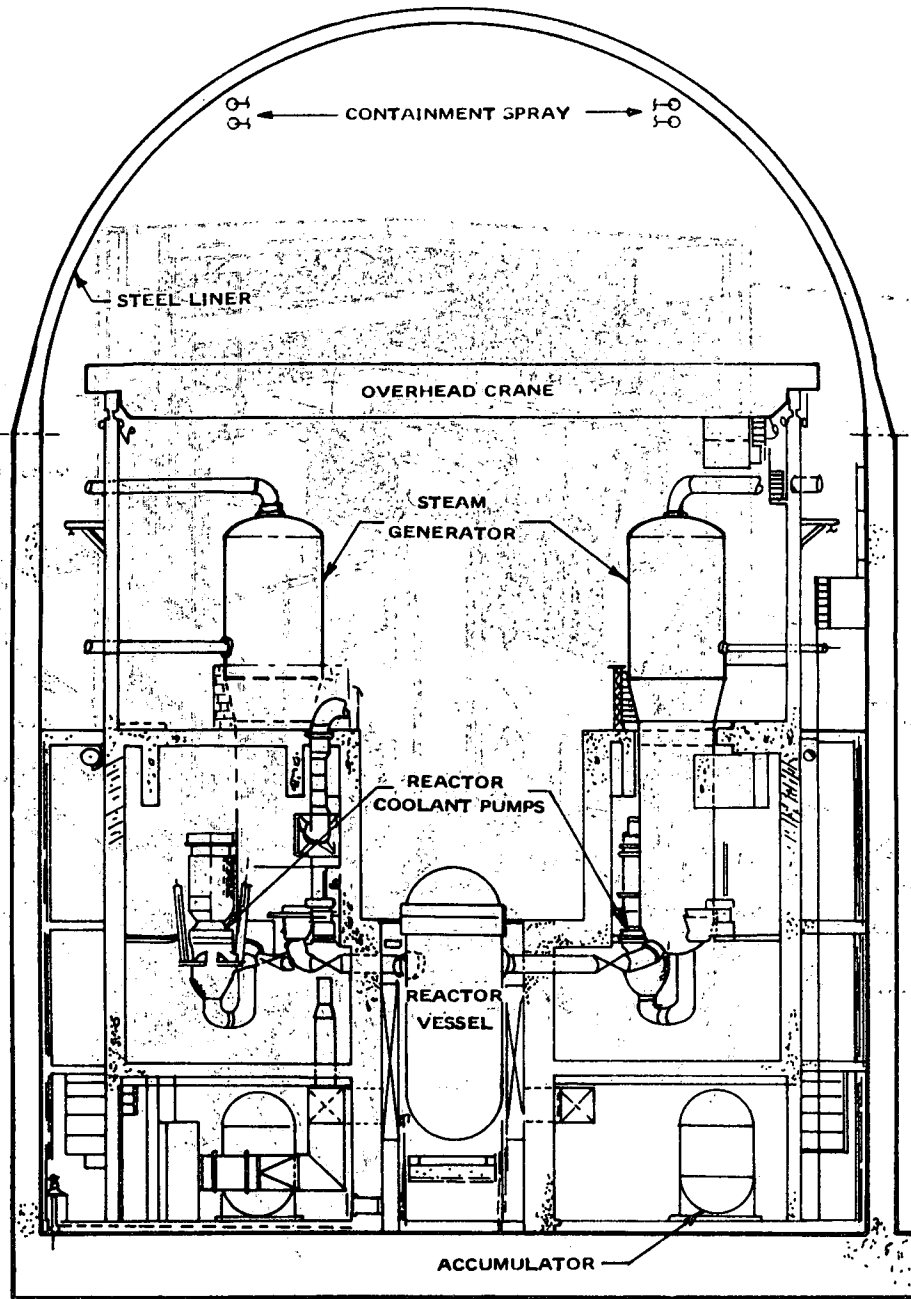
FIGURE 3-7 Typical PWR Containment
