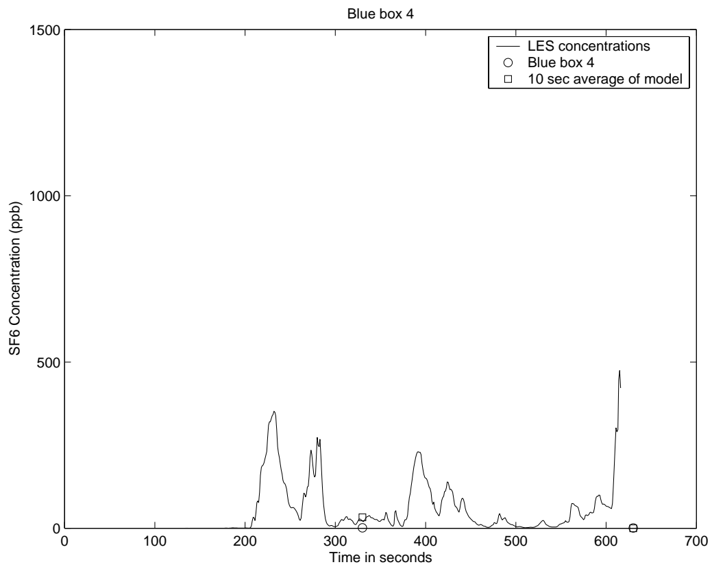
Figure 25. Concentrations of SF6 (ppb): simulated vs measured - BlueBox station 4.
