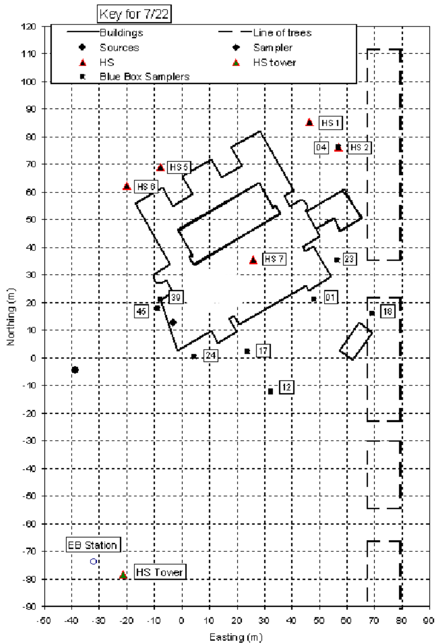
Figure 4. Instrument deployment map for July 22. EB represents the energy-budget station, and HS refers to locations of high-speed sonics. The fast response SF 6 (Miran) sampler is located at the southwest corner of the building as designated by the diamond.
