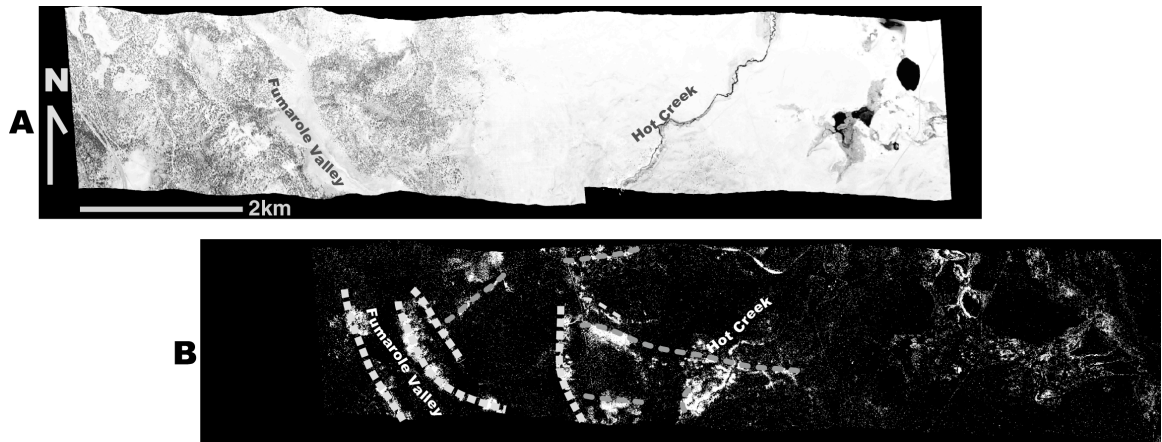
Figure 2A. Geo-corrected, panchromatic HyMap image of the Fumarole Valley/Hot Creek region. B. The kaolinite distribution image. Pixels that match the reference kaolinite spectrum to 95% are shown in white. Previously mapped faults are shown by the square-box lines, while hyperspectrally determined structures are shown with the rounded-box lines.
