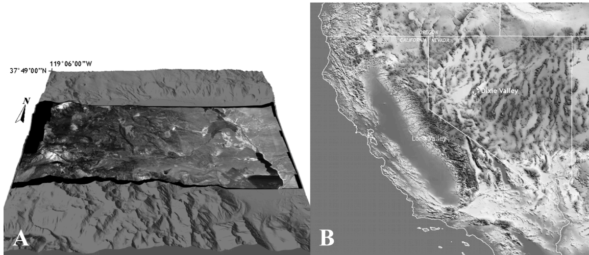
Figure 1A. Spatial extent of 1999 HyMap acquisition over Long Valley Caldera draped over a USGS 10-meter DEM. B. Geographical location of Long Valley Caldera, CA and Dixie Meadows, NV.
