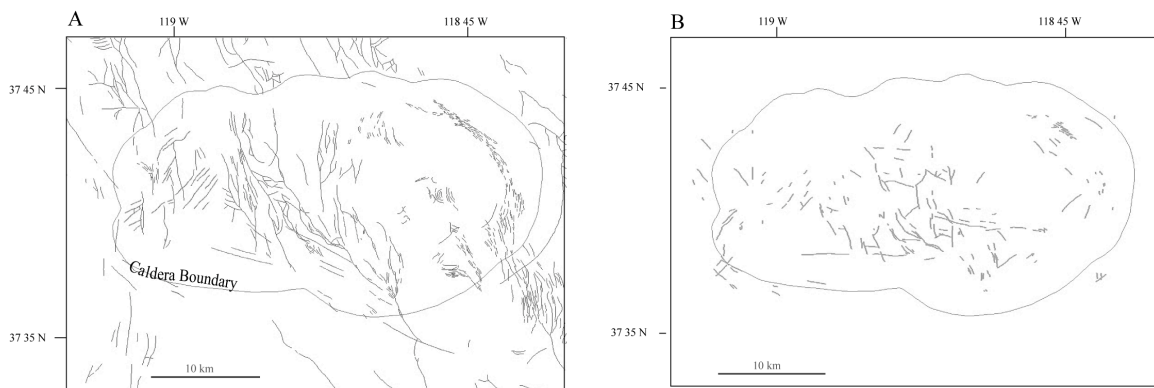
Figure 3A. Map of previously known fault distribution in Long Valley Caldera. B. Hyperspectrally detected faults and fractures.
