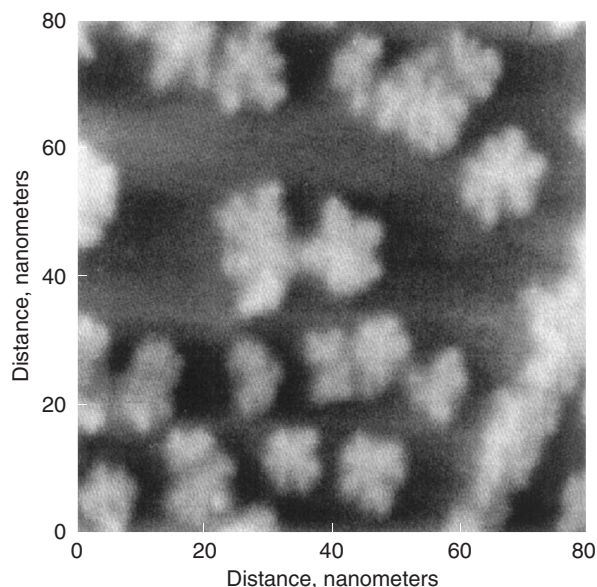
An image of silicon nanocrystals using an atomic force microscope. The nanocrystals, produced using gas-phase vaporization, range from 1 to 4 nanometers. Note how the nanoclusters gather at the step edges of the graphite substrate or assemble into snowflake-like superclusters.
