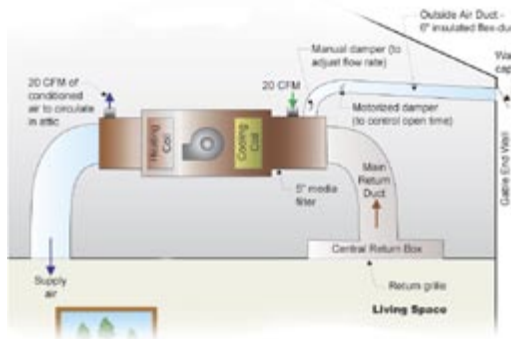
FIGURE 15: Outside Vents
