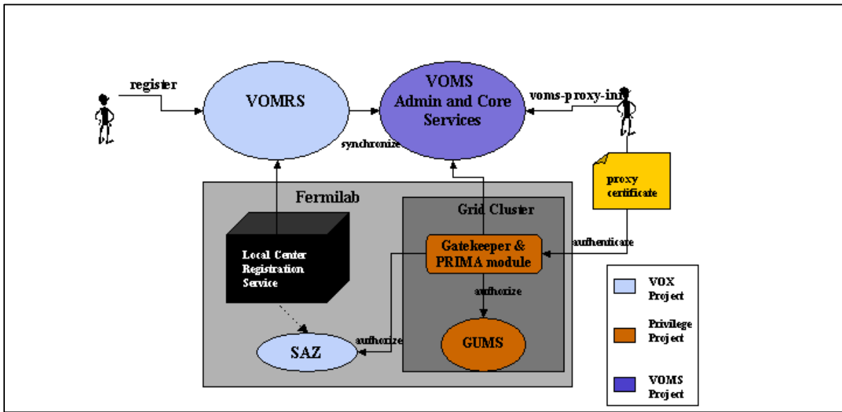
Figure 1: VO Management Infrastructure at Fermilab
