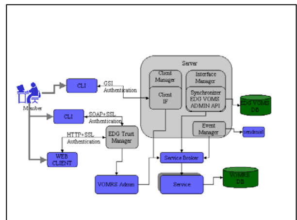
Figure 4: VOMRS Architecture
