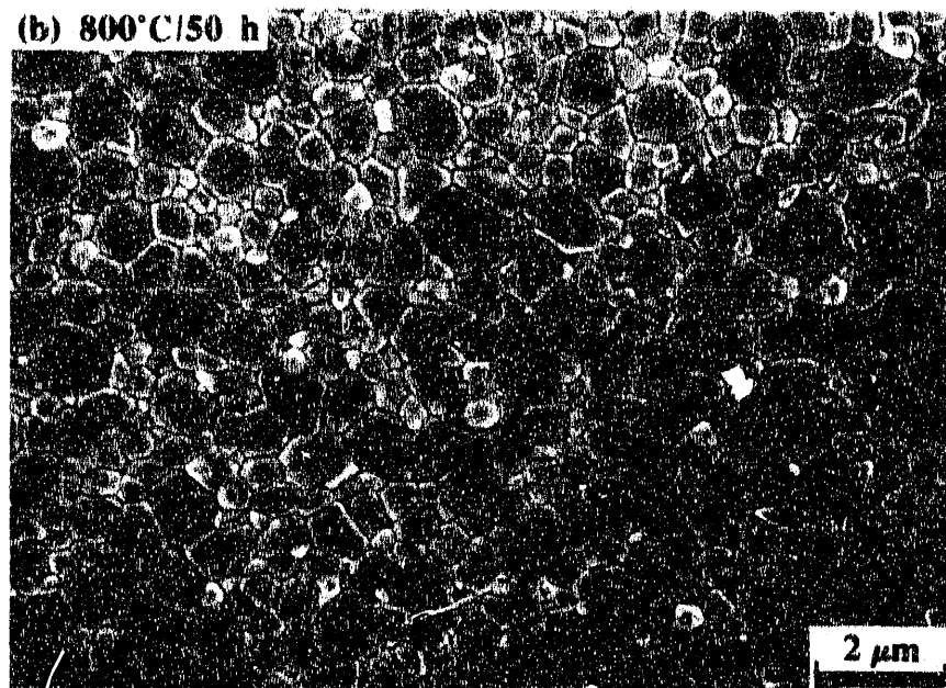
Figure 4.23 Scanning electron micrographs of polished and thermally etched surfaces of 250 ppm MgO-doped \text{Al}_2\text{O}_3 compacts formed by isostatic pressing. Sintering was conducted at a constant heating rate of 5^\circ\text{C}/\text{min} . to 1450^\circ\text{C} : (a) conventional sample; (b) 800^\circ\text{C}/50\text{ h} homogenized; (c) 800^\circ\text{C}/100\text{ h} homogenized; (d) 800^\circ\text{C}/200\text{ h} homogenized.
