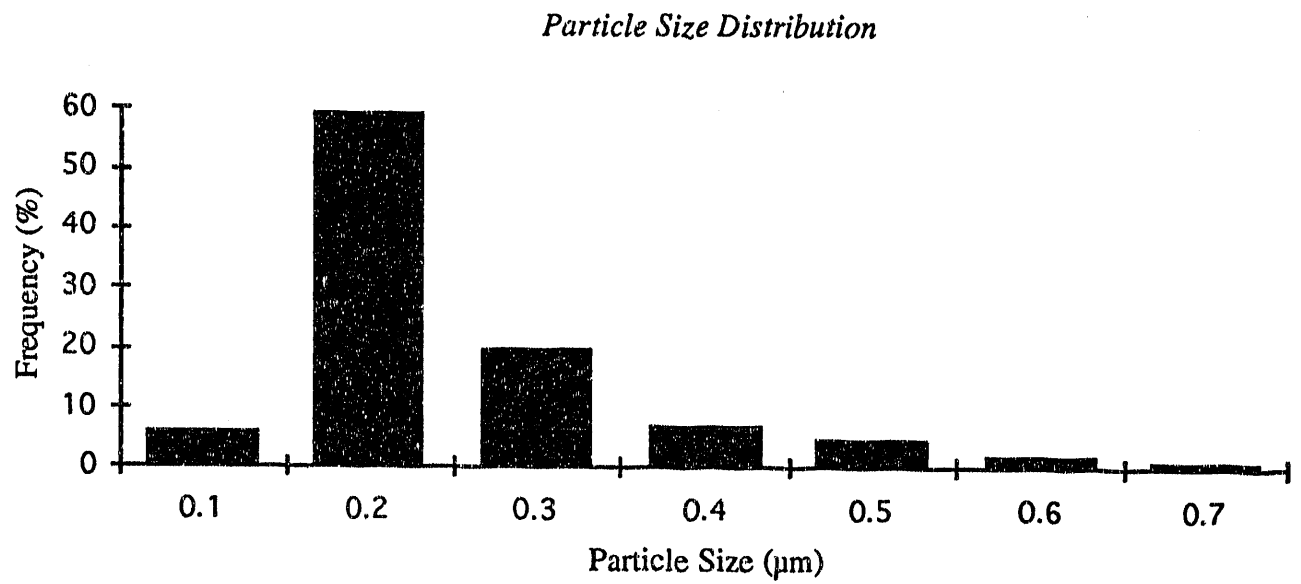
Figure 3.2 Particle size distribution of \text{Al}_2\text{O}_3 powder measured by the centrifugal sedimentation method. The size distribution is very narrow.
