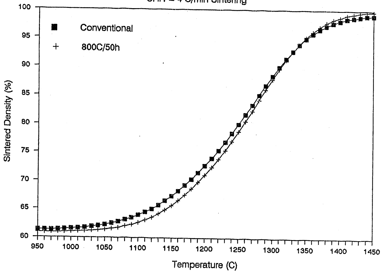
Figure 4.6 Evolution of instantaneous density as a function of temperature for the conventional and the homogenized samples sintered in air at a constant heating rate of 4°C/min. to 1450°C without soaking.
