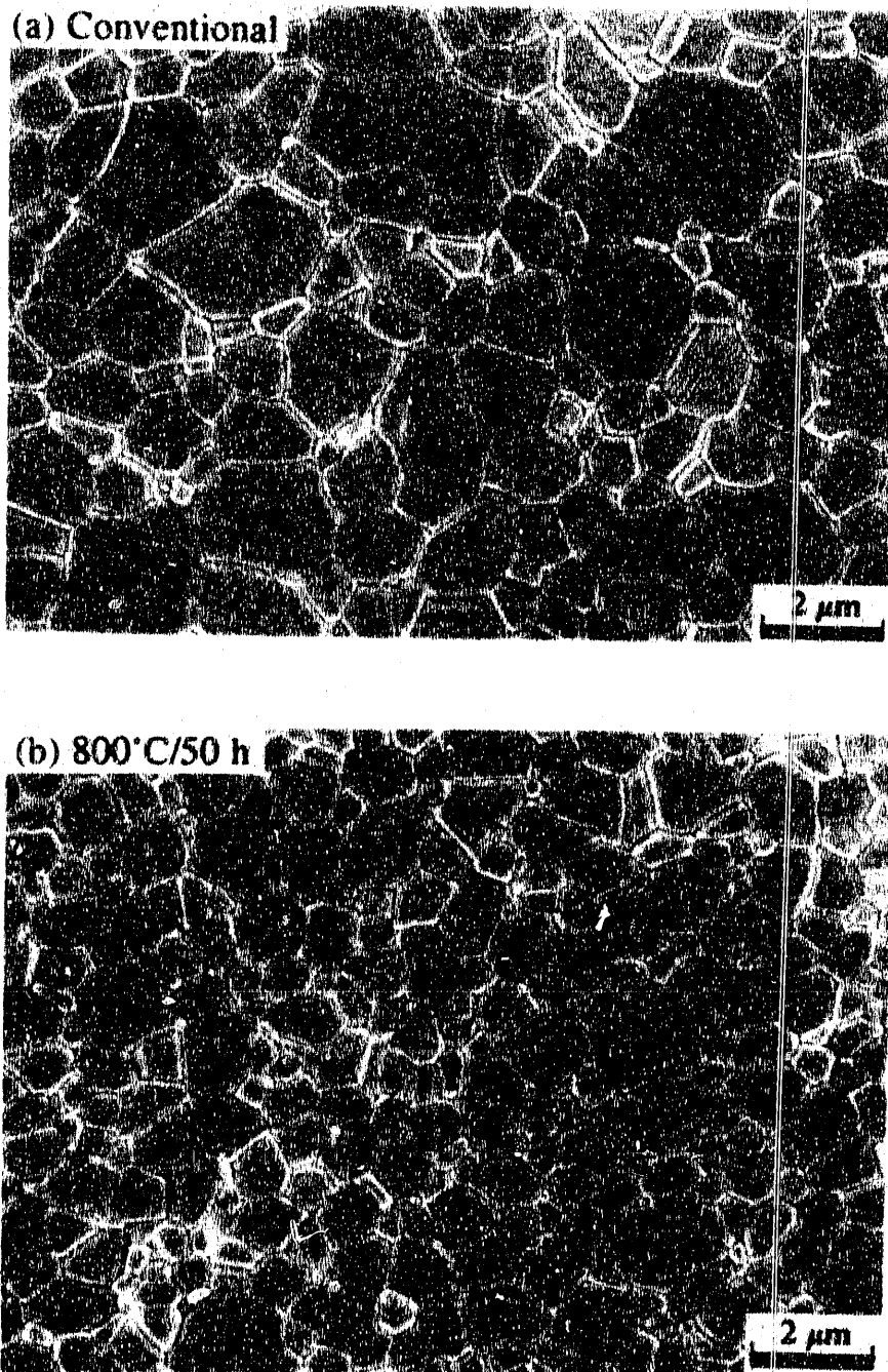
Figure 4.25 Scanning electron micrographs of polished and thermally etched surfaces of 250 ppm MgO-doped \text{Al}_2\text{O}_3 compacts formed by isostatic pressing ( \approx 1380 MPa). Sintering was conducted at a constant heating rate of 4^\circ\text{C}/\text{min.} to 1450^\circ\text{C} in air: (a) conventional sample, mean grain size is 1.44 \mu\text{m} ; (b) 800^\circ\text{C}/50 h homogenized, mean grain size is 1.07 \mu\text{m} .
