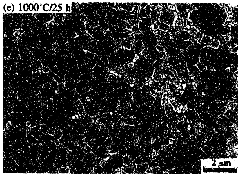
Figure 4.21 (Continued) Scanning electron micrographs of polished and thermally etched surfaces of Al 2 O 3 compacts sintered at a constant heating rate of 4°C/min. to 1400°C: (a) conventional sample; (b) 800°C/25 h homogenized; (c) 800°C/50 h homogenized; (d) 900°C/25 h homogenized; (e) 1000°C/25 h homogenized.
