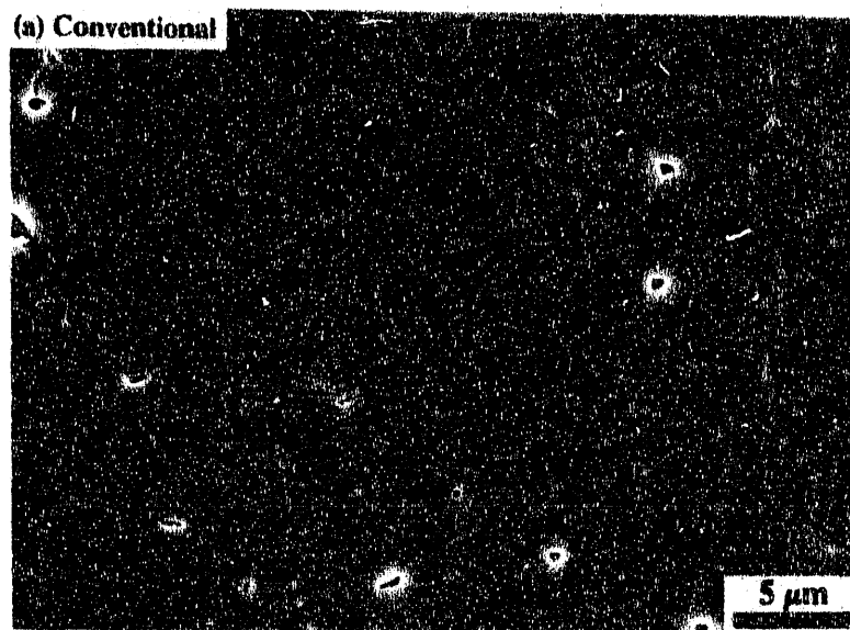
Figure 4.24 Scanning electron micrographs of polished and thermally etched surfaces of MgO-doped Al 2 O 3 samples fast fired in vacuum at a heating rate of 340°C/min. to 1750°C and held for 5 minutes: (a) conventional sample; (b) 800°C/50 h homogenized; (c) 800°C/100 h homogenized.
