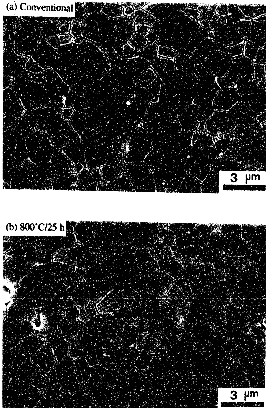
Figure 4.22 Scanning electron micrographs of polished and thermally etched surfaces of \text{Al}_2\text{O}_3 compacts sintered at a constant heating rate of 4^\circ\text{C}/\text{min.} to 1450^\circ\text{C} : (a) conventional sample; (b) 800^\circ\text{C}/25 h homogenized; (c) 800^\circ\text{C}/50 h homogenized; (d) 900^\circ\text{C}/25 h homogenized; (e) 1000^\circ\text{C}/25 h homogenized.
