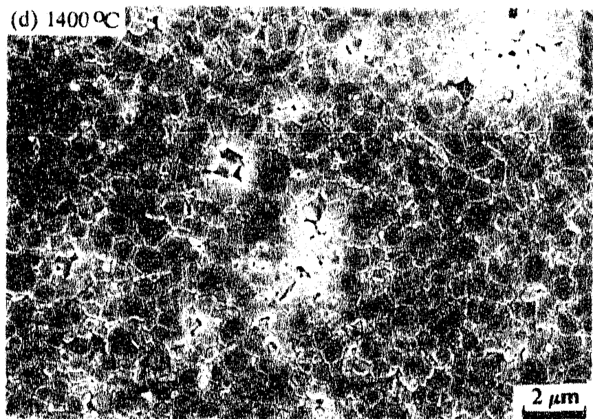
Figure 4.11 (Continued) Scanning electron micrographs of the conventional samples sintered at a constant heating rate of 4°C/min. to different final temperatures: (a) 1260°C; (b) 1300°C; (c) 1350°C; (d) 1400°C.
