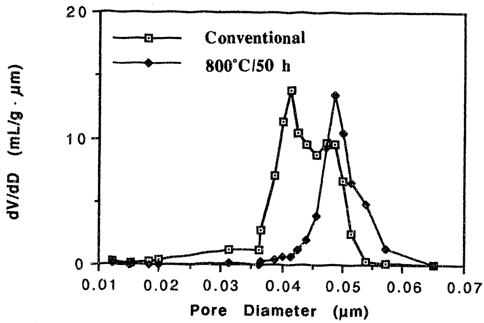
Figure 4.2 Plot of pore size distribution as a function of pore diameter obtained from mercury porosimetry for the conventional and 800°C/50 h homogenized samples (before sintering).
