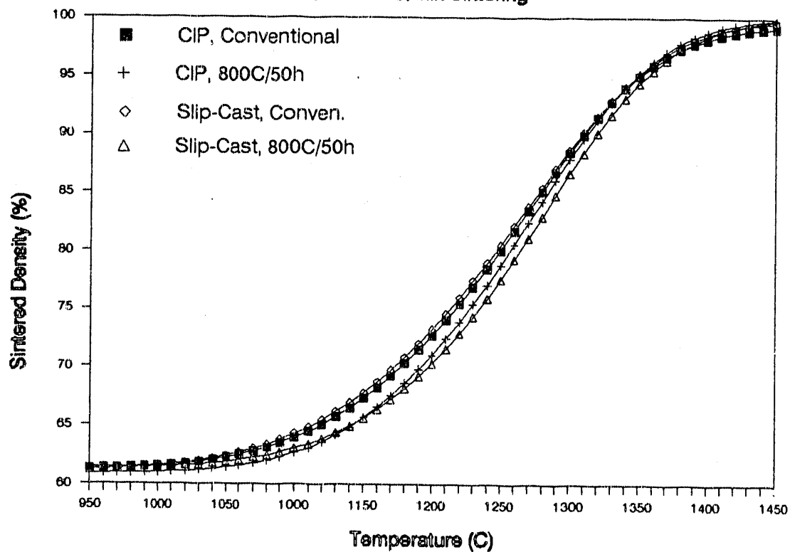
Figure 4.17 Sintered density is plotted as a function of temperature for powder compacts formed by isostatic pressing and slip casting techniques. Sintering was conducted for the conventional and the homogenized samples at a constant heating rate of 4°C/min. to 1450°C in air.
