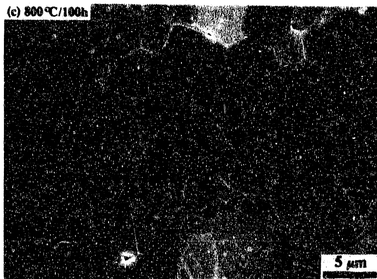
Figure 4.24 (Continued) Scanning electron micrographs of polished and thermally etched surfaces of MgO-doped \text{Al}_2\text{O}_3 samples fast fired in vacuum at a heating rate of 340^\circ\text{C}/\text{min.} to 1750^\circ\text{C} and held for 5 minutes: (a) conventional sample; (b) 800^\circ\text{C}/50 h homogenized; (c) 800^\circ\text{C}/100 h homogenized.
