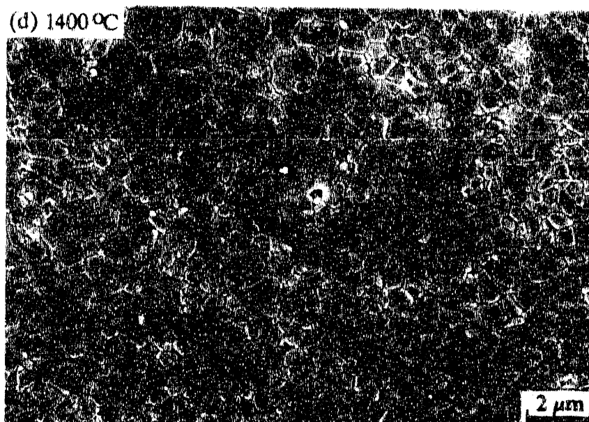
Figure 4.12 (Continued) Scanning electron micrographs of the 800°C/50 h homogenized samples sintered at a constant heating rate of 4°C/min. to different final temperatures: (c) 1350°C; (d) 1400°C.
