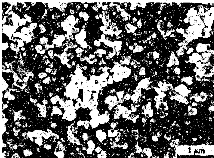
Figure 3.1 The morphology of Al 2 O 3 powder after 29 hours sedimentation to remove agglomerates. The average particle size is 0.17 μm.
