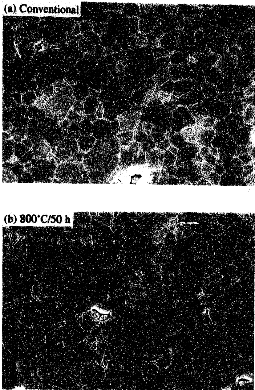
Figure 4.5 Another set of samples sintered at the same conditions as in Figure 4.4 with lower magnification showing nonuniform grain size distribution in the conventional sample.
