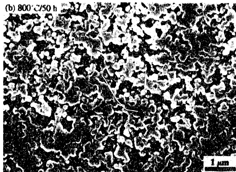
Figure 4.9 Scanning electron micrographs of polished and thermally etched surfaces of \text{Al}_2\text{O}_3 samples sintered at a heating rate of 4^\circ\text{C}/\text{min.} to 1200^\circ\text{C} : (a) conventional sample, \rho_f = 0.76 T.D.; (b) 800^\circ\text{C}/50 h homogenized sample, \rho_f = 0.73 T.D.
