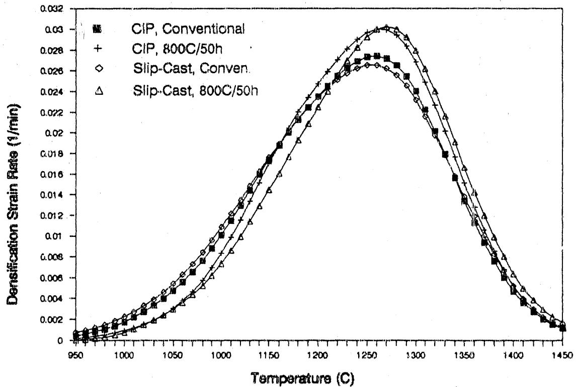
Figure 4.18 Densification rate is plotted as a function of temperature for powder compacts formed by isostatic pressing and slip casting techniques. Sintering was conducted for the conventional and the homogenized samples at a constant heating rate of 4°C/min. to 1450°C in air.
