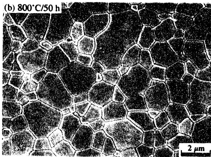
Figure 4.16 Scanning electron micrographs of polished and thermally etched surfaces of slip cast \text{Al}_2\text{O}_3 samples sintered at a heating rate of 4^\circ\text{C}/\text{min.} to 1450^\circ\text{C} without soaking: (a) conventional sample, mean grain size is 2.16\ \mu\text{m} ; (b) 800^\circ\text{C}/50\ \text{h} homogenized, mean grain size is 1.84\ \mu\text{m} .
