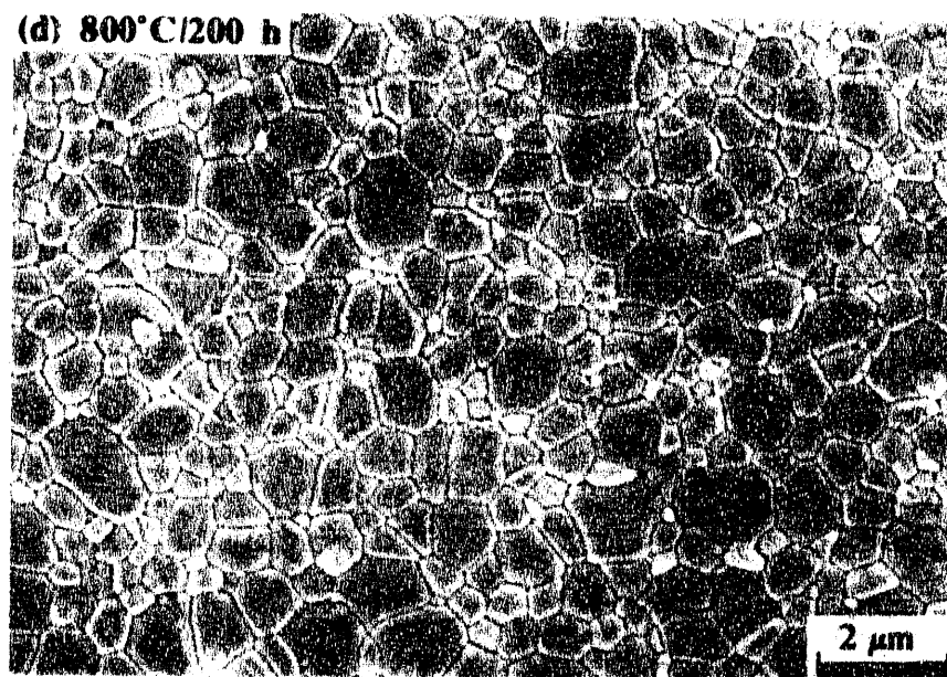
Figure 4.23 (Continued) Scanning electron micrographs of polished and thermally etched surfaces of 250 ppm MgO-doped \text{Al}_2\text{O}_3 compacts formed by isostatic pressing. Sintering was conducted at a constant heating rate of 5^\circ\text{C}/\text{min.} to 1450^\circ\text{C.} : (c) 800^\circ\text{C}/100 h homogenized; (d) 800^\circ\text{C}/200 h homogenized.
