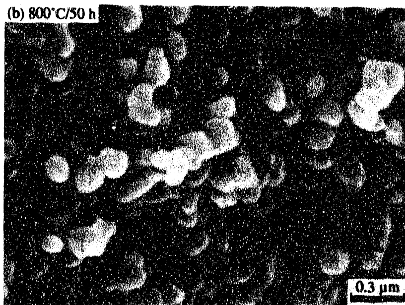
Figure 4.1 Scanning electron micrographs of fracture surfaces of unsintered \text{Al}_2\text{O}_3 compacts. Powder compacts were formed by isostatic pressing at 1380 MPa: (a) as-formed; (b) after 800°C/50 h heat treatment.
