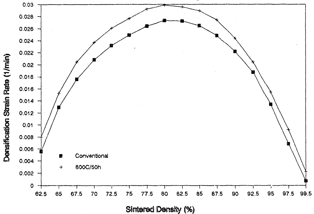
Figure 4.8 Plot of densification strain rate as a function of sintered density for the conventional and the homogenized sintered in air at a constant heating rate of 4°C/min. to 1450°C without soaking.
