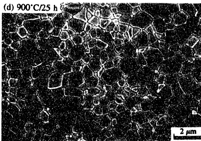
Figure 4.21 (Continued) Scanning electron micrographs of polished and thermally etched surfaces of \text{Al}_2\text{O}_3 compacts sintered at a constant heating rate of 4^\circ\text{C}/\text{min.} to 1400^\circ\text{C} : (a) conventional sample; (b) 800^\circ\text{C}/25\text{ h} homogenized; (c) 800^\circ\text{C}/50\text{ h} homogenized; (d) 900^\circ\text{C}/25\text{ h} homogenized; (e) 1000^\circ\text{C}/25\text{ h} homogenized.
