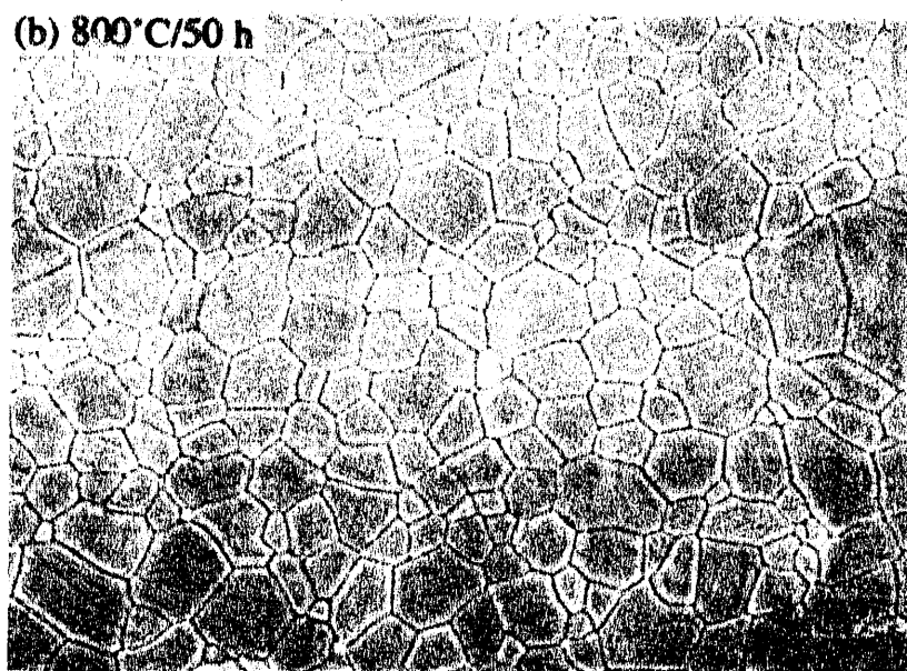
Figure 4.4 Scanning electron micrographs of polished and thermally etched surfaces of \text{Al}_2\text{O}_3 samples sintered at a heating rate of 4^\circ\text{C}/\text{min.} to 1450^\circ\text{C} : (a) conventional sample, mean grain size is 1.52\ \mu\text{m} ; (b) 800^\circ\text{C}/50\ \text{h} homogenized, mean grain size is 1.18\ \mu\text{m} .
