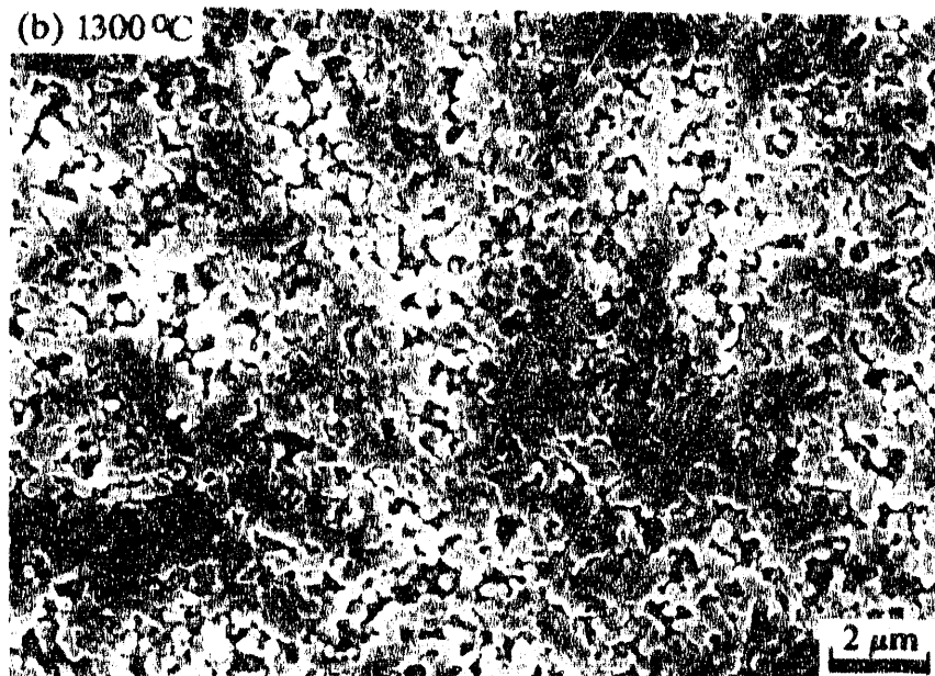
Figure 4.12 Scanning electron micrographs of the 800°C/50 h homogenized samples sintered at a constant heating rate of 4°C/min. to different final temperatures: (a) 1260°C; (b) 1300°C; (c) 1350°C; (d) 1400°C.
