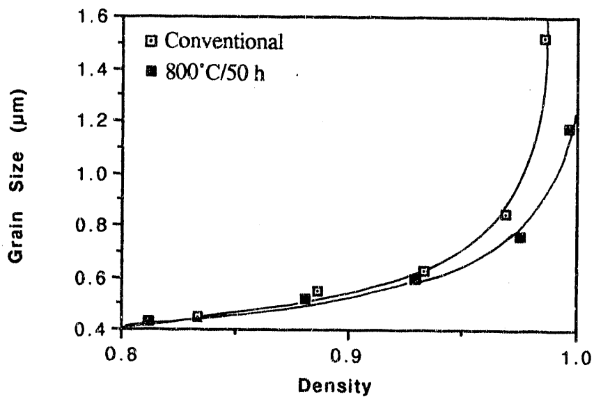
Figure 4.15 Plot of average grain size as a function of sintered density for the conventional and the 800°C/50 h homogenized samples. The average grain size is significantly reduced at higher densities through the use of the homogenization heat treatment.
