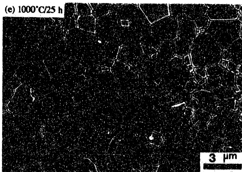
Figure 4.22 (Continued) Scanning electron micrographs of polished and thermally etched surfaces of \text{Al}_2\text{O}_3 compacts sintered at a constant heating rate of 4^\circ\text{C}/\text{min.} to 1450^\circ\text{C} : (a) conventional sample; (b) 800^\circ\text{C}/25 h homogenized; (c) 800^\circ\text{C}/50 h homogenized; (d) 900^\circ\text{C}/25 h homogenized; (e) 1000^\circ\text{C}/25 h homogenized.
