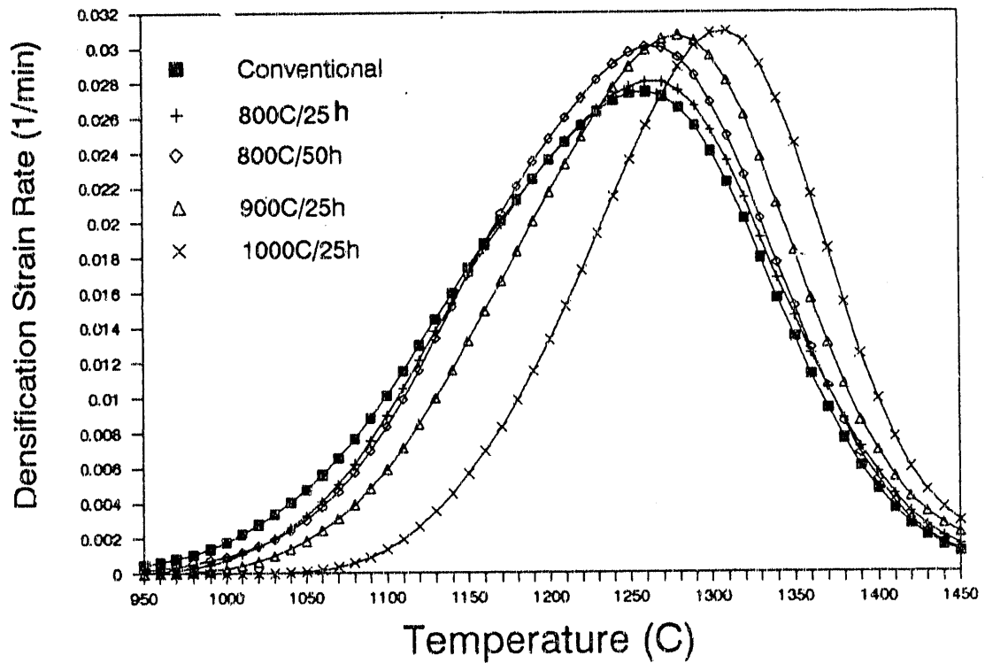
Figure 4.20 Densification rate is plotted as a function of temperature for powder compacts formed by isostatic pressing ( \approx 1380 MPa). Sintering was conducted at a constant heating rate of 4^\circ\text{C}/\text{min} . to 1450^\circ\text{C} in air.
