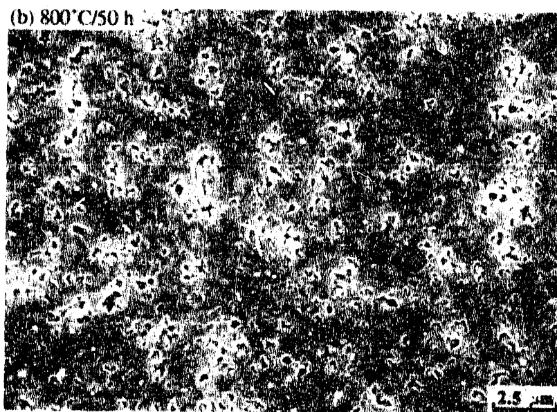
Figure 4.10 Scanning electron micrographs of polished and thermally etched surfaces of \text{Al}_2\text{O}_3 samples sintered at a heating rate of 4^\circ\text{C}/\text{min} . to 1350^\circ\text{C} . Dense regions are surrounded by large pores in (a) conventional sample; pore size is small and uniformly distributed in (b) 800^\circ\text{C}/50\text{ h} homogenized sample.
