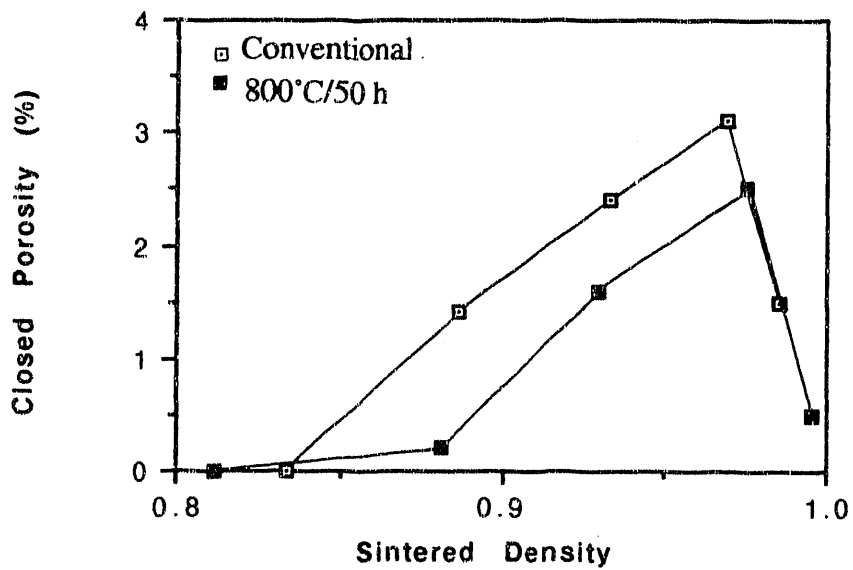
Figure 4.14 Variation of closed porosity as a function of sintered density for the conventional and the homogenized samples sintered at a constant heating rate of 4°C/min.
