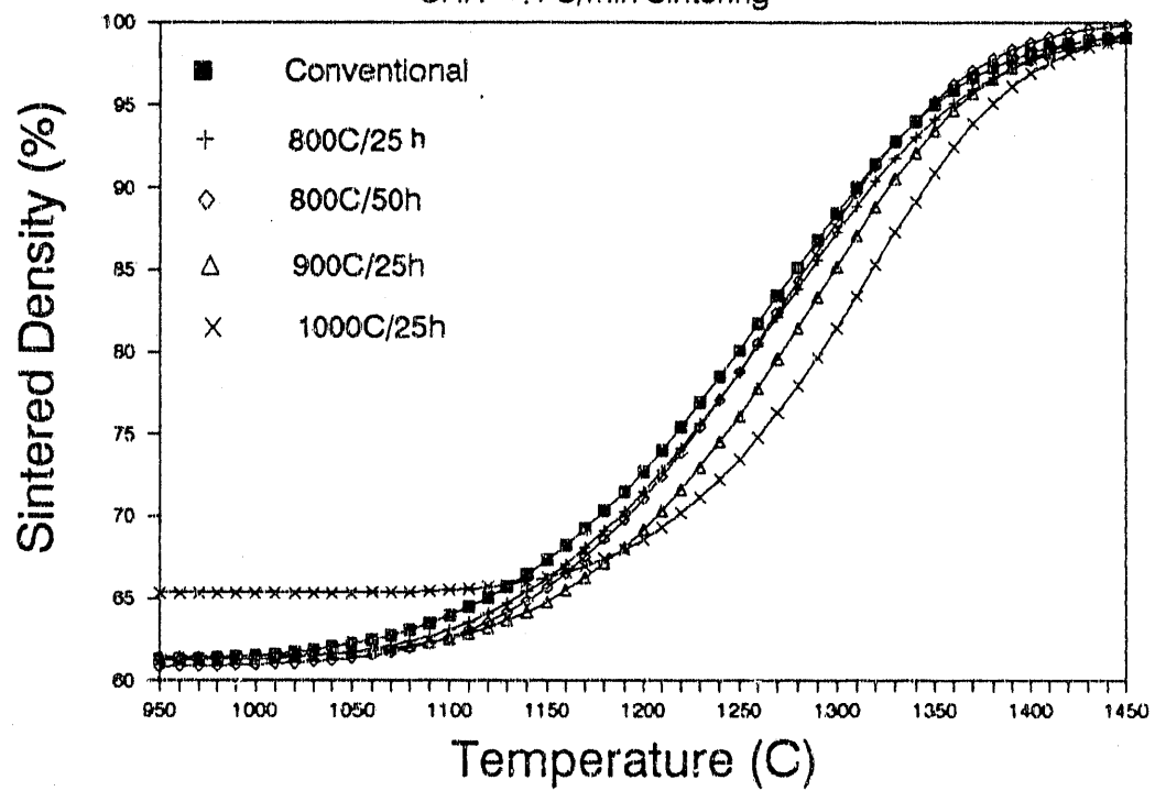
Figure 4.19 Sintered density is plotted as a function of temperature for powder compacts formed by isostatic pressing. Sintering was conducted at a constant heating rate of 4°C/min. to 1450°C in air.
