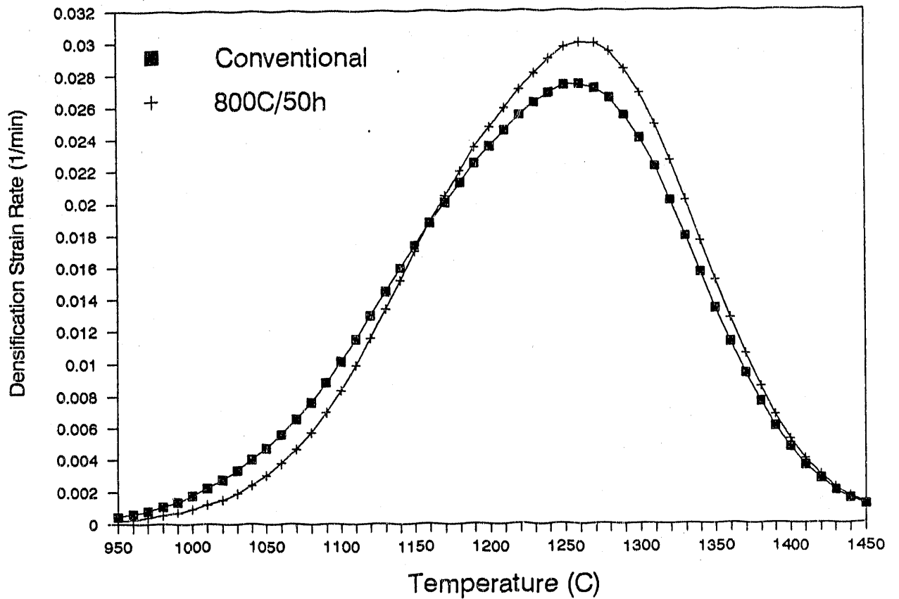
Figure 4.7 Plot of densification strain rate versus temperature for the conventional and the homogenized samples sintered in air at a constant heating rate of 4°C/min. to 1450°C without soaking.
