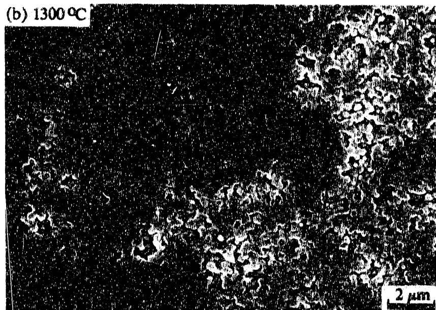
Figure 4.11 Scanning electron micrographs of the conventional samples sintered at a constant heating rate of 4°C/min. to different final temperatures: (a) 1260°C; (b) 1300°C; (c) 1350°C; (d) 1400°C.
