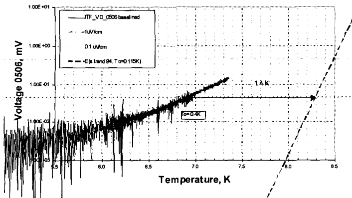
Fig.3. Voltage-temperature characteristic of the TF Insert and comparison with the Bochvar strand transition (46 kA, 12 T)
