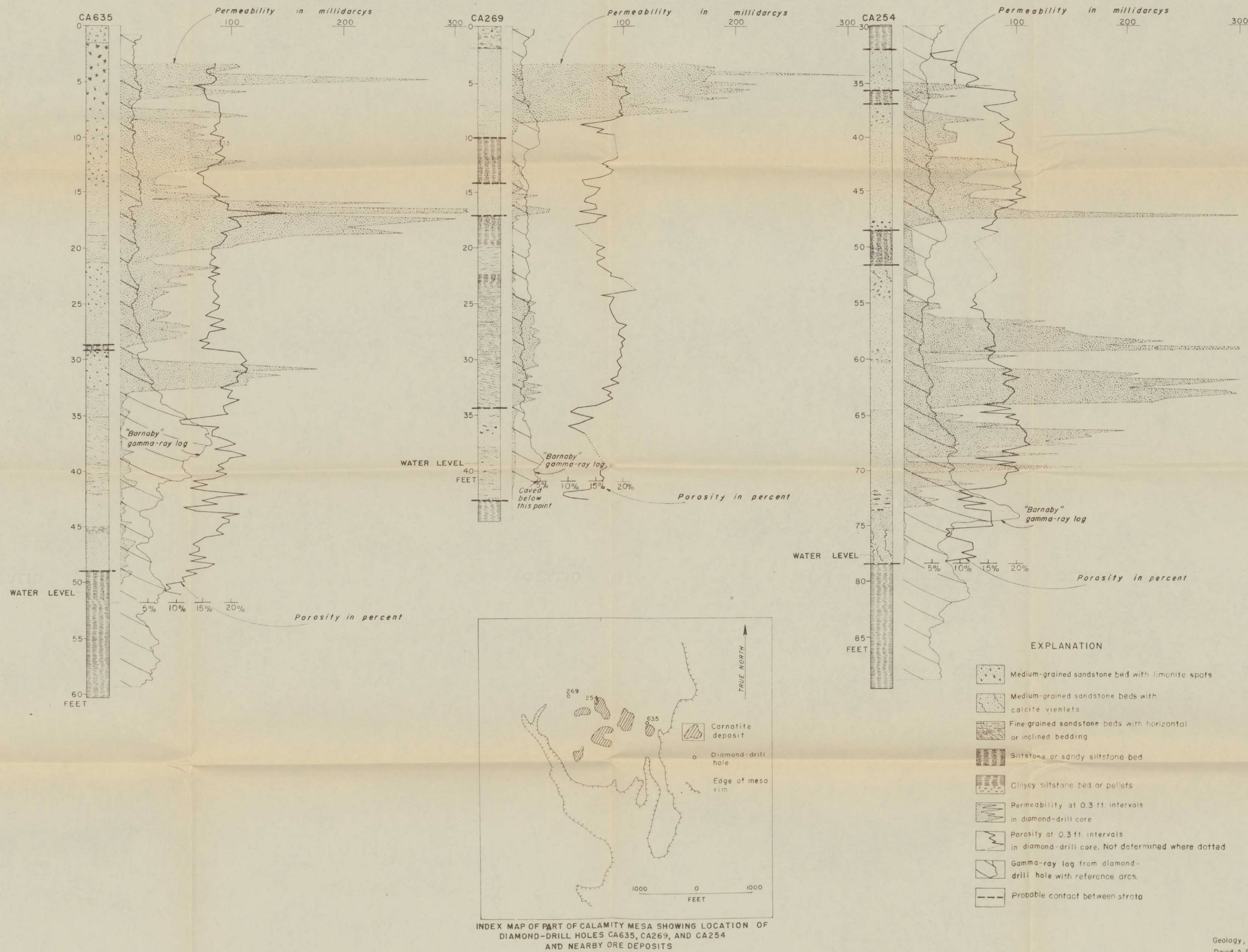
FIGURE 1. GEOLOGIC LOGS OF CORE FROM THREE DIAMOND-DRILL HOLES ON CALAMITY MESA, MESA COUNTY, COLO., SHOWING CORRELATION BETWEEN THE GAMMA-RAY LOGS AND THE PERMEABILITY AND POROSITY OF THE ORE-BEARING SANDSTONE OF THE SALT WASH SANDSTONE MEMBER OF THE MORRISON FORMATION.
