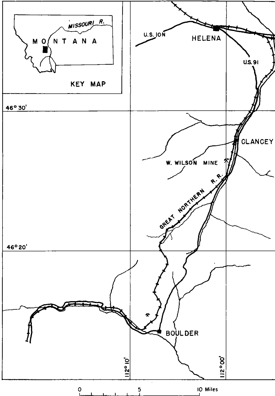
Figure 1. - Index map showing location of W. Wilson Mine near Clancey, Jefferson County, Montana.
