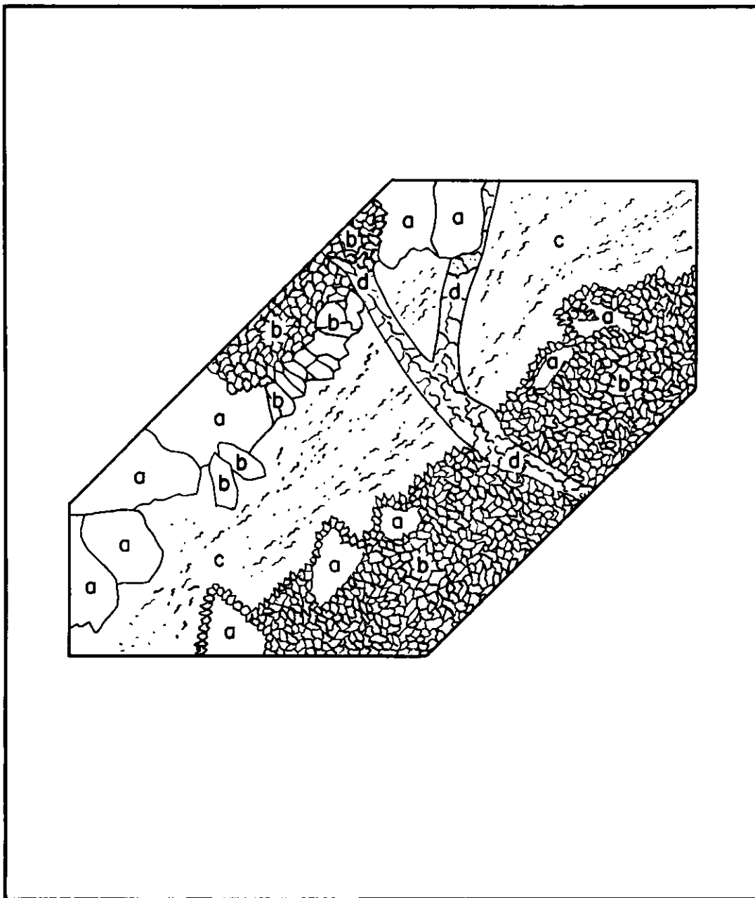
FIGURE 4-SKETCH SHOWING QUARTZ-CHALCEDONY RELATIONS IN VEINS.
